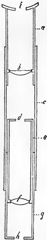
FIG. 3.—Janssen's compound microscope (1590).
