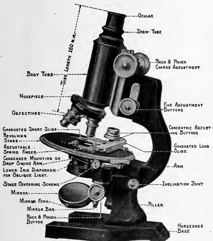
FIG. 6.—A modern compound microscope.
