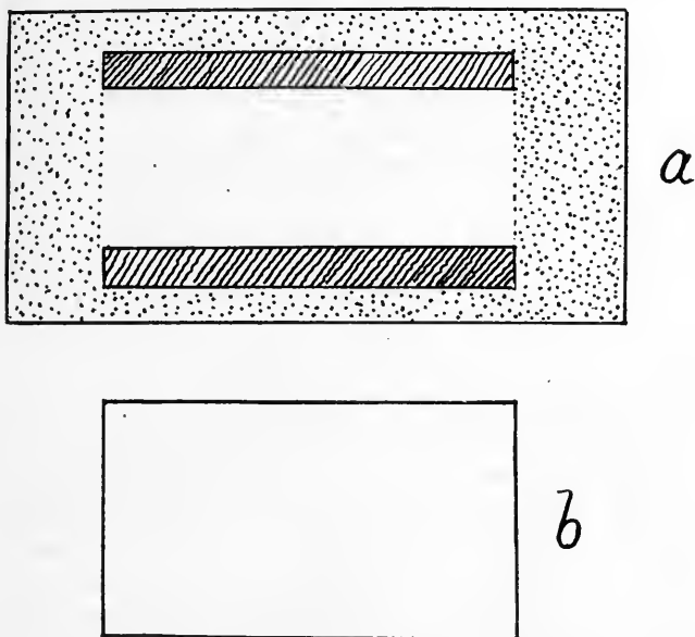
FIG. 35.—Special counting chamber for making quantitative microanalyses of foods, spices and drugs. The two glass slips upon the extra size slide are exactly 0.2 mm. thick and the area bounded on two sides by the two slips is 10 sq. cm. (1,000 sq. mm.). 0.2 cc. suspensions of this material to be examined is spread in this area and covered with the rectangular cover glass (b). Full size. (Made by the Bausch and Lomb Optical Company.)
