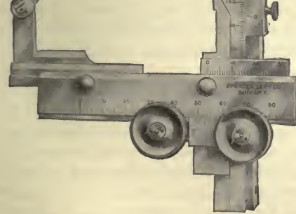
FIG. 71.—Attachable Mechanical Stage for Microscope.
