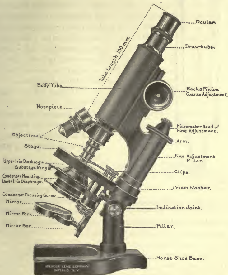
FIG. 54.—A Compound Microscope with Parts Named
