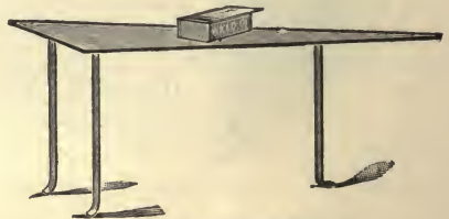
FIG. 26.—Imbedding-Table There should be two rectangular boxes (about 3×3×16 cm.) to contain paraffin. When in use the boxes are so placed on the imbedding-table that the paraffin in one end remains melted; in the other, solid. Regulate the temperature by placing the flame at the proper distance under the acute angle of the table. It is best, when gas is used, always to turn on the gas completely and then regulate the height of the flame by means of a clamp on the rubber tubing which conducts gas to the burner.
