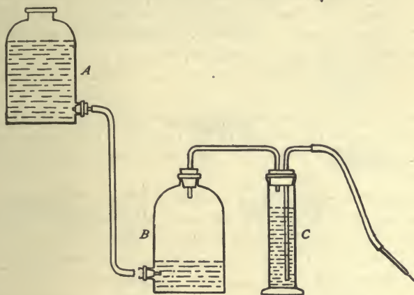
FIG. 35.—Apparatus for Continuous Air-Pressure Injection (after B. G. Smith)
