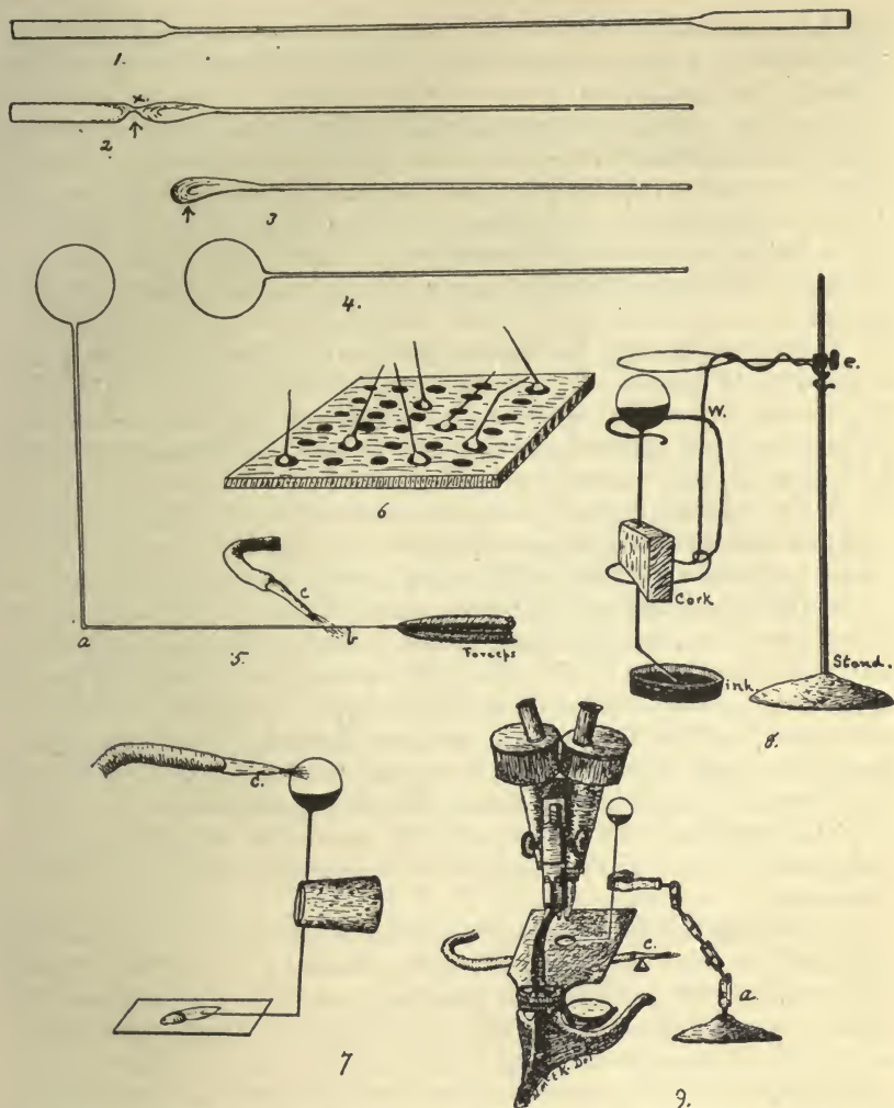
FIG. 36.—Apparatus for the Injection of Small Embryos, etc., under the Microscope (after Knower).
