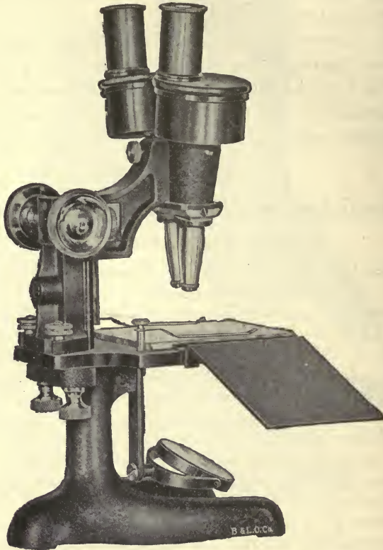
FIG. 61.—The Bausch & Lomb KA Binocular Dissecting Microscope, Greenough Type.
