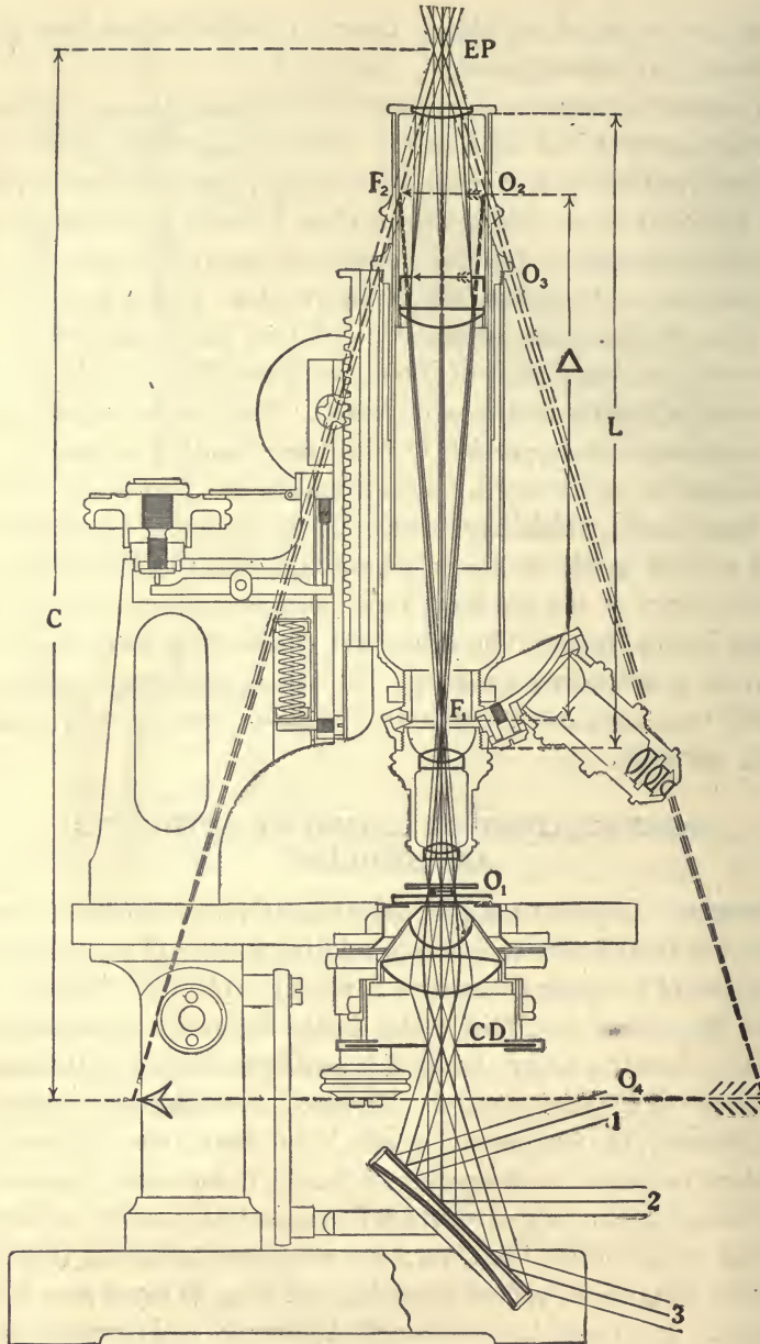
FIG. 58.—Diagram Showing Path of Light Rays through the Compound Microscope Together with Images (from Bausch and Lomb catalog).
