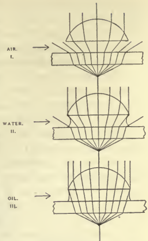
FIG. 70.—Diagram to Illustrate the Relative Amounts of Light Utilized with Dry, Water Immersion, and Homogeneous Oil Immersion Objectives Respectively (after Bausch).
