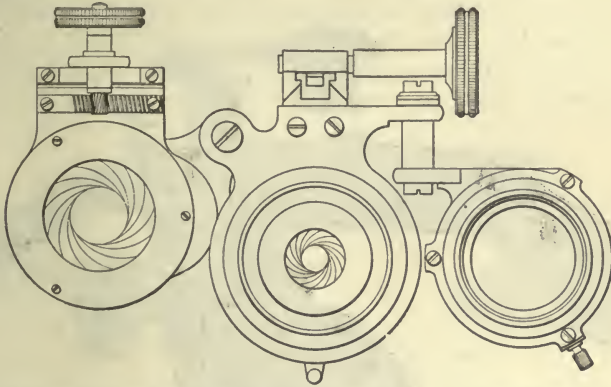
FIG. 66.—Top View of a Substage Attachment with Condenser and Lower Iris Diaphragm Thrown out of Optical Axis.
