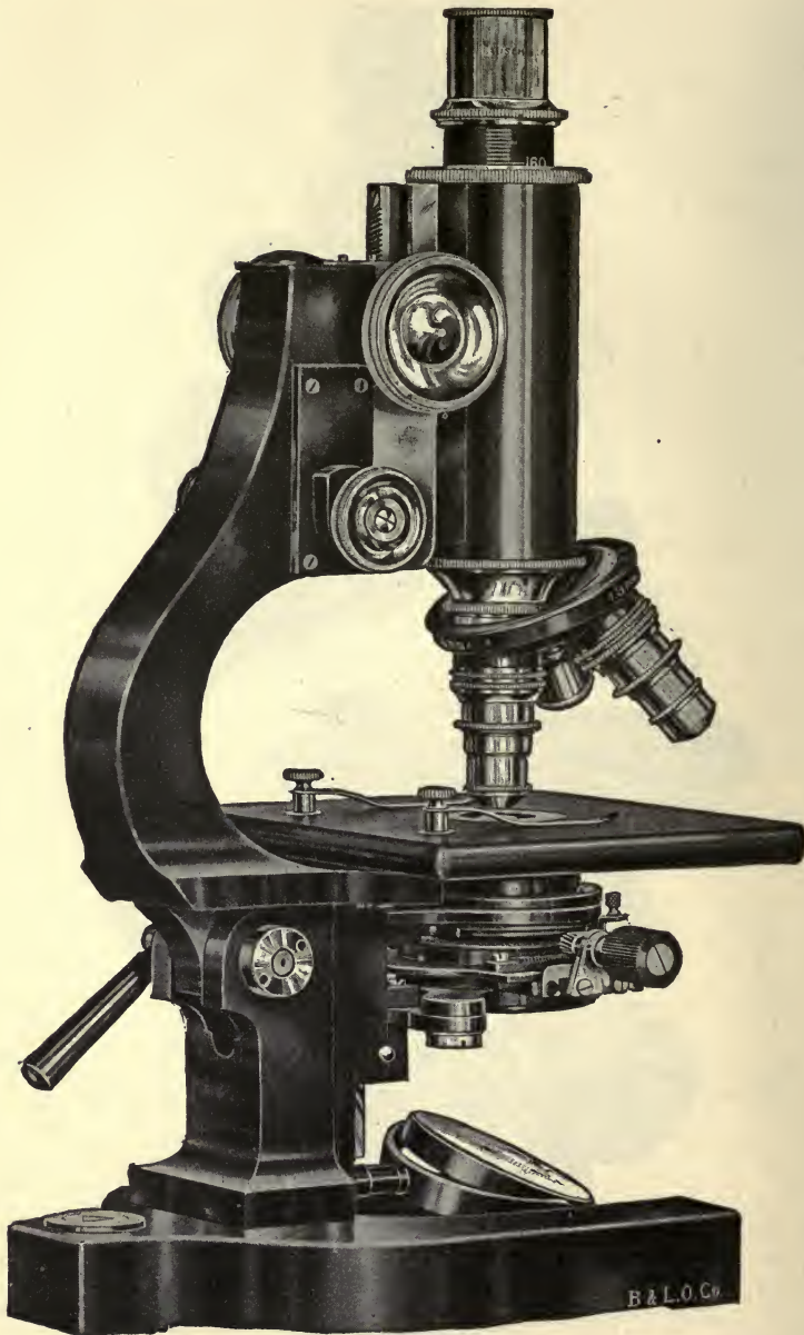
FIG. 60.—The Bausch & Lomb CAS Compound Microscope
