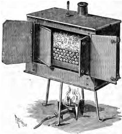
FIG. 4.—HOT-AIR CHAMBER FOR STERILISING TEST-TUBES AND COTTON-WOOL.
