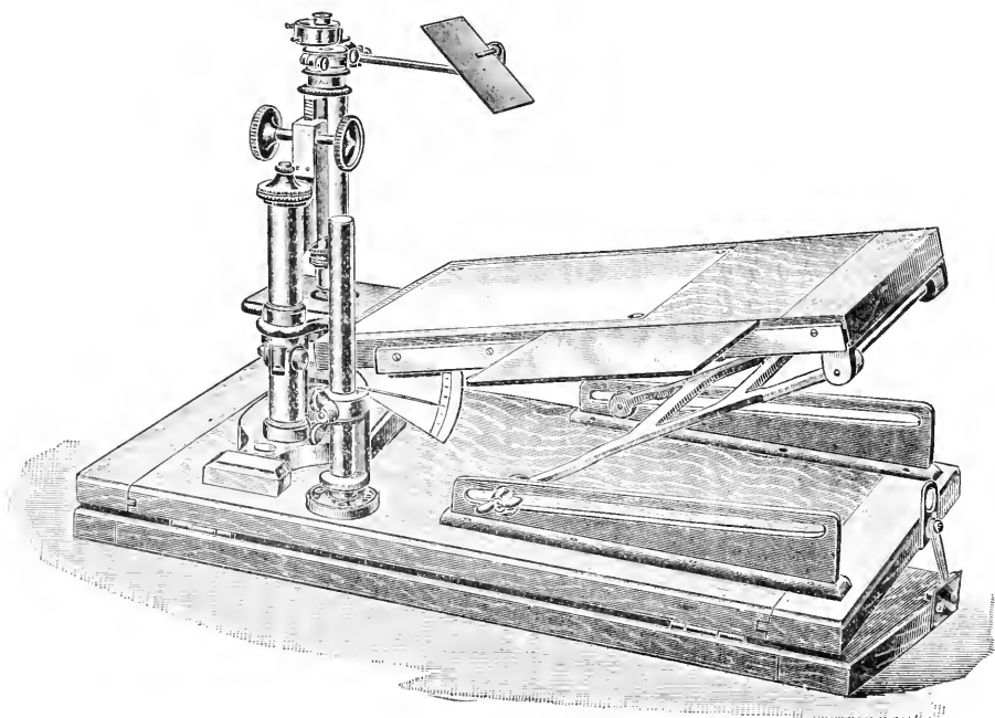
FIG. 111. Drawing Board for the Abbe Camera Lucida This drawing board, devised by the Bausch & Lomb Optical Co., is adjustable vertically, and the board may be inclined to prevent distortion. It is also arranged for use with an inclined microscope by having the base board hinged. Microscope and drawing surface are then inclined together. The camera lucida has a graduated arm to bear the mirror and a graduated quadrant at the mirror joint so that the angle of the mirror may be accurately determined. (See also Fig. 105. (From the Bausch & Lomb Optical Co.)
