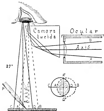
FIG. 105. Wollaston's Camera Lucida, showing the rays from the microscope and from the drawing surface, and the position of the pupil of the eye.
