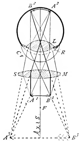
FIG. 38. Diagram of the simple microscope showing the course of the rays and all the images, and that the eye forms an integral part of it.
