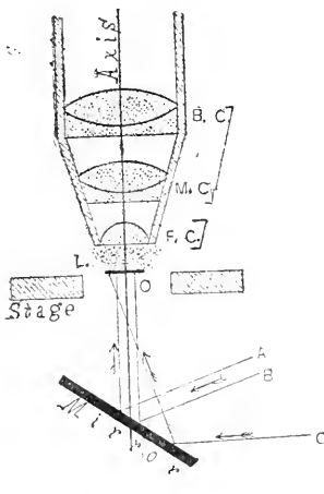
FIG. 23. Sectional view of an Immersion, Adjustable Objective, and the object lighted with axial and central and with oblique light.
