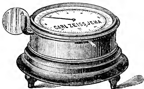
FIG. 122. Zeiss Cover-Glass Measurer. With this the knife edge jaws are opened by means of a lever, and the cover inserted. The thickness may then be read off on the face as the pointer indicates the thickness in hundredths millimeter in the outer circle and in hundredths inch on the inner circle.
