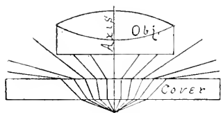
FIGS. 27-29 are somewhat modified from Ellenberger, and are introduced to illustrate the relative amount of utilized light, with dry, water immersion and homogeneous immersion objectives of the same equivalent focus. The point from which the rays emanate is in air in each case. If Canada balsam were in place of the air beneath the cover glass there would be practically no refraction of the rays on entering the cover glass ( \frac{1}{2} 16).
