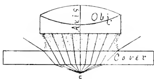
FIG. 29. Rays from an axial point of the object traversing a cover glass and entering the front of a homogeneous immersion objective.
