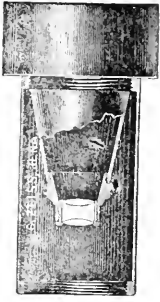
FIG. 149. Zeiss' Apochromatic, Projection Objective of 70 mm. equivalent focus, for photo-micrography. (Zeiss's Catalog. No. 30). This, and another of 35 mm. focus, are designed for making pictures of moderate magnification. Usually rather large objects are photographed with them. The object may be illuminated in the ordinary way. They are used without an ocular, like a photographic objective. The one of 35 mm. is screwed into the tube of the microscope like an ordinary objective, but the one of 70 mm. here shown, is, by means of a conical adapter, screwed into the ocular end of the tube.
