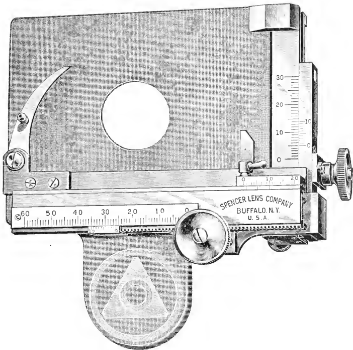
FIG. 70a.— Spencer-Winkel form of Mechanical Stage. It is readily attachable to any microscope with rectangular stage, by two clamping screws on the right. Its range of motion is about 30 \times 60 mm., thus enabling one to study as large a series as is usually put on an ordinary slide.
