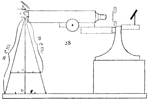
FIG. 95. Figure showing the position of the microscope, the camera lucida, and the eye, and the different sizes of the image depending upon the distance at which it is projected from the eye. (a) The size at 25 cm.; (b) at 35 cm., (§ 153).
