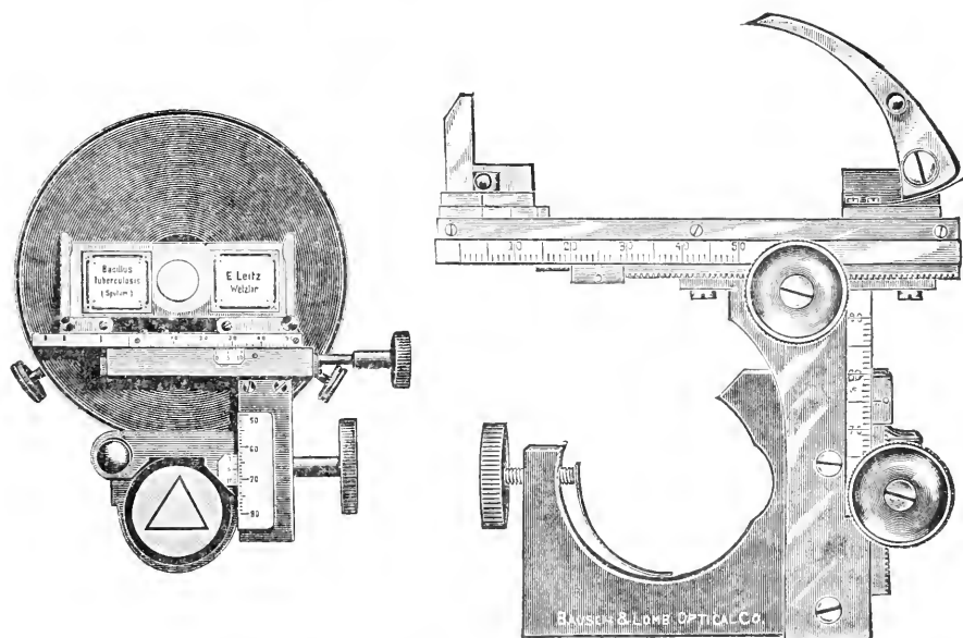
FIGS. 68-69. The Tolles-Mayall Mechanical Stage ( \frac{1}{2} 116).
