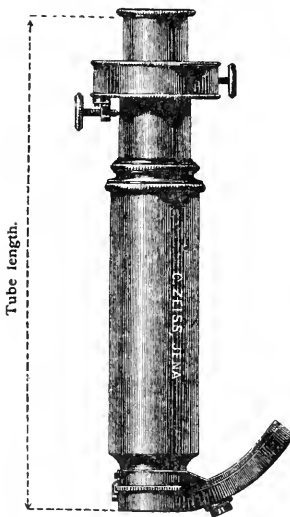
Fig. 25. The tube of a microscope with ocular micrometer and nose piece in position to show that in measuring tube-length one must measure from the eye lens to the place where the objective is attached. (Zeiss' Catalog, No. 30).
