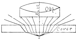
FIG. 27. Showing the course of the rays passing through a cover glass from an axial point of the object, and the number that finally enter the front of a dry objective.
