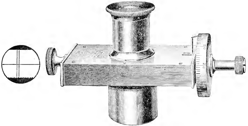
FIGS. 98, 99. Filar Ocular Micrometer with Field (Bausch & Lomb, Optical Co.). For other ocular micrometers see pp. 25, 26.
