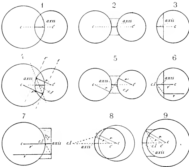
FIG. 167. SPHERICAL LENSES WITH THEIR FORMS AND PRINCIPAL FEATURES.
