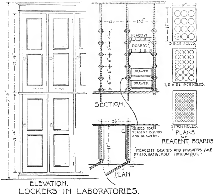
FIG. 208. LABORATORY LOCKERS REAGENT BOARDS AND DRAWERS DESIGNED IN 1895.
