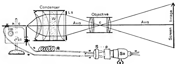
FIG. 110. MAGIC LANTERN WITH PROJECTED IMAGE.
