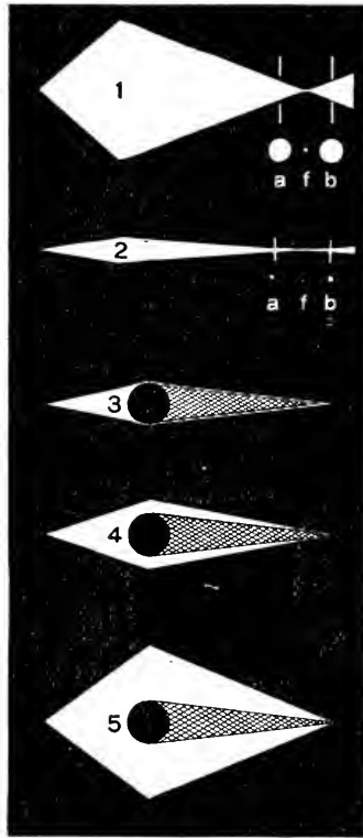
FIG. 180. EFFECT OF APERTURE ON DEFINITE FOCUS AND ON OVERCOMING OPACITIES.
