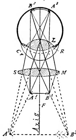
FIG. 5-6. VISION BY THE UNAIDED EYE AND BY THE AID OF A SIMPLE MICROSCOPE.
