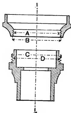
FIG. 64. ROYAL MICROSCOPICAL SOCIETY'S STANDARD SCREW FOR OBJECTIVES.
