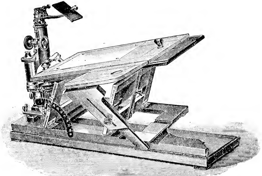
FIG. 102. BERNHARD'S DRAWING BOARD FOR THE ABBE CAMERA LUCIDA.
