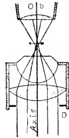
FIG. 41. SUBSTAGE CONDENSER OF ABBE WITH PARALLEL LIGHT.
