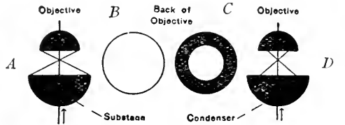
FIG. 45. APERTURE OF THE SUBSTAGE CONDENSER AND OF THE OBJECTIVE. (From Nelson, Jour. Roy. Micr. Soc.).
