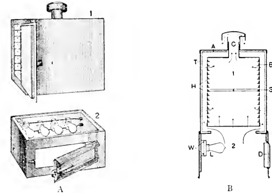
FIG. 244. DRYING OVEN FOR SLIDE TRAYS.
