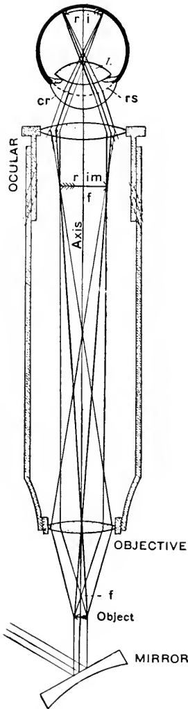
FIG. 3. A COMPOUND MICROSCOPE HELPING THE EYE TO FORM A RETINAL IMAGE OF A NEAR OBJECT.
