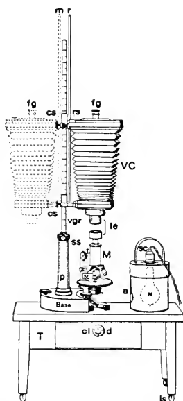
FIG. 129. VERTICAL MICROSCOPE AND CAMERA FOR PHOTO-MICROGRAPHY. (About \frac{1}{20} natural size).
