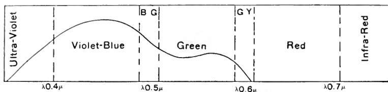
FIG. 141. NORMAL SPECTRUM SHOWING THE SENSITIVENESS OF ORTHOCHROMATIC OR ISOCHROMATIC PLATES.
