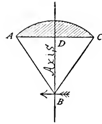
FIG. 176. ANGULAR APERTURE OF AN OBJECTIVE.
