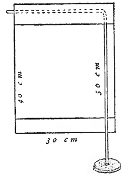
FIG. 33. SCREEN FOR SHADING THE MICROSCOPE AND THE OBSERVER.
