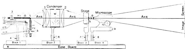
FIG. 111. PROJECTION MICROSCOPE.
