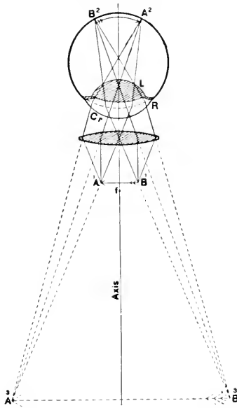
FIG. 182. PROJECTED VIRTUAL IMAGE OF A MAGNIFIER. (Simple Microscope or Ocular).
