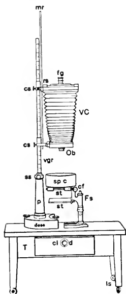
FIG. 126. VERTICAL PHOTOGRAPHIC CAMERA.
