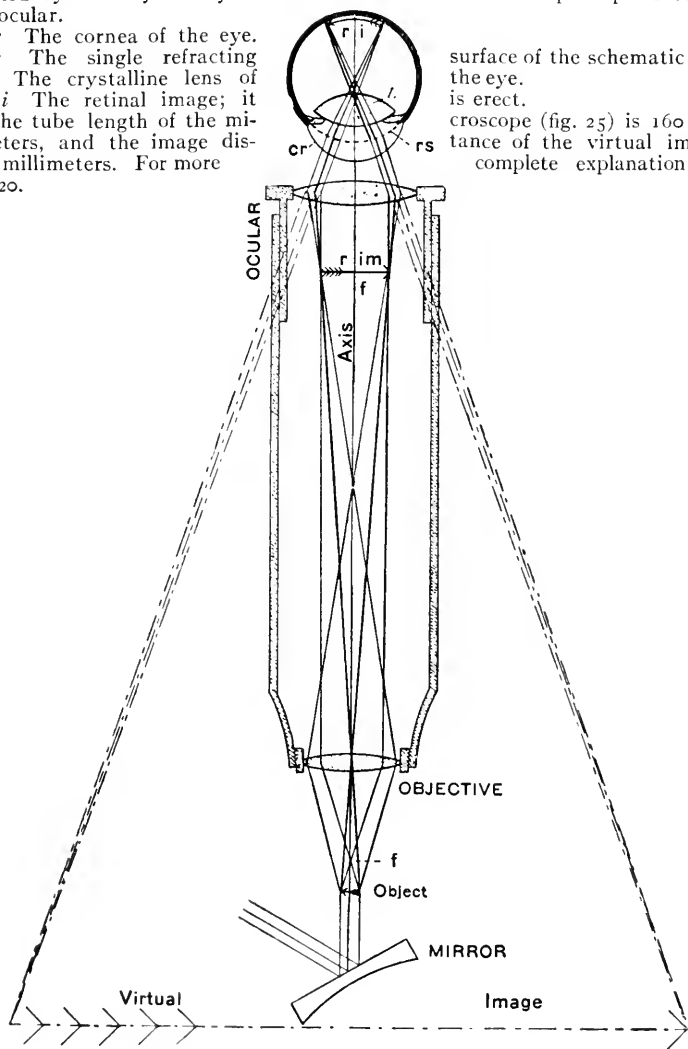
FIG. 78. COMPOUND MICROSCOPE SHOWING ALL THE IMAGES.
