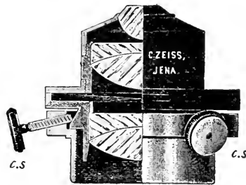
FIG. 40. ACHROMATIC SUBSTAGE CONDENSER WITH THE DIAPHRAGM BETWEEN THE COMBINATIONS.
