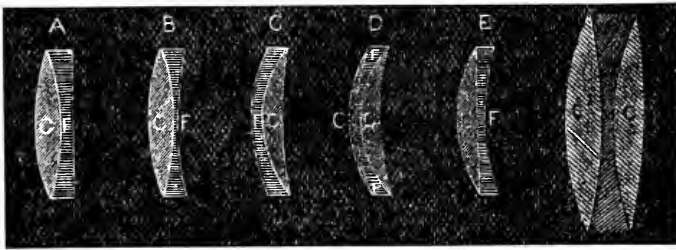
FIG. 173. ACHROMATIC COMBINATIONS OF CROWN AND FLINT GLASS LENSES.
