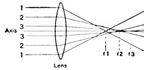
FIG. 168. SPHERICAL ABERRATION IN LENSES.
