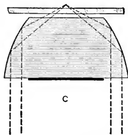
FIG. 50. CONDENSER FOR DARK-GROUND ILLUMINATION.
