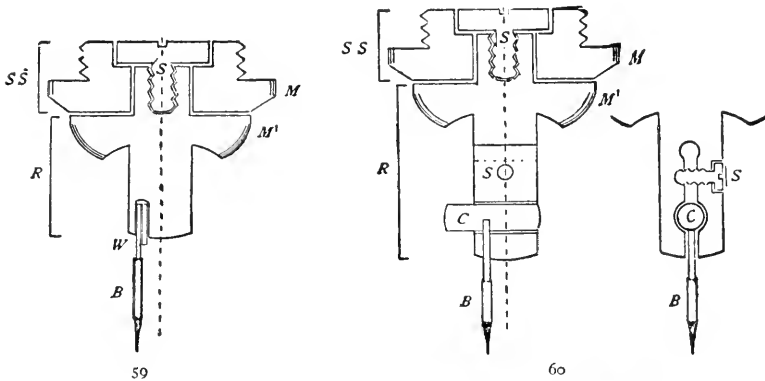
FIG. 59-60. MARKERS FOR MICROSCOPICAL SPECIMENS.
