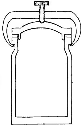
FIG. 214. SPECIMEN JAR WITH CLAMP.
