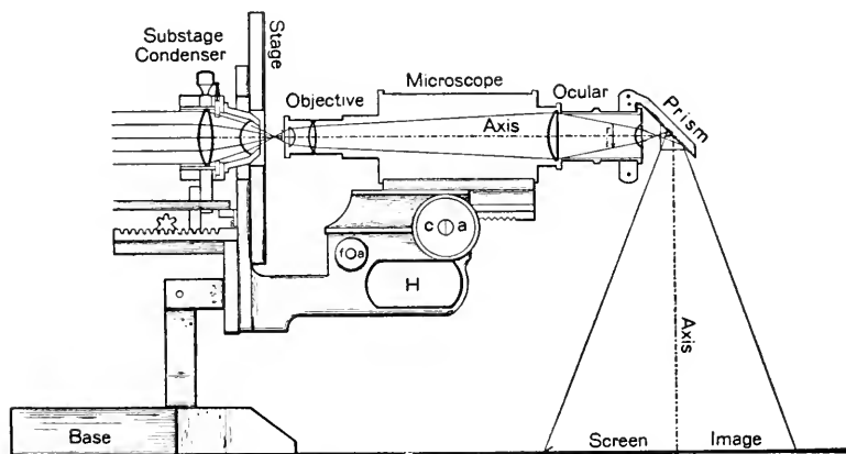
FIG. 114. THE MICROSCOPE ARRANGED FOR DRAWING ON A HORIZONTAL SURFACE.
