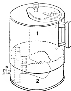
FIG. 210. KINGSBURY'S PARAFFIN MELTING OVEN.
