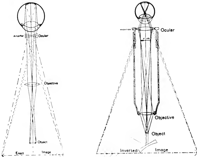
FIG. 248, 249. DUTCH AND KEPLERIAN COMPOUND MICROSCOPES FOR COMPARISON.
