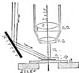
FIG. 34. LOW-POWER OBJECTIVE SHOWING WORKING DISTANCE AND REFLECTED LIGHT.
