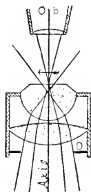
FIG. 42. SUB-STAGE CONDENSER WITH CONVERGING LIGHT.
