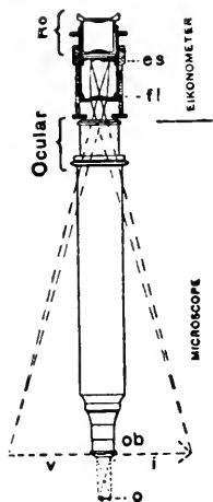
FIG. 96. WRIGHT'S EIKONOMETER.
