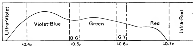
FIG. 142. NORMAL SPECTRUM SHOWING THE SENSITIVENESS OF PANCHROMATIC PLATES.
