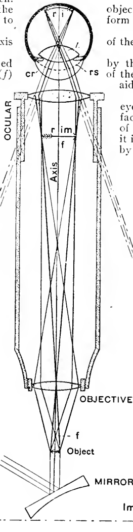
FIG. 20. COMPOUND MICROSCOPE WITH PROJECTED VIRTUAL IMAGE.
