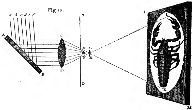
FIG. 79. REAL IMAGE FORMED BY A PROJECTION MICROSCOPE.
