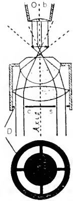
FIG. 47. DARK-GROUND ILLUMINATION BY A HOLLOW CONE OF LIGHT.
