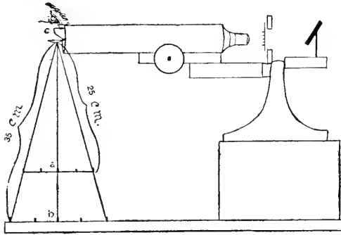
FIG. 85. DIAGRAM TO SHOW THAT THE SIZE OF THE VIRTUAL IMAGE DEPENDS UPON THE PROJECTION DISTANCE.
