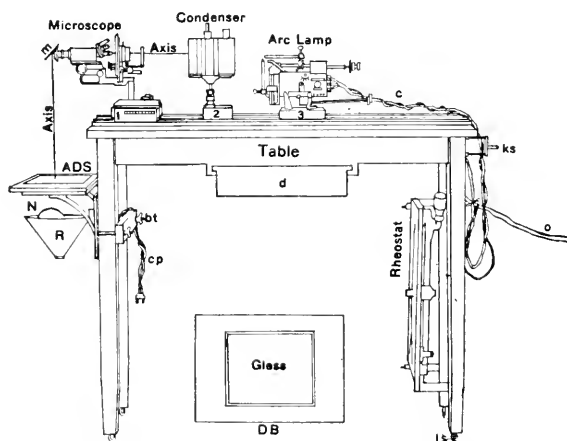
FIG. 247. DRAWING AND PROJECTION OUTFIT.
