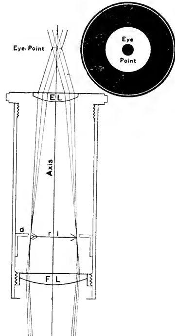
FIG. 23. LOW-POWER HUYGENIAN OCULAR IN SECTION.
