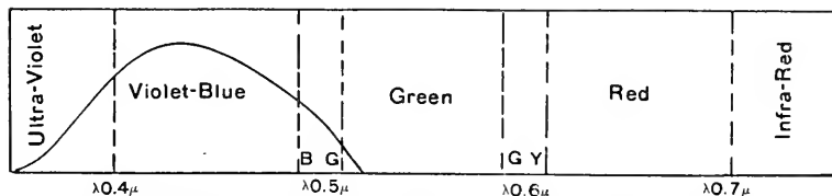
FIG. 140. NORMAL SPECTRUM SHOWING THE SENSITIVENESS OF ORDINARY PHOTOGRAPHIC PLATES.
