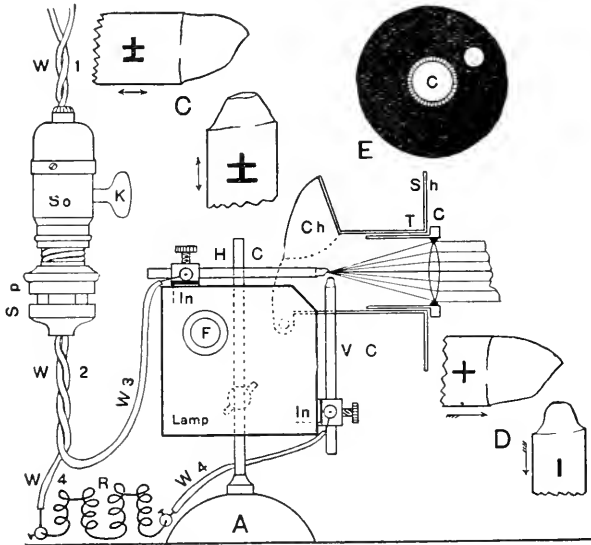
FIG. 49. SMALL ARC LAMP AND CONNECTIONS. (From Optic Projection).
