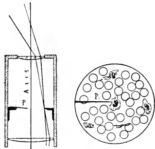
FIG. 62-63. POINTER OCULAR AND MICROSCOPIC FIELD.
