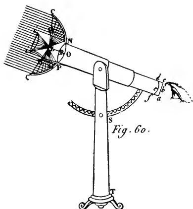
FIG. 251. DESCARTES' DUTCH COMPOUND MICROSCOPE WITH A PARABOLIC MIRROR AND A CONDENSING LENS.
