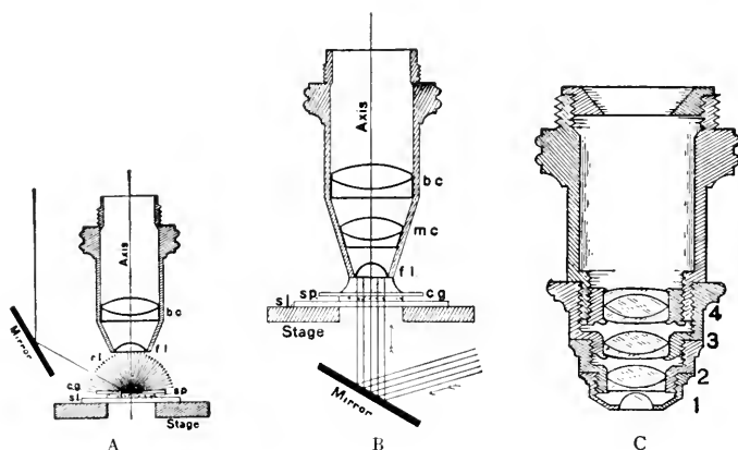
FIG. 21 A. LOW OBJECTIVE IN SECTION.
