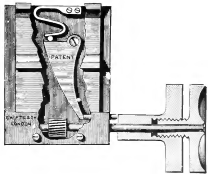
FIG. 149.—Karop's fine adjustment for sub-stage, made by Swift (1892).
