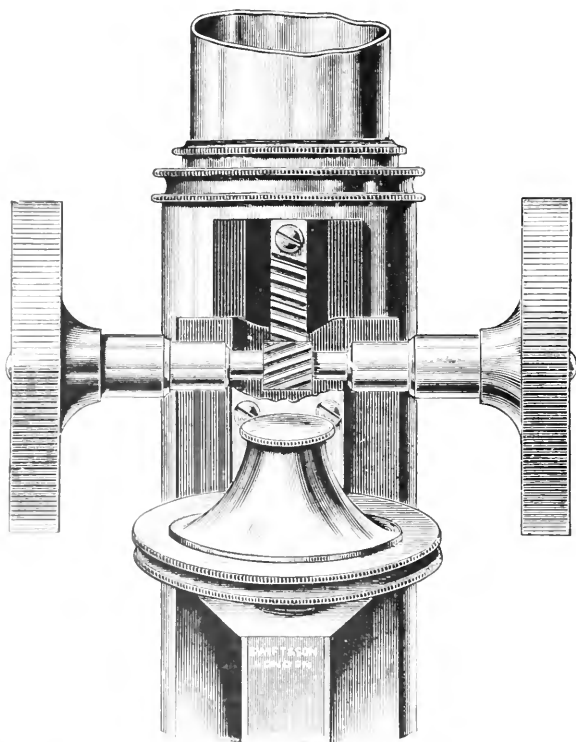
FIG. 121. Diagonal rack and twisted pinion devised in 1881.
