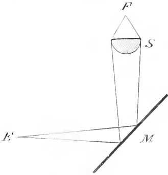
FIG. 348.—Another method of getting critical image.
