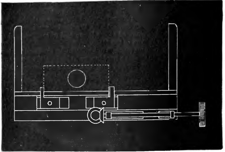
FIG. 142. Nelson's new mechanical stage (1897).
