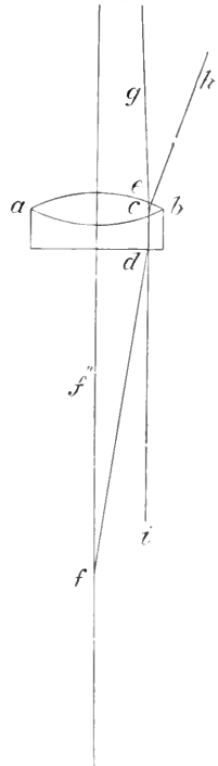
FIG. 309.—The two aplanatic foci of an optical combination.
