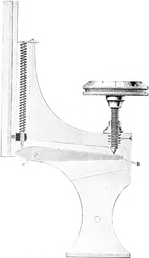
FIG. 132. Watson's lever fine adjustment (1889).
