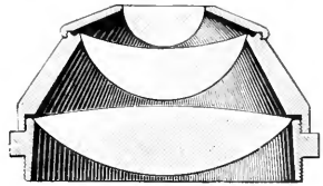
FIG. 254.—Optical arrangement of Abbe's chromatic condenser.
