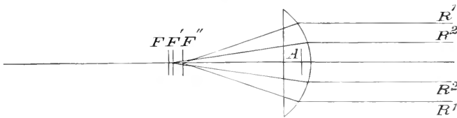
Fig. 18.—Spherical aberration.
