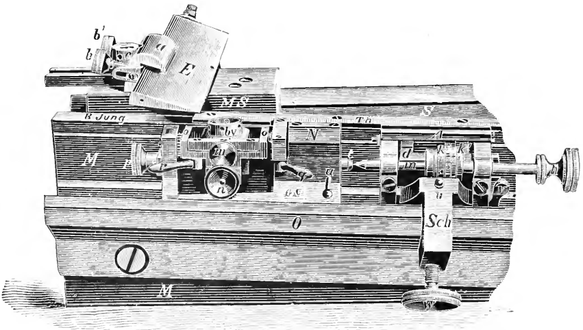
FIG. 392.—The Thoma microtome with the usual zoologist's knife.
