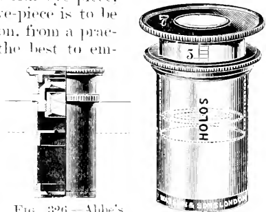
FIG. 327.—Watson's holoscopic eye-piece.
