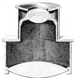
FIG. 323.—Kellner eye-piece.
