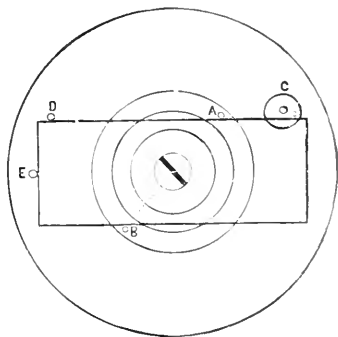
FIG. 381.—Griffith's turn-table.
