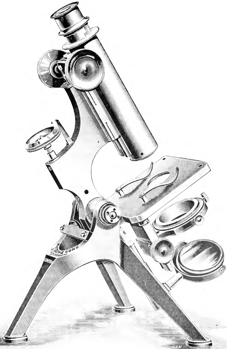
FIG. 179.—Watson's Edinburgh Student's; stand 'G' (1893).
