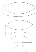
FIG. 318.—Combination for 'homogeneous' immersion by Abbe.
