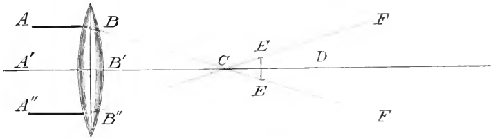
FIG. 19.—Chromatic aberration.
