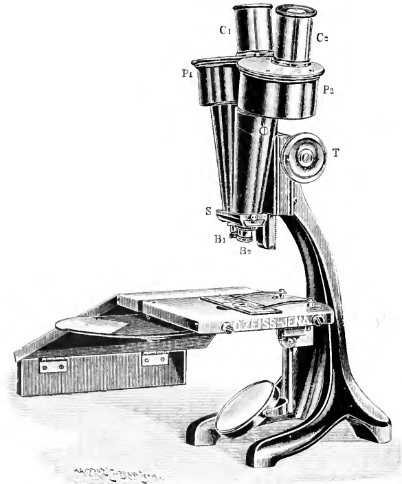
FIG. 201. — Greenough's binocular, arranged as a dissecting microscope (1897).
