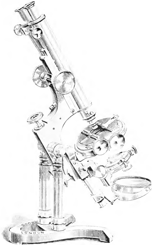
FIG. 125.—Ross-Zentmayer model 1878.
