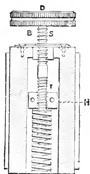
FIG. 126.—Campbell's differential screw fine adjustment (1886).
