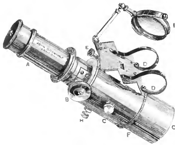
FIG. 269.—Micro-spectroscope.
