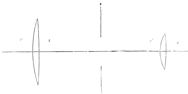
FIG. 324.—Nelson's new formula Huyghenian eye-piece.
