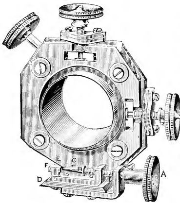
FIG. 148.—Fine adjustment to sub-stage. Powell (1882).
