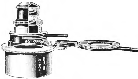
FIG. 245.—Watson's parachromatic condenser.
