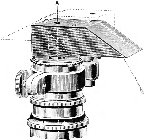
FIG. 225.—Bausch and Lomb's modification of Abbe's camera.
