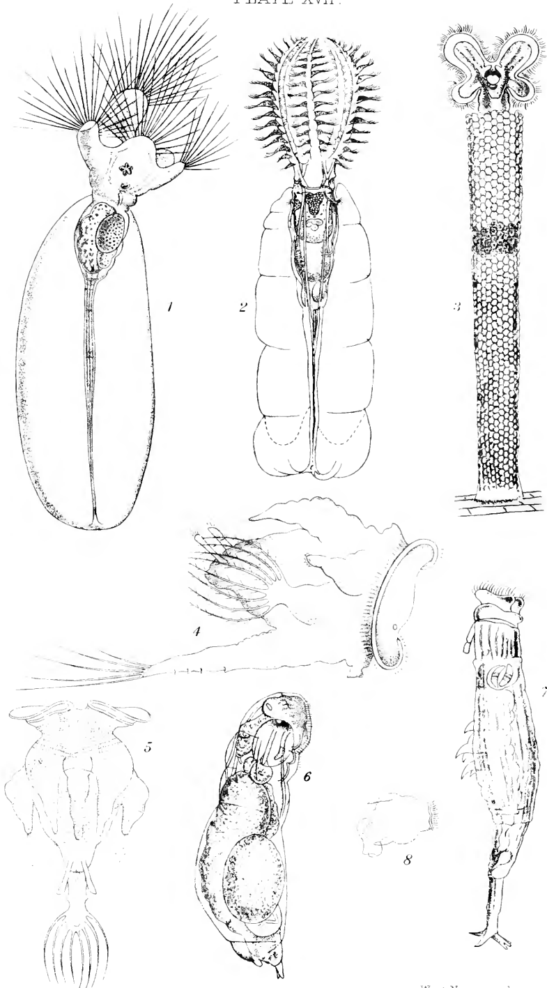
Typical Rotifers
