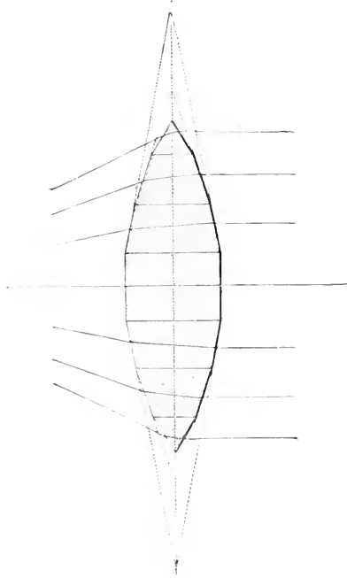
FIG. 7.—Proof that a lens may be considered as an assemblage of prisms. (From the 'Forces of Nature'.)
