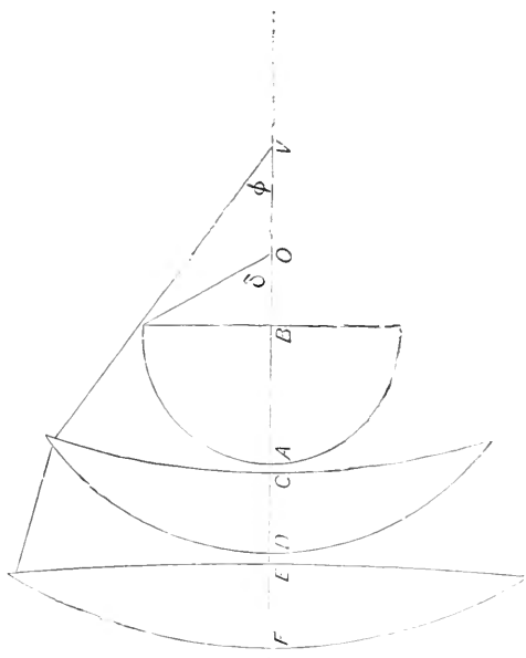
FIG. 320.—Nelson's new immersion front for a condenser.
