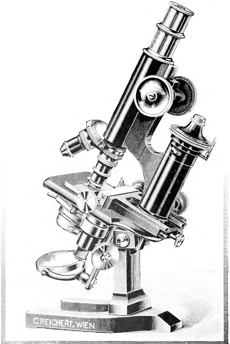
Fig. 168. One of Reichert's large stands (Hb) with new lever fine adjustment fitted (1899).
