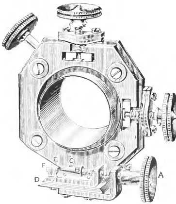
FIG. 158.—Powell and Lealand's sub-stage with fine adjustment (1882).
