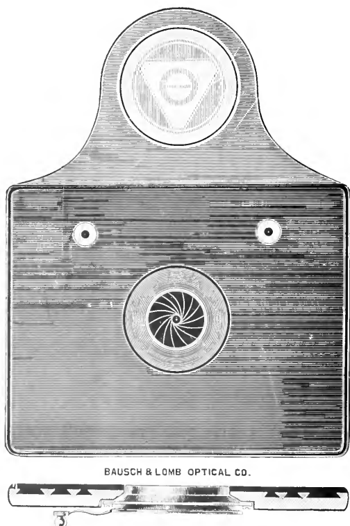
FIG. 147A.—Attachable stage with diaphragm in the plane of the stage. Top view and cross section showing construction of stage and attachment of iris diaphragm.
