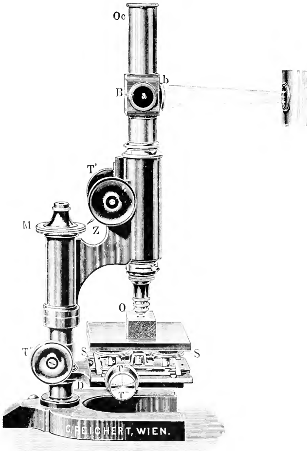
FIG. 207.—Reichert's microscope for the examination of metals (1897).
