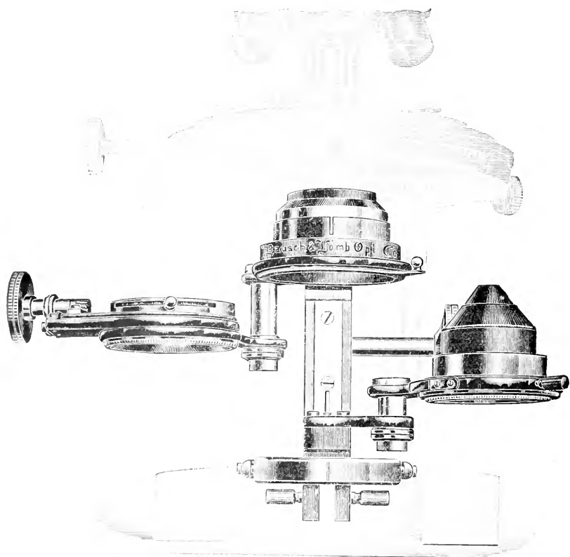
FIG. 171. —Bausch and Lomb's sub-stage, separated to show construction.
