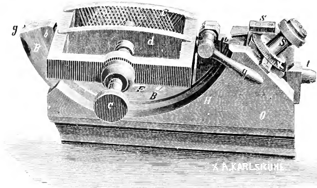
FIG. 395.—Object-holder for analysis by diversified section.
