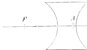
FIG. 25A.—Focus of a concave lens.
