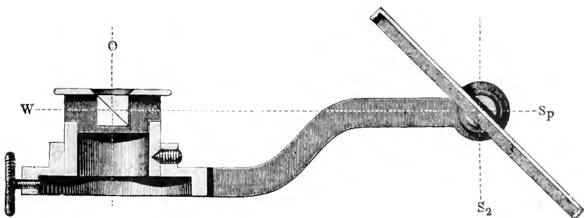
FIG. 220.—Abbe's camera lucida.
