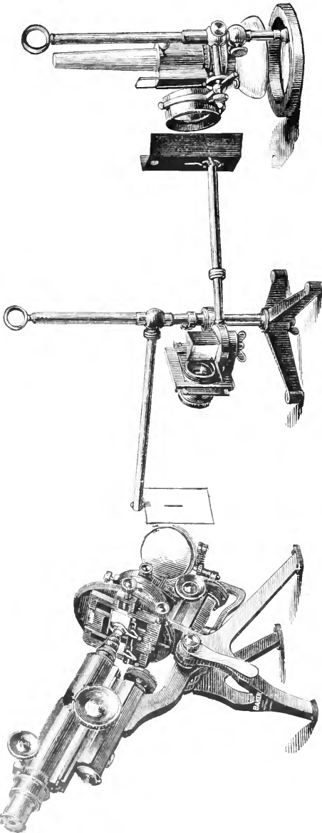
FIG. 268.—Mr. Nelson's apparatus for obtaining monochromatic light.
