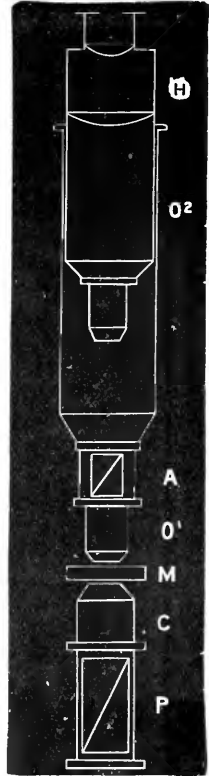
FIG. 265.—In this diagram P is the polarising prism in the sub-stage, C sub-stage condenser. On the stage M mineral. On nose-piece O 1 objective \frac{4}{10} ths \cdot 64 N.A.; A analysing prism. In the draw-tube, O 2 objective 2 or 3 in. H, Huyghenian eye-piece.
