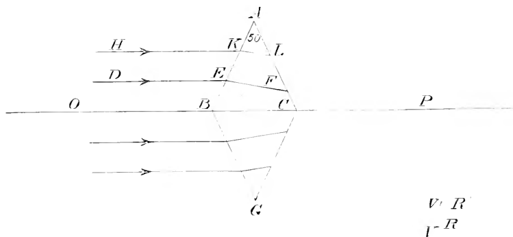
FIG. 8.—Action of a pair of prisms with their bases in contact on parallel light.
