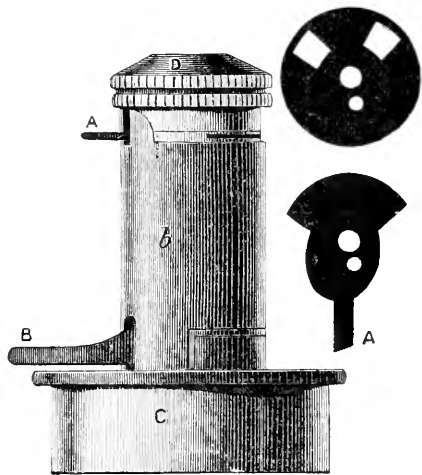
FIG. 256.—Powell and Lealand's chromatic oil condenser (1880).
