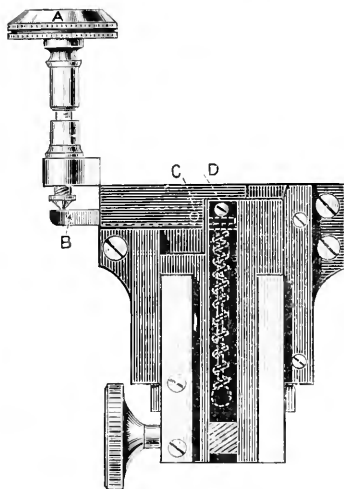
FIG. 150. Watson's sub-stage fine adjustment (1899).
