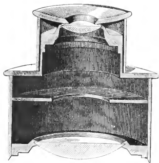
FIG. 322.—Huyghenian eye-piece.
