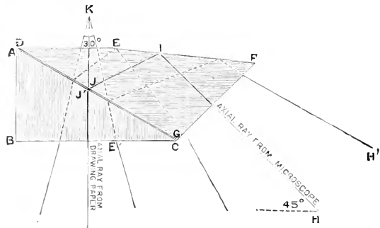
FIG. 227.—Diagram explaining Schröder's camera lucida.
