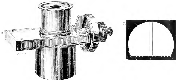
FIG. 212.—The micrometer eye-piece.
