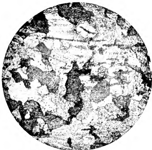
FIG. 208.—Wrought iron magnified 250 diameters.
