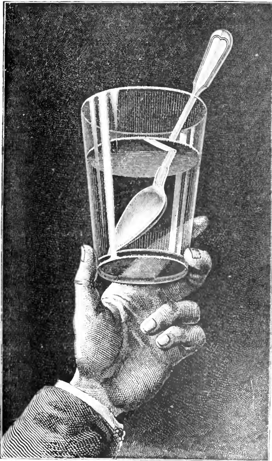
FIG. 3. — The phenomenon of total reflexion. (From the 'Forces of Nature,' published by Macmillan.)
