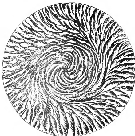
FIG. 816. —Spiral crystallisation of copper sulphate.
