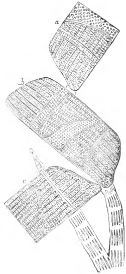
FIG. 457.— Isthmia nervosa .
