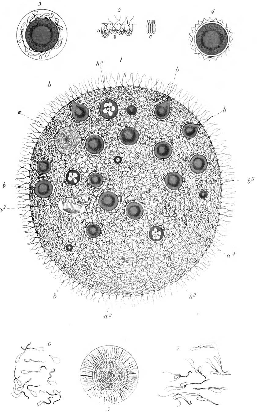
Volvox globator .
