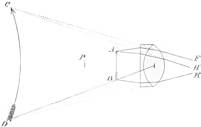
FIG. 27.—The formation of a 'virtual image.'
