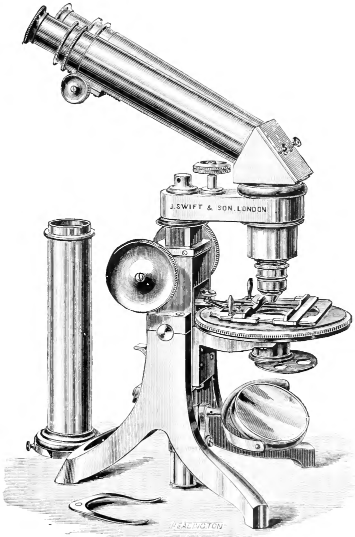
FIG. 200.—Stephenson's binocular by Swift (1887).
