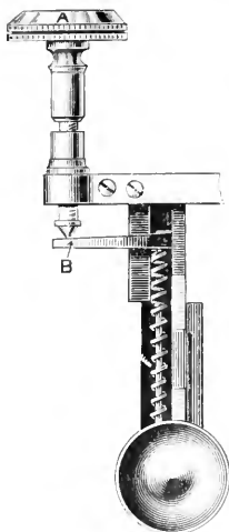
FIG. 150. Watson's sub-stage fine adjustment (1899).
