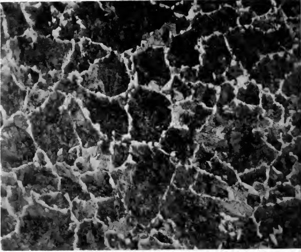
PHOTOGRAPH NO. 5. X75. 0.57% carbon. Ferrite and pearlite.
