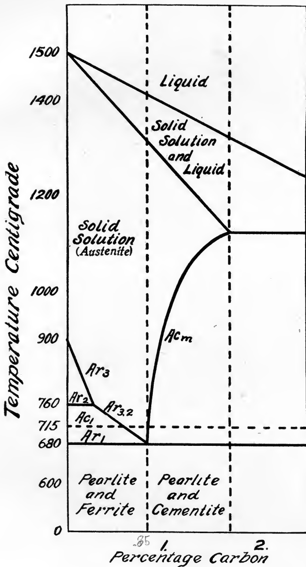
Portion of iron-carbon diagram
