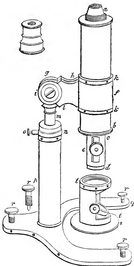
Goring's Megaloscope, one-sixth its real size.
