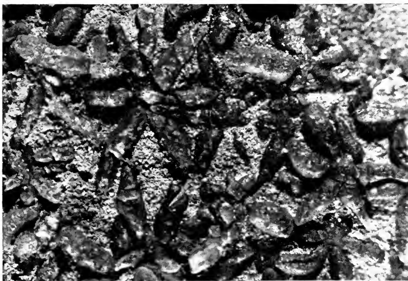
FIG. 36. Astraeospongia clauda , sp. nov. Spicules enlarged, showing impressing of overlapping rays and thin distal projection of rays, probably representing filling of axial canal. Holotype, C.N.H.M. PE999. \times 12.3 .
