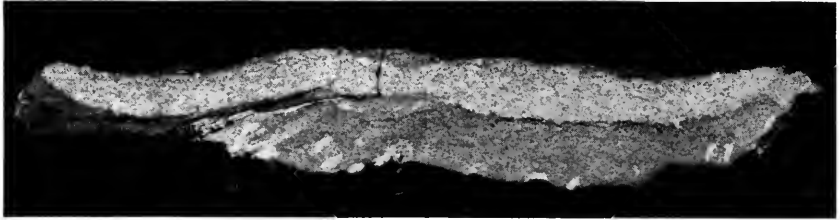
FIG. 34. Astraeospongia clauda , sp. nov. Cross section on a diameter, oral surface at top. The shape is the result of collapse of an originally cup-like form. Holotype, C.N.H.M. PE999. \times 1 .
