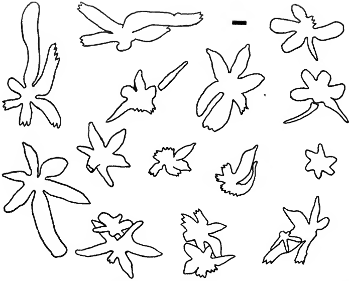
FIG. 37. Spicules of Astraeospongia clauda , sp. nov. Rays terminating in a jagged line pass beneath the matrix or another spicule. The black line represents one millimeter, to the same scale of magnification as the spicules. Camera lucida drawings from holotype, C.N.H.M. PE999. \times 5 .
