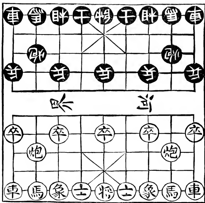
Chinese Chess-board.
