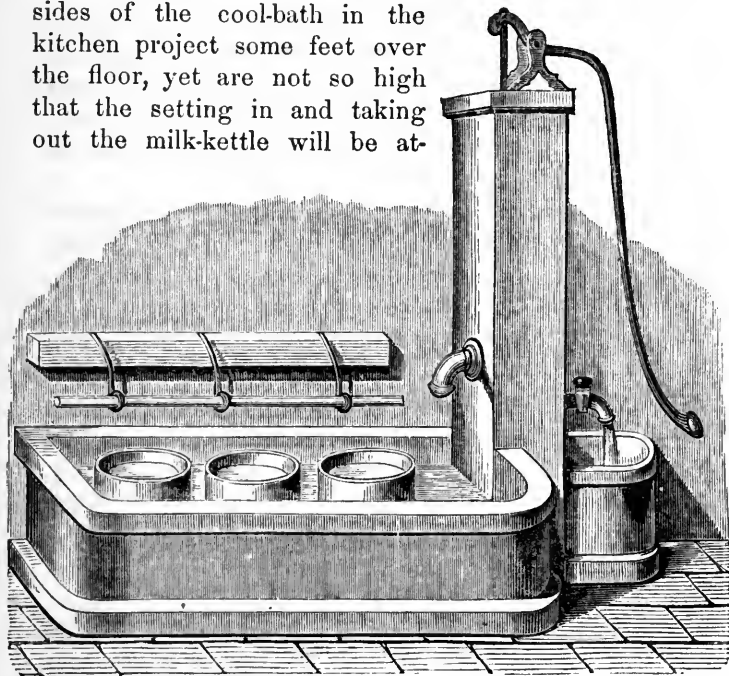
Fig. 96. Cool-bath.
