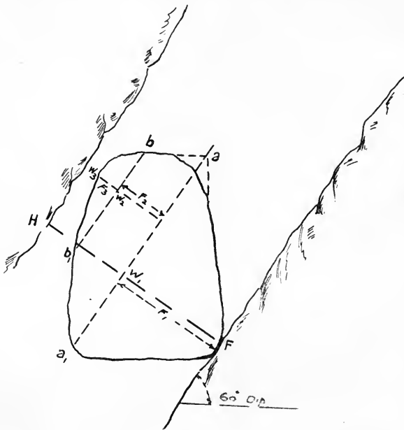
Fig. 9. INCLINED OREBODY, ONE WALL EXPOSED.
