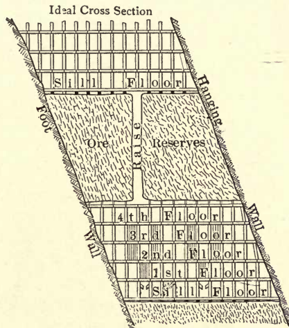
FIG. 59. — WORKING FLOORS AT ROSSLAND, B.C.
