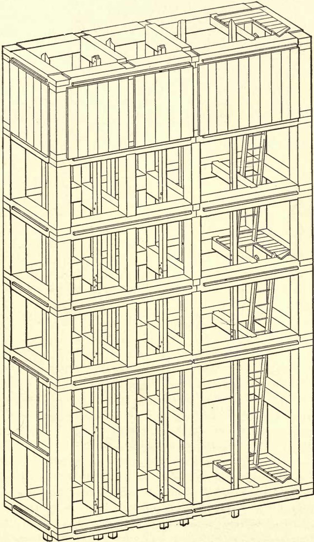
FIG. 31. — FRAMING OF THREE-COMPARTMENT SHAFT. Perspective.
