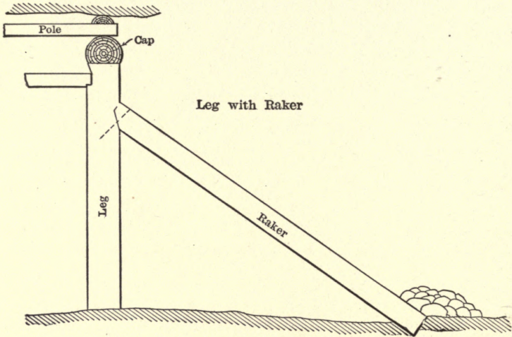
FIG. 91. — RAKER, SECTION 16 MINE.
