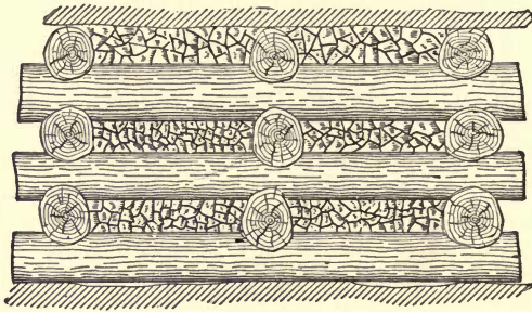
FIG. 43. — CRIB WITH WASTE FILLING.
