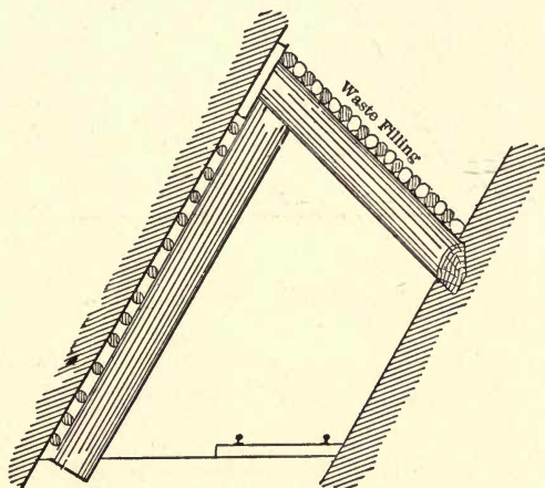
FIG. 36. — TWO-PIECE SET.
