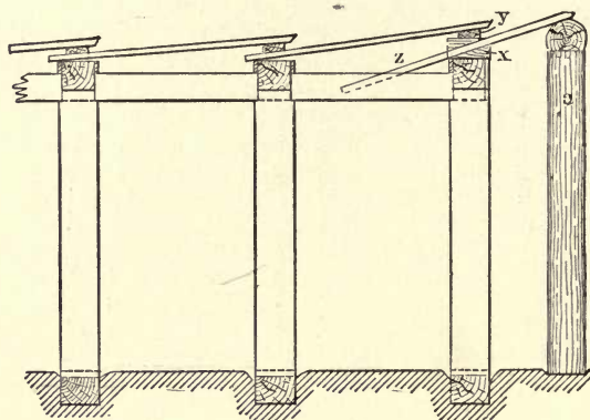
FIG. 40. — SPILING IN LOOSE GROUND.
