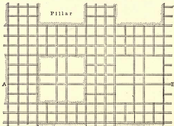
Plan of Stope, Queen Mine. Negaunee, Mich.
