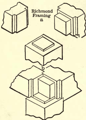
FIG. 55.—RICHMOND METHOD.
