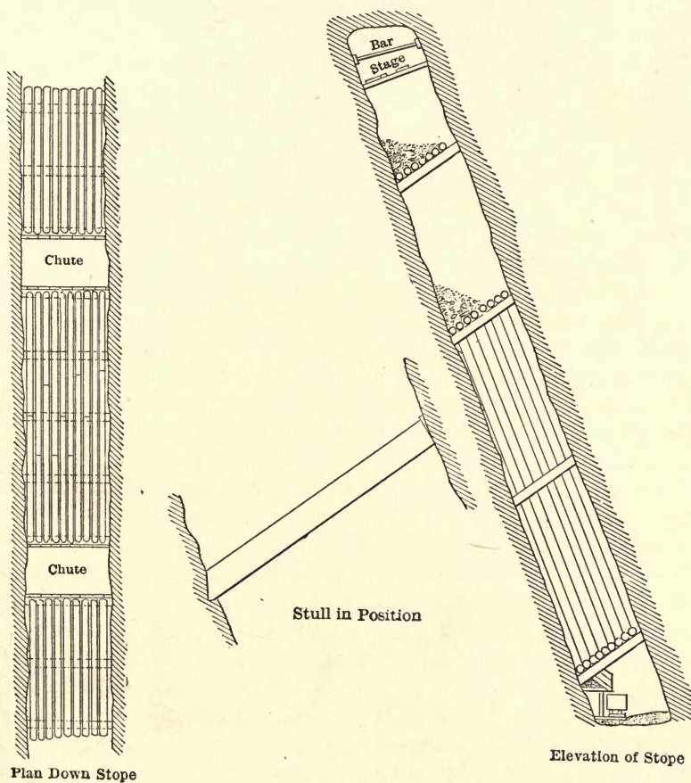
FIGS. 64-66. — STULL TIMBERING, LE ROI MINE.
