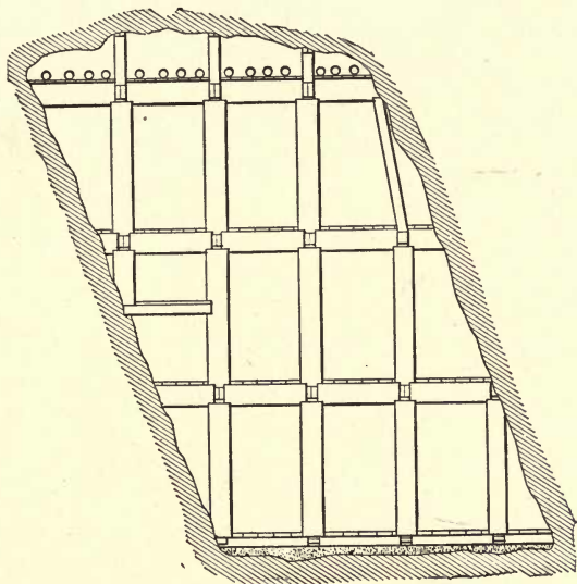
FIG. 69. — SQUARE SETS IN POSITION, LE ROI MINE.
