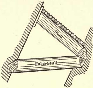
FIG. 45. — STULL AND FALSE STULL.
