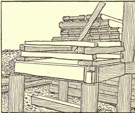
FIG. 115. — SQUARE-SET TIMBERS.
