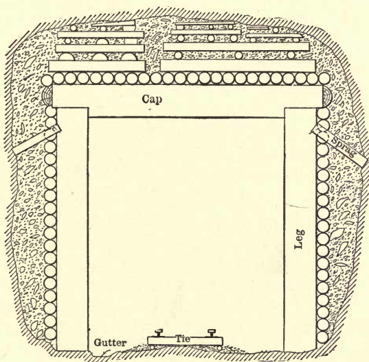
FIG. 90. — END VIEW OF DRIFT SET, SECTION 16 MINE.
