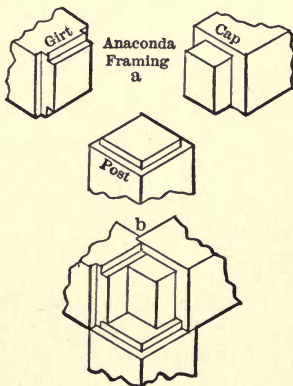
FIG. 52. — ANACONDA METHOD.
