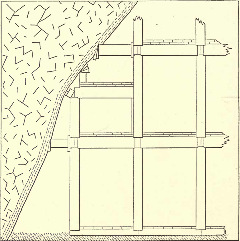
FIG. 104. — SHORT SETS.
