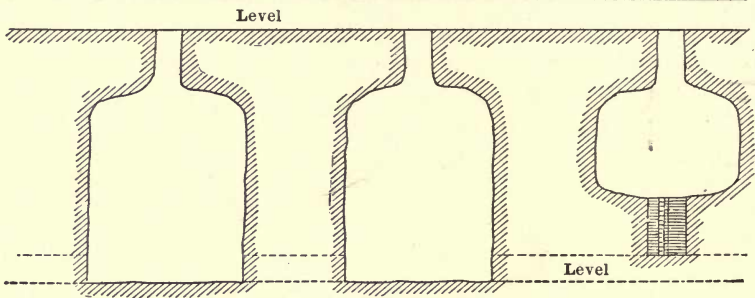
FIG. 82. — STOPES AND PILLARS.
