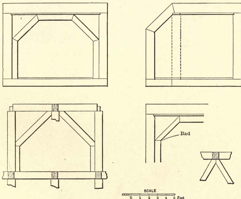
FIGS. 127-131. — DETAILS OF FRAMING.
