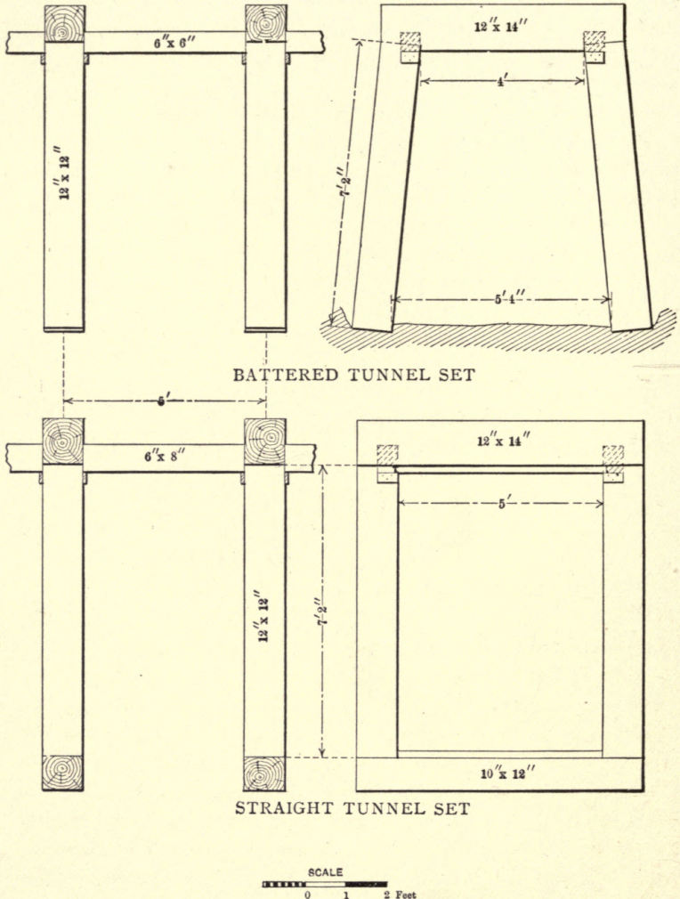
FIG. 118. — BATTERED AND STRAIGHT TUNNEL SETS.
