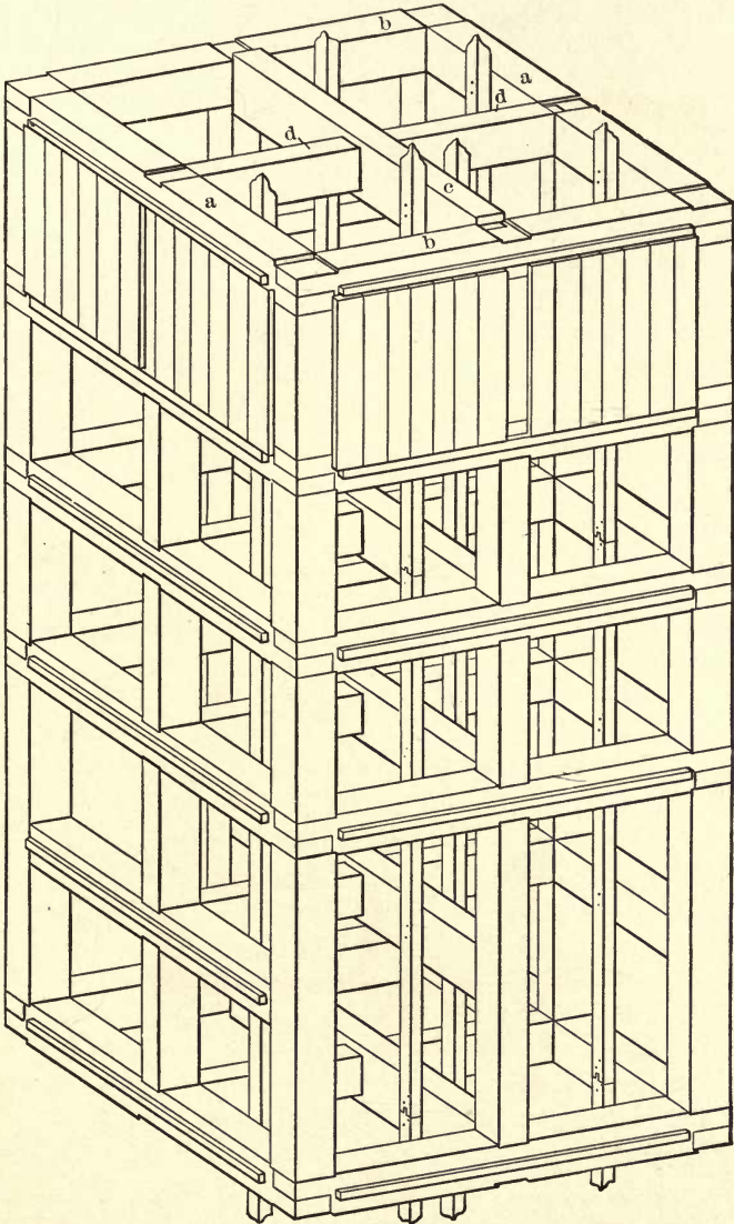
FIG. 34. — FRAMING OF DOUBLE-WIDTH FOUR-COMPARTMENT SHAFT. Perspective.
