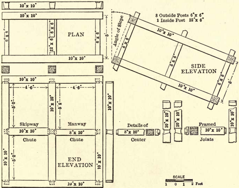
FIG. 121. — FOUR-COMPARTMENT SHAFT.
