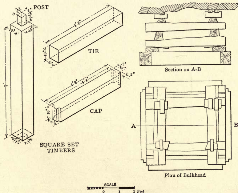
FIGS. 110-114. — SQUARE-SET TIMBERS.
