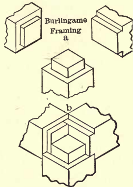
FIG. 54.—BURLINGAME METHOD.
