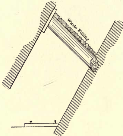
FIG. 35. — SINGLE-PIECE SET.
