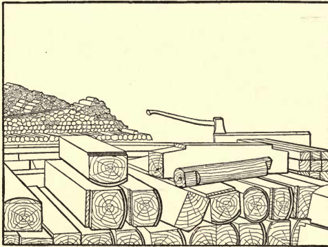
FIG. 119. — TUNNEL-SET TIMBERS.
