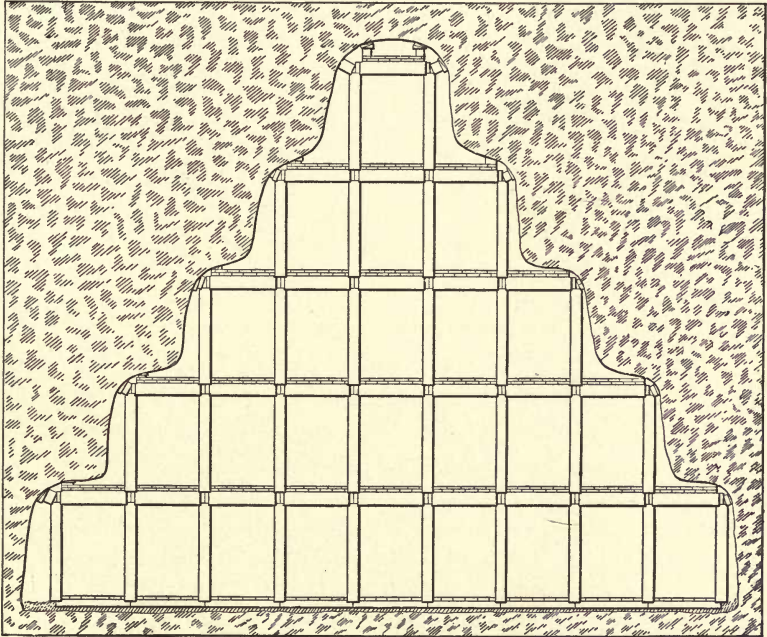
FIG. 102. — TRANSVERSE SECTION OF STOPE.
