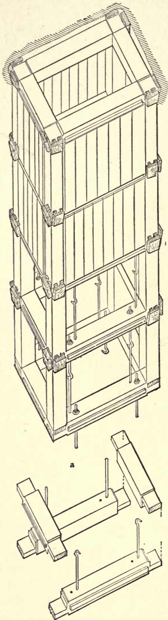
FIG 27. — TIMBERING OF A ONE-COMPARTMENT SHAFT. Perspective.
