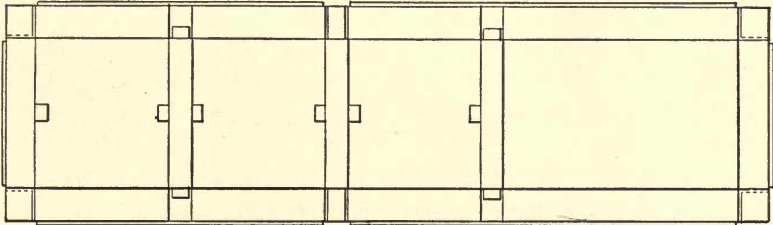
FIG. 32. — FRAMING OF SINGLE-WIDTH, FOUR-COMPARTMENT SHAFT.
