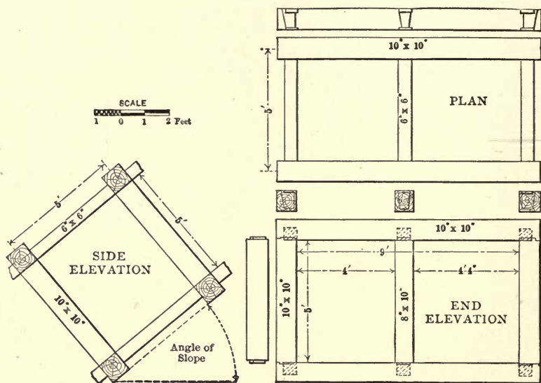
FIG. 120. — TWO-COMPARTMENT SHAFT.
