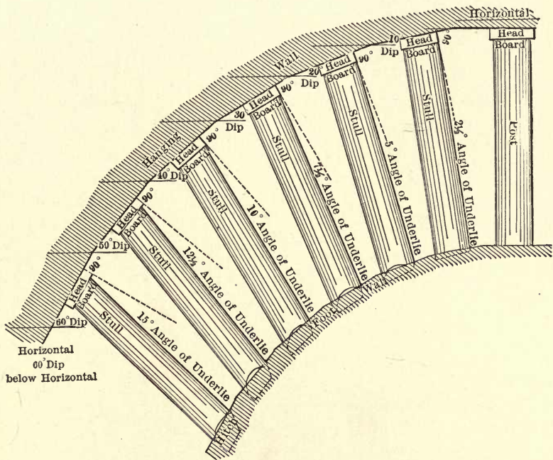
FIG. 50. — ANGLE OF UNDERLIE OF STULLS.
