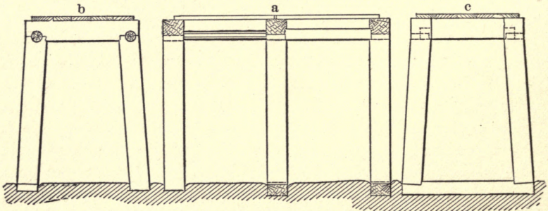
FIG. 38. — THREE-PIECE SET.
