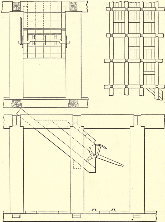
FIGS. 70-72. — VIEWS OF CHUTE, LE ROI MINE.
