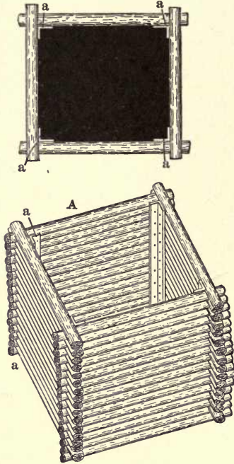
FIGS. 21 AND 21A. — CRIBBED SHAFT TIMBERING WITH POLES.
