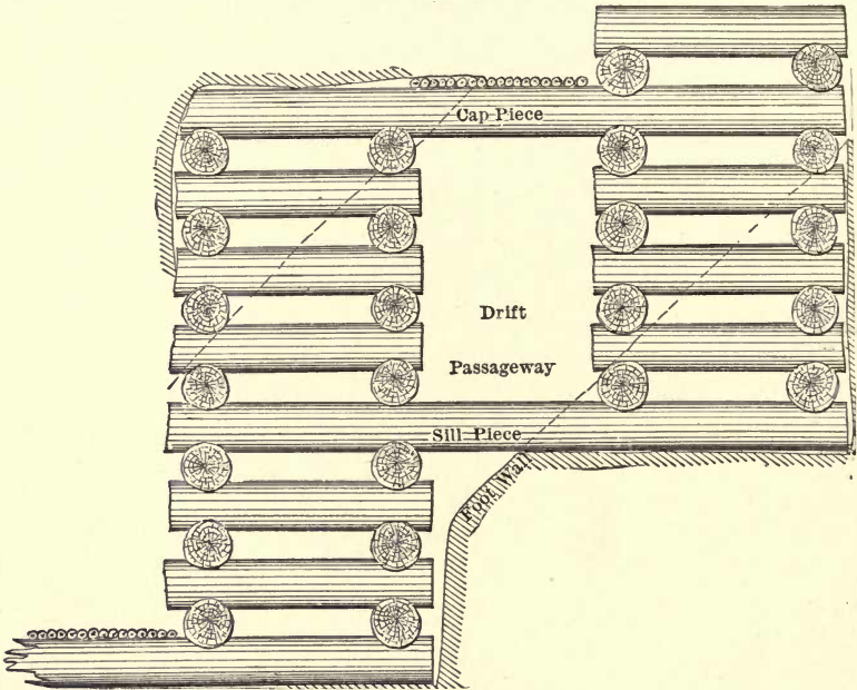
FIG. 49. — PENNING.
