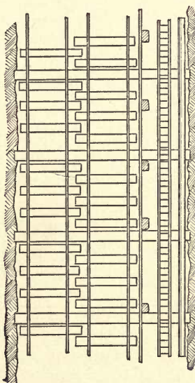
FIG. 107. — SHAFT TIMBERING. Plan and section.
