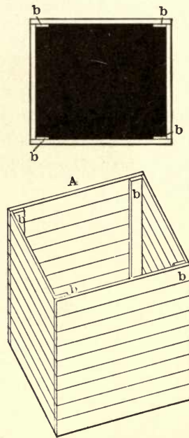
FIGS. 22 AND 22A. — CRIBBED SHAFT TIMBERING WITH PLANKS.
