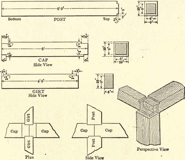
FIG. 106. — DETAILS OF SQUARE-SET TIMBERING.
