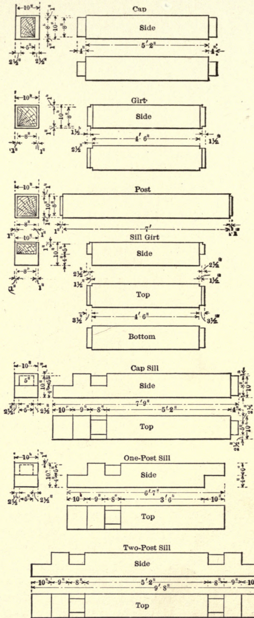
FIG. 56. — ANACONDA METHOD OF FRAMING. Details.
