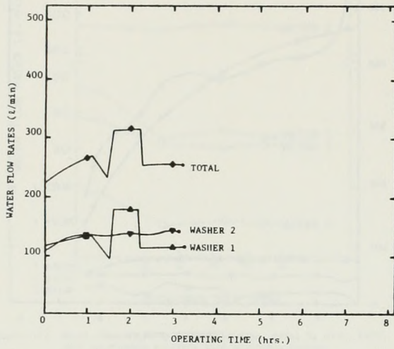
Figure A-9: Water overflow rates from conventional washers vs. operating time, Trial 3, Spring, 1976, when processing spinach on the west line.
