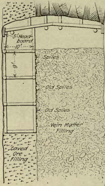
FIG. 32. CROSS SECTION OF CAVED STOPE SHOWING STULL SUPPORT UNDER BACK AND THREE FLOORS OF SPILED DRIFT
