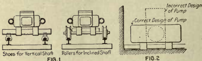
FIG. 47. ARRANGEMENTS FOR PUMPS IN SHAFTS
