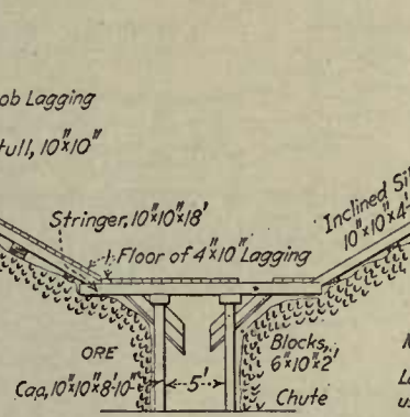
Fig.2 Regular Section Timbers
