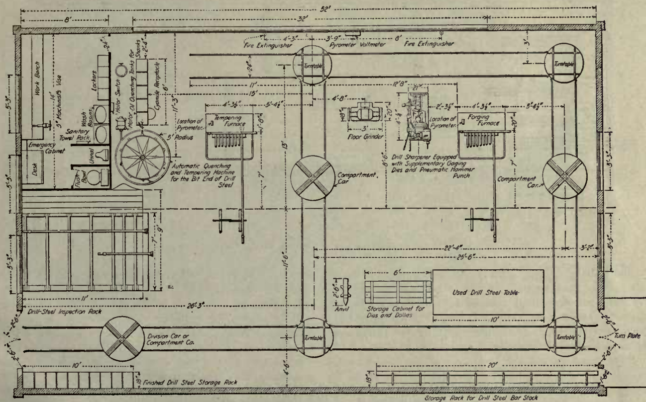
FIG. 49. FLOOR PLAN OF IDEAL SHOP FOR SHARPENING STEEL
