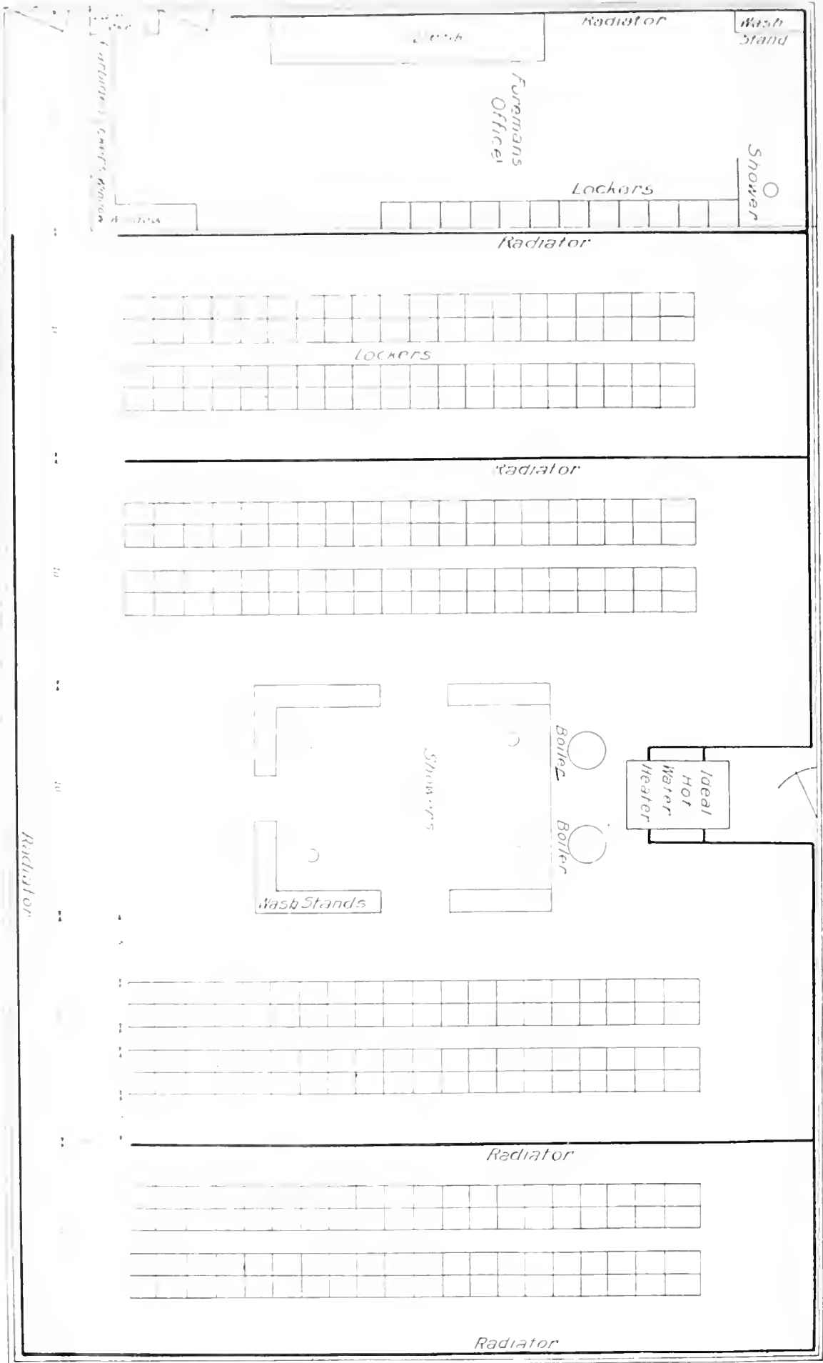
PLAN OF CHAMBER MINE 1000 FT. ST., NAVAJO CITY, ARIZONA.
