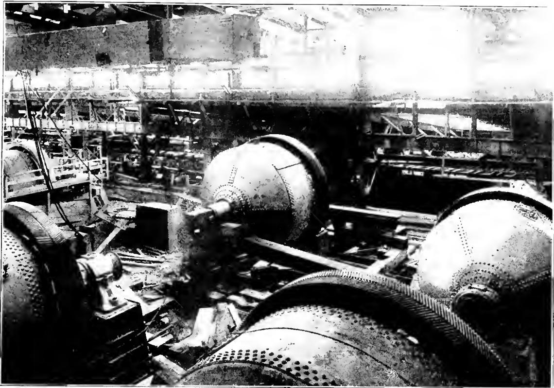
FIG. 6. HARBIDGE MILLS, RE-GRINDING DIVISION.
