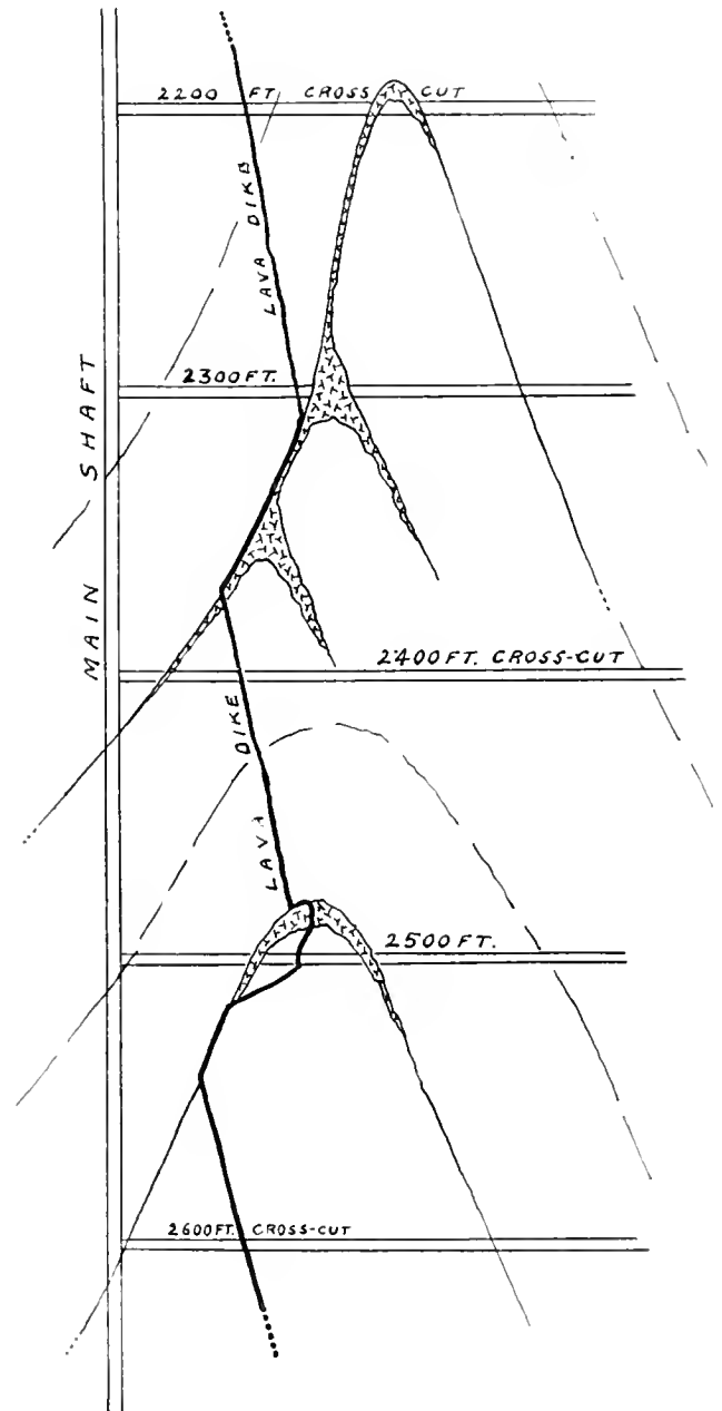
FIG. 2. THE SADDLE-BEELS IN THE 180 MINE, AT BENDIGO.
