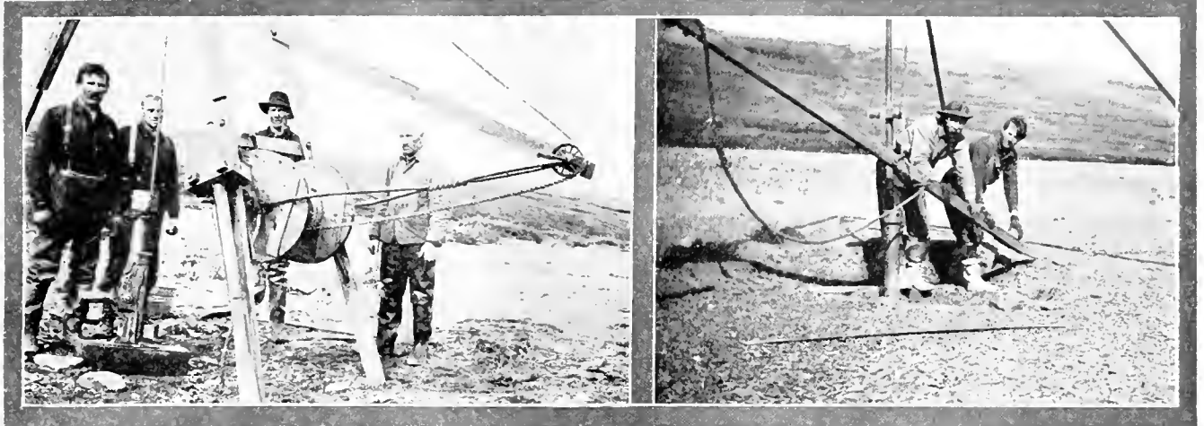
A PLACER-DRILL.
