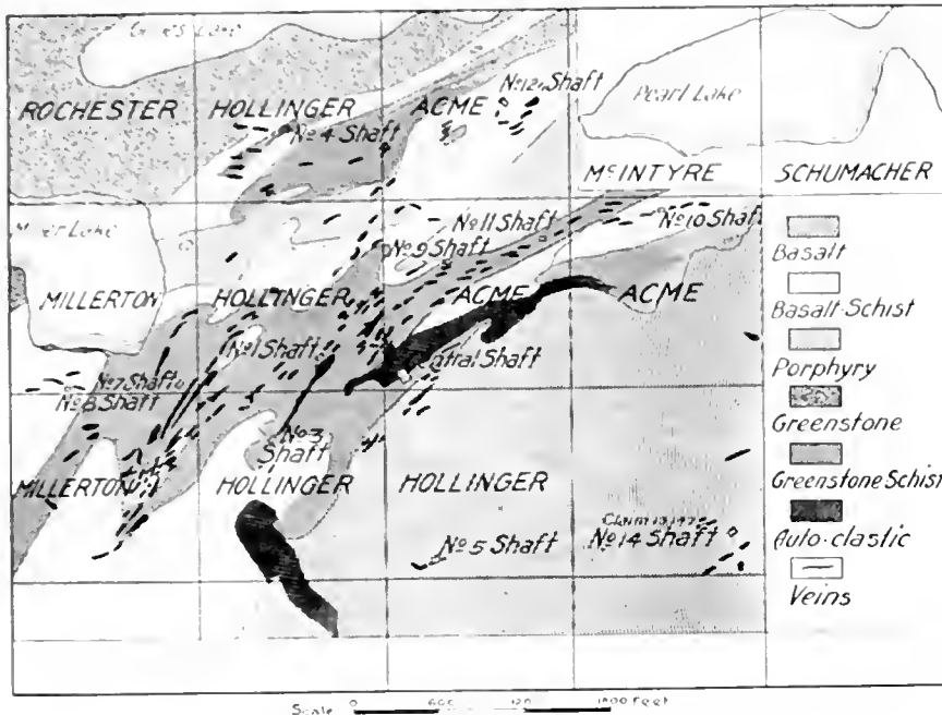
PLAN SHOWING VEIN OUTCROPS AND SURFACE GEOLOGY OF THE NEW CONSOLIDATION AT PORCUPINE, ONTARIO; THE HOLLINGER CONSOLIDATED GOLD MINES, LTD.
