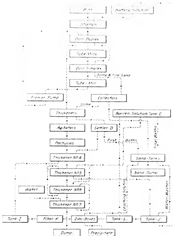
FLOW-SHEET OF COMACARAN MILL.
