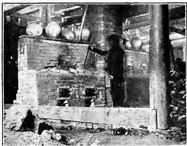
SHOWING OPERATION OF ANTIMONY FURNACES FOR PRODUCING 'CRUDE' METAL IN CHINA.
