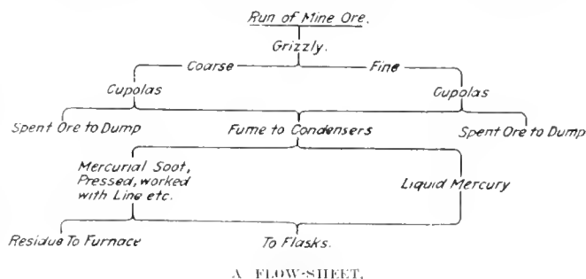
A FLOW-SHEET.
