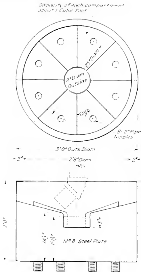
FIG. 5. ROUND-TABLE DISTRIBUTER.
