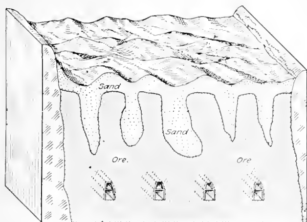
FIG. 1. THE EFFECT OF PROMISCUOUS CAVING.
