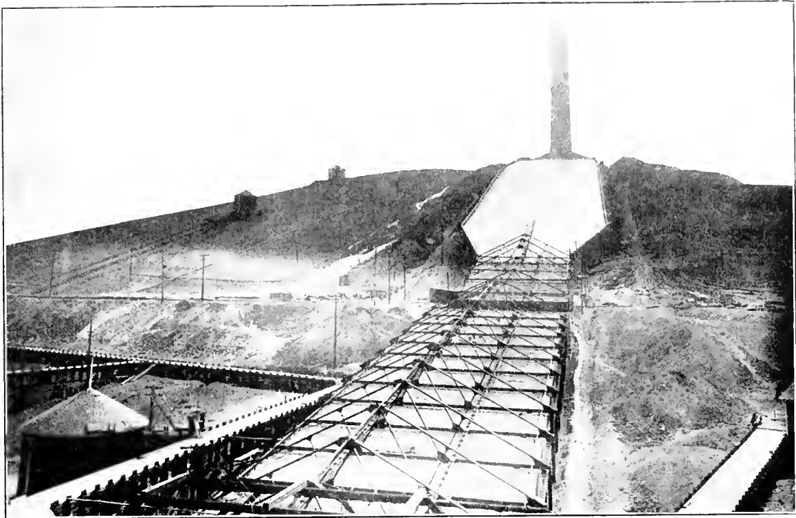
FIG. 2. THE MAIN FLUE AND STACK. THE SINGLE OR 60-FT. FLUE IN THE FOREGROUND HAS A TRUSSED ROOF. THE DOUBLE OR 120-FT. FLUE HAS A PLATE-IRON ROOF. THE STACK IS 30 FT. DIAM. BY 300 FT. HIGH.
