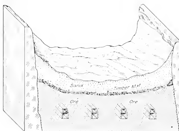
FIG. 2. BLOCK-CAVING CORRECTLY DONE.
