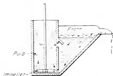
FIG. 10B. ANOTHER FORM OF HOOVER MACHINE.
