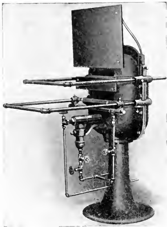
NO. 3 FURNACE FOR DRILL-STEEL.
