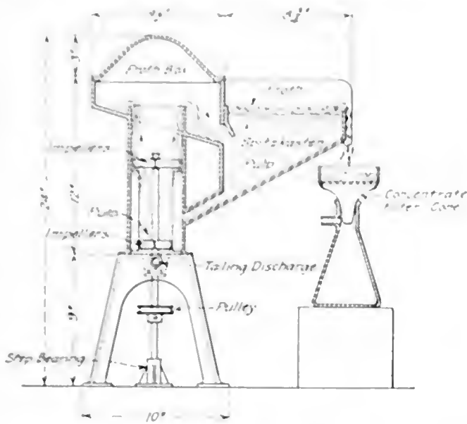
FIG. 7. THE JANNEY TEST MACHINE.
