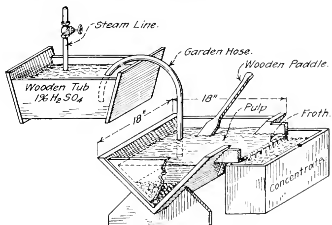
FIG. 4. A POTTER-DELPAT TEST.
