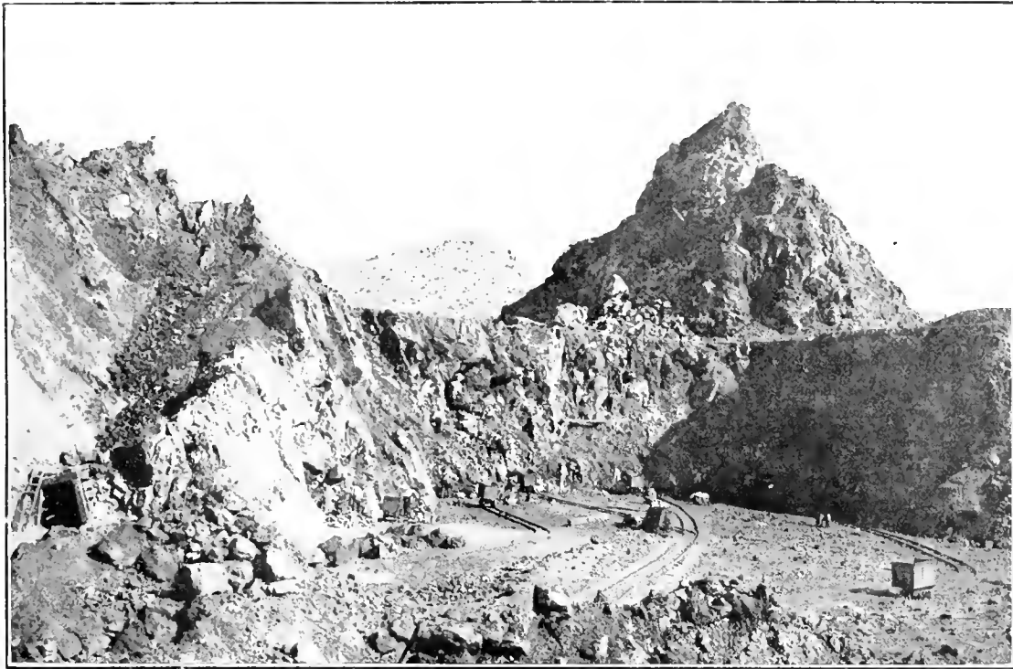
FIG. 3. TYPICAL OUTCROP OF CONTACT METAMORPHIC OREBODY, SHANNON MINE, METCALF, ARIZONA.
