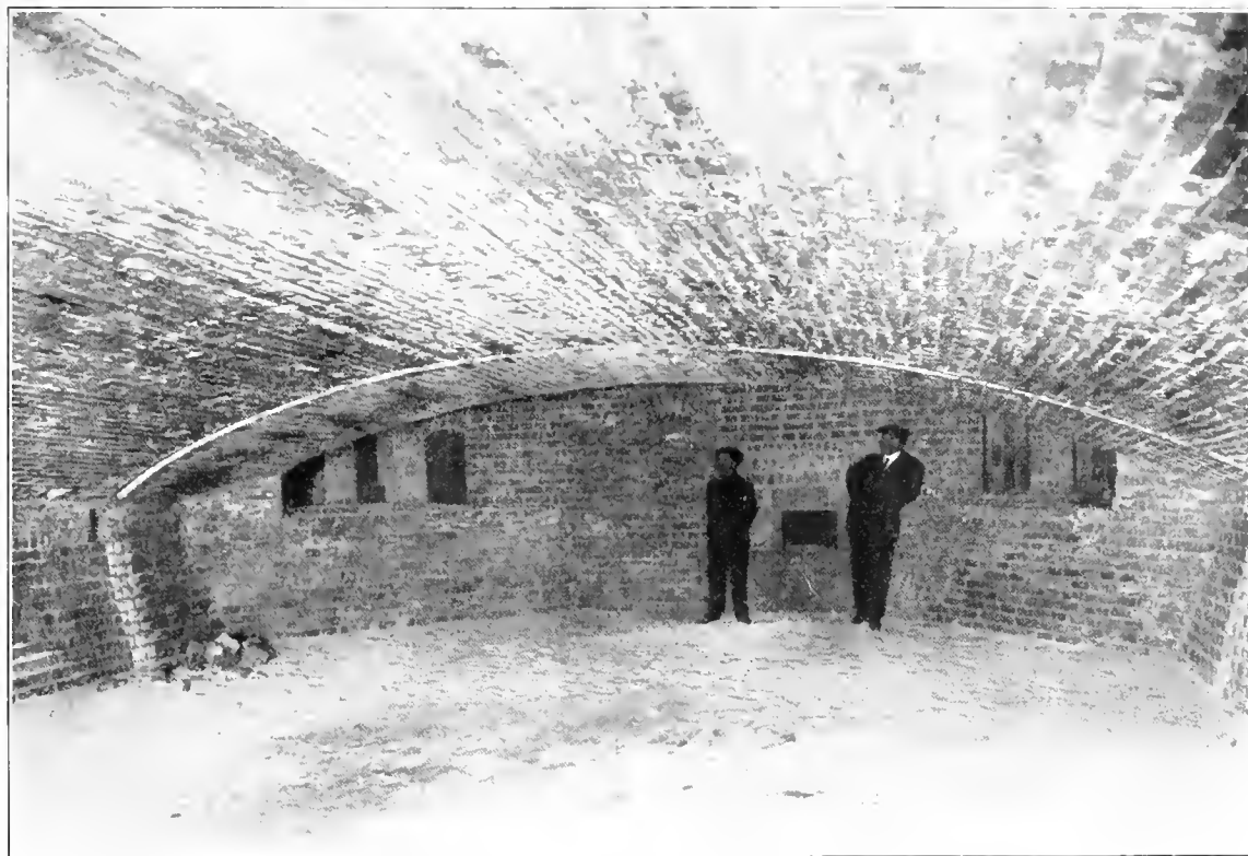
FIG. 5. FRONT END OF NO. 6 REVERBERATORY FURNACE. THE INDEPENDENT VERB ARCH IS SHOWN, SEPARATED BY A 4-INCH JOINT FROM THE REST OF THE ROOF. THIS JOINT CLOSES BY EXPANSION WHEN THE FURNACE IS HOT. BETWEEN THE MEN IS THE SLAG-HOLE OR SKIMMING-HOLE.
