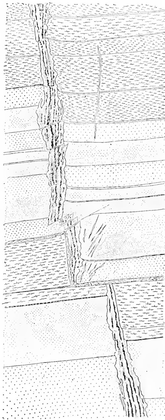
CROSS-SECTION OF THE JUMBO VEIN, IN THE ENTERPRISE MINE, RICO, COLORADO.
