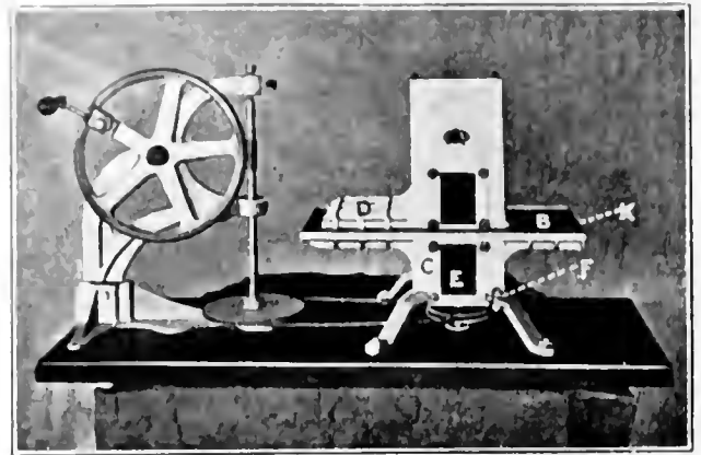
FIG. 11. THE SLIDE MACHINE.
