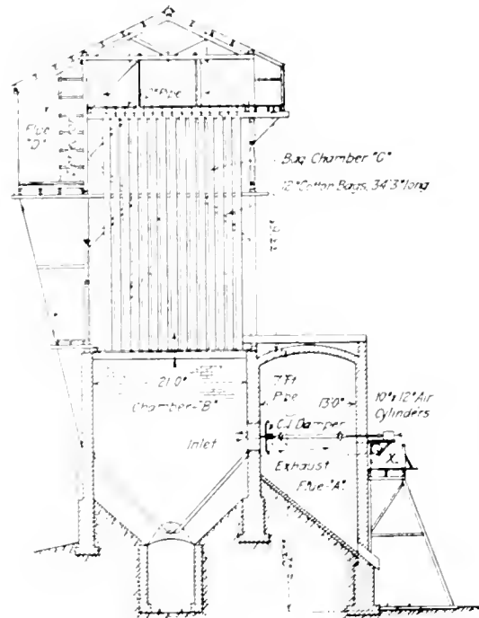
FIG. 3. SHOWING POSITION OF INLET-DAMPER AND AIR-FEEDER.
