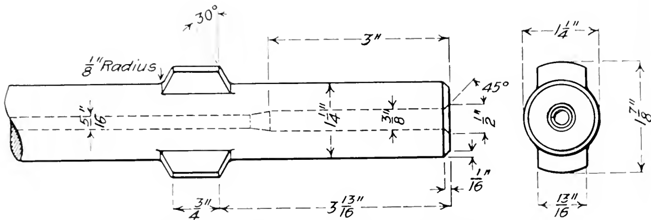
FIG. 1. A DRILL-SHANK ON ROUND STEEL FOR MOUNTED HAMMER-DRILLS. NOTE THE TWO LUGS.
