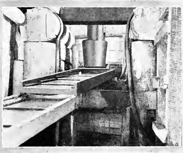
A CLOSE VIEW OF THE MORTAR-BOX.
