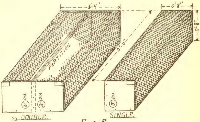
Fig. 5. SHIPPING BOXES.
