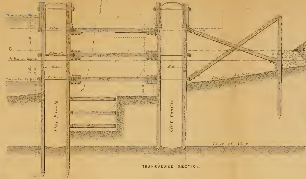
DAMS NOS 1 & 2.
