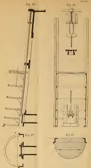
OUTLET SLUICE FOR TOWN PIPE WITH SCREEN.
