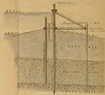
ENLARGED SECTION OF OUTER COFFER DAM.
