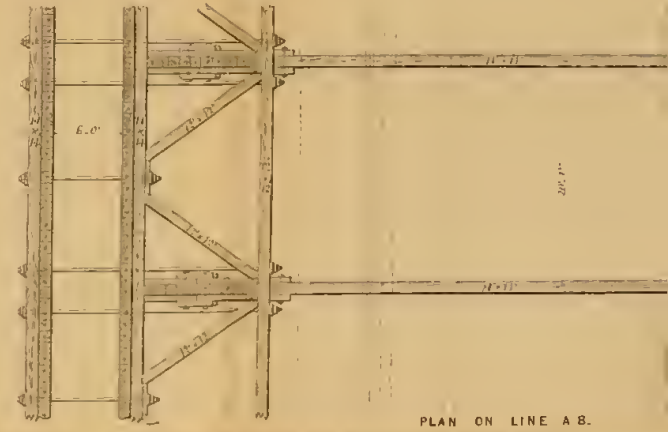
PLAN ON LINE A. B.
