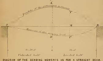
DIAGRAM OF THE BENDING MOMENTS AS FOR A STRAIGHT BEAM.
