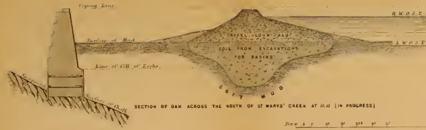
Fig 1. CHATHAM DOCKYARD EXTENSION.
