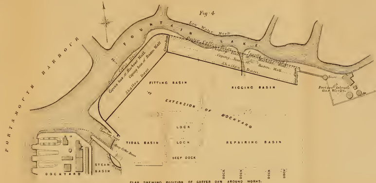
PLAN SHEWING POSITION OF COFFER DAM AROUND WORKS.
