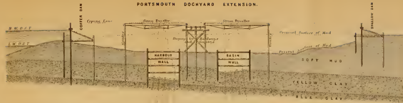
SECTION THROUGH COFFER DAM AROUND WORKS, AT B.B.
