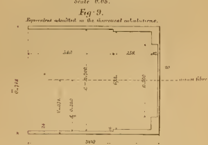
SECTION AT THE SUMMIT. Scale 0.05.
