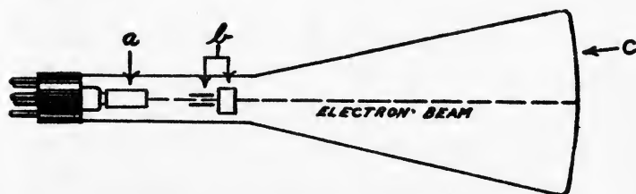
The cathode-ray tube is composed of three principal parts: (a) the electron gun; (b) the horizontal and vertical deflecting plates; (c) the willemite picture screen.
