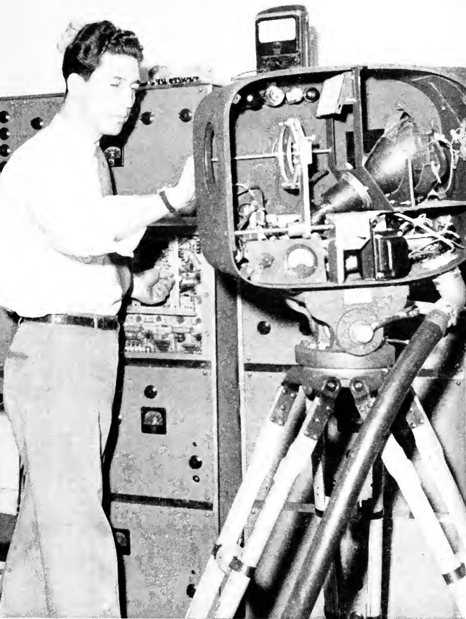
We see here a television camera with the side removed so that we can learn a little about the maze of wires and strange tubes and lenses which make up its working parts. The large conduit leading from the front of the camera is a coaxial cable.
