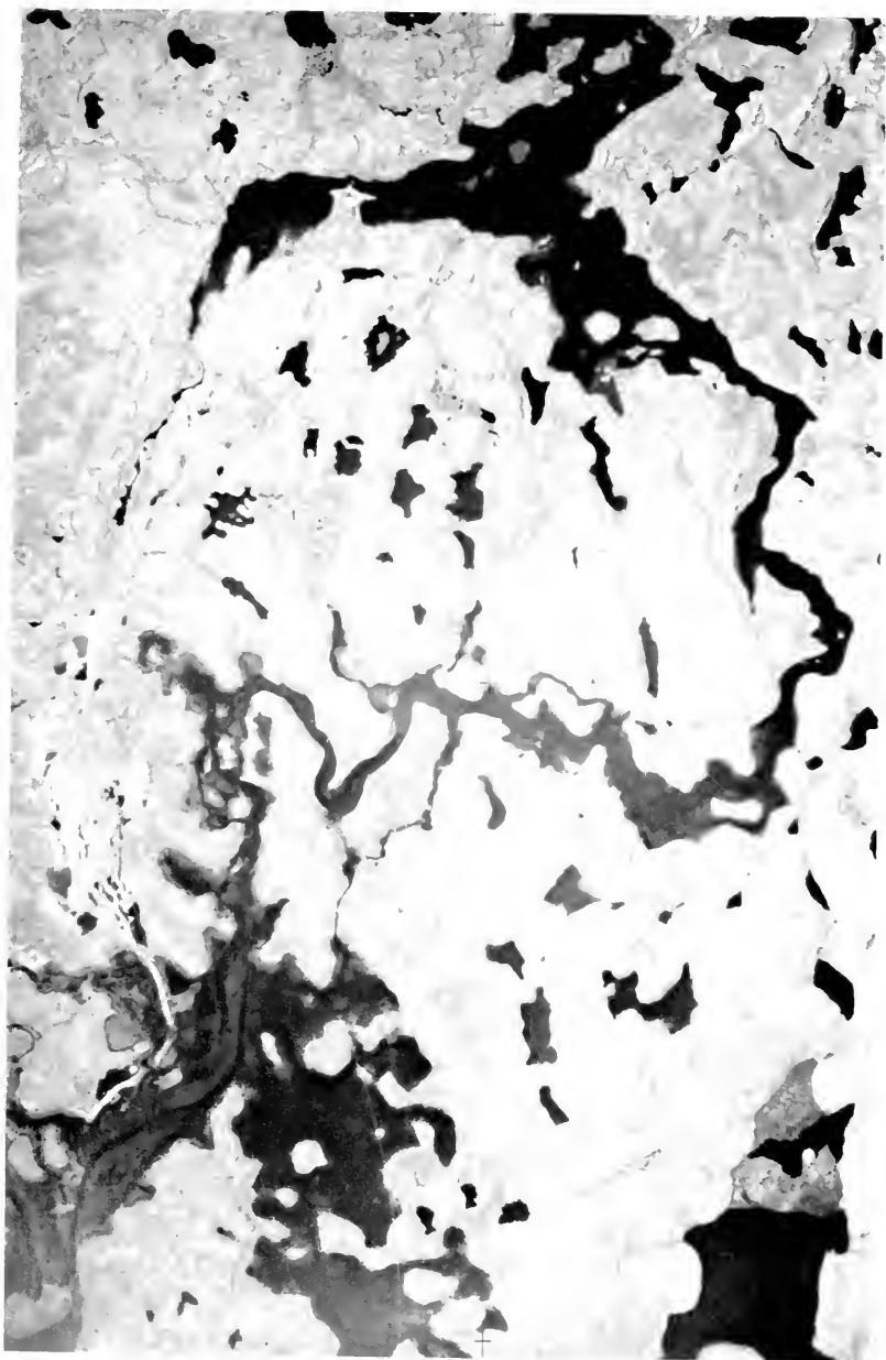
Eskimo country along the upper Kazan River at approximately lat. 61° 22' N., long. 100° 36' W. The area shown is about 5 × 3.2 miles in extent. A vertical photograph from an altitude of 18,000 feet above sea level, July 5, 1949. (Courtesy of Royal Canadian Air Force.)
