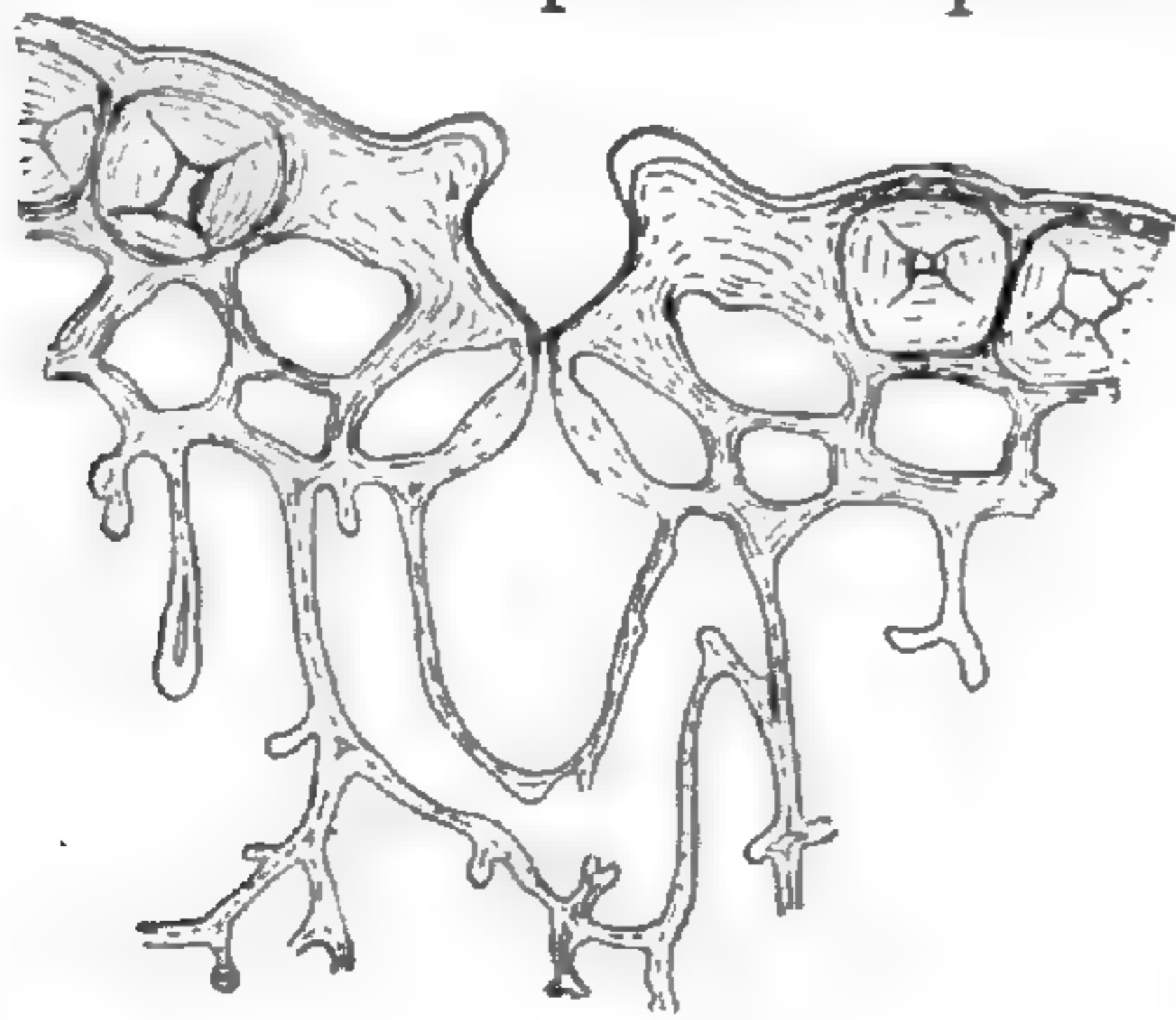
Fig. 8. Section of stoma of Pinus sylvestris X 650.
