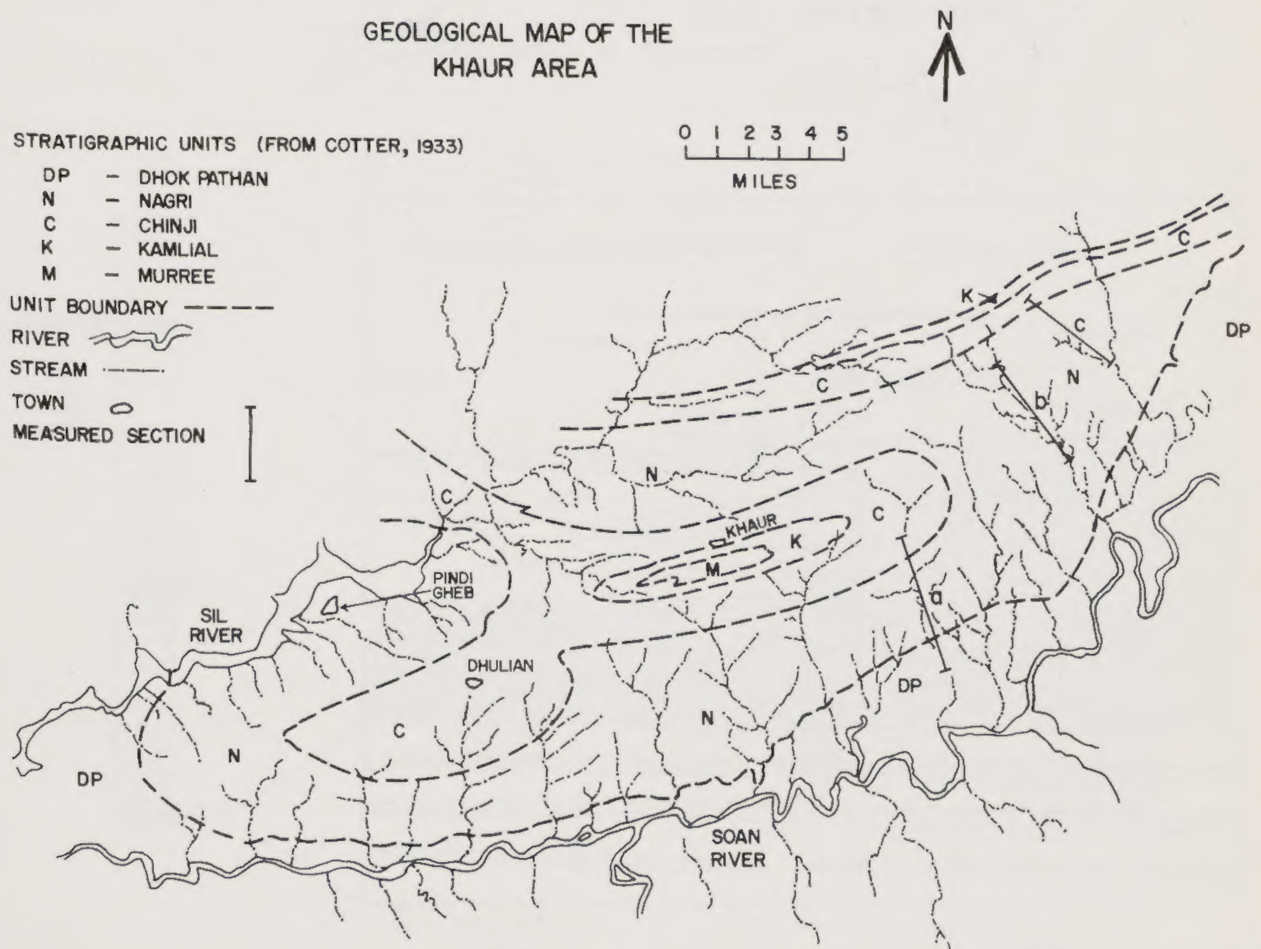
Fig. 3 Map of Dhok Pathan-Khaur-Kaulial area (A of Fig. 2) showing lithological units according to Cotter (1933) and location of measured sections.
