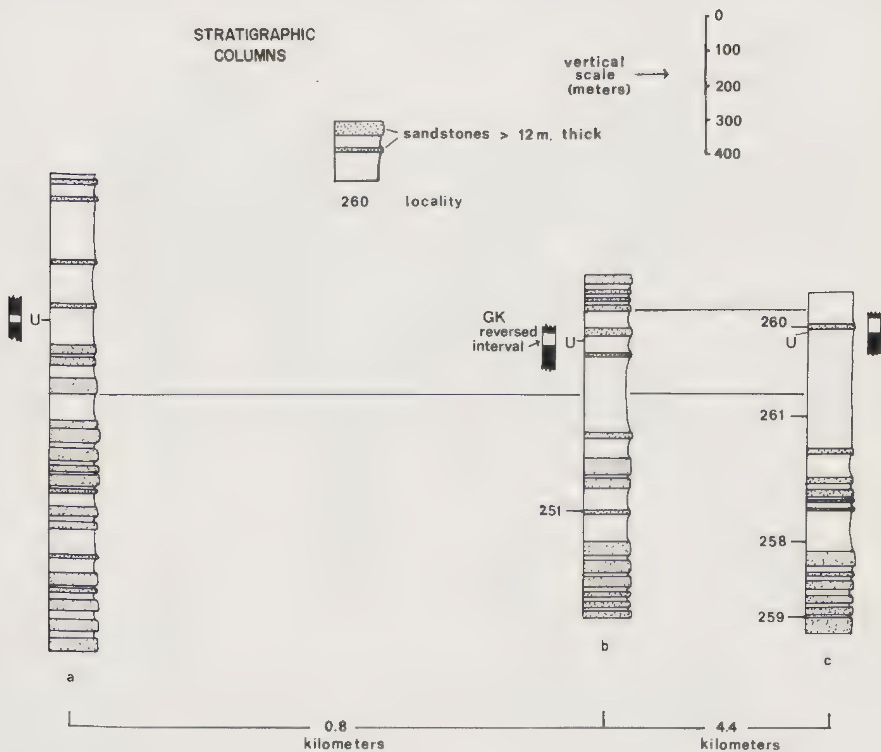
Fig. 5 Simplified measured sections corresponding to locations given in Figure 3. The position of the "U" sandstone, Ganda Kas reversed intervals, and representative fossil localities are shown. Solid lines connecting the columns are lithologically continuous horizons walked out between sections. Only sands thicker than 12 m are shown; thinner sands occur throughout the columns (i.e., "U").
