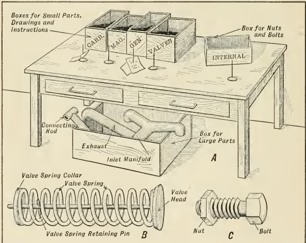
Fig. 67.—Showing Method of Providing Boxes for Keeping Parts Together in Overhauling Cars Systematically.
