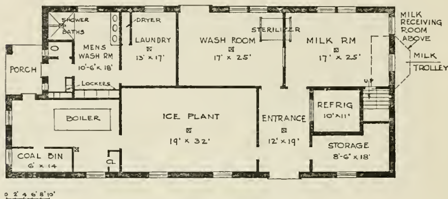
FIG. 28—PLAN OF DAIRY AT CEDARHURST, L. I.
