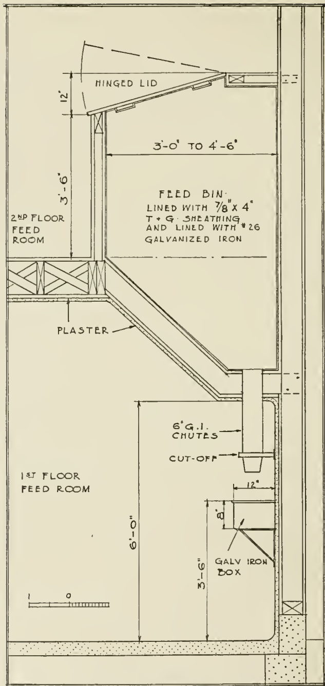
FIG. 2—SECTION OF FEED BIN [24]
