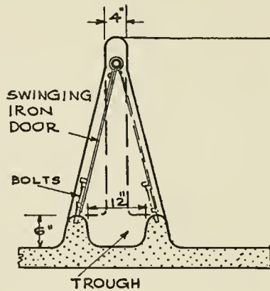
FIG. 74—SECTION THROUGH FEEDING TROUGHS
