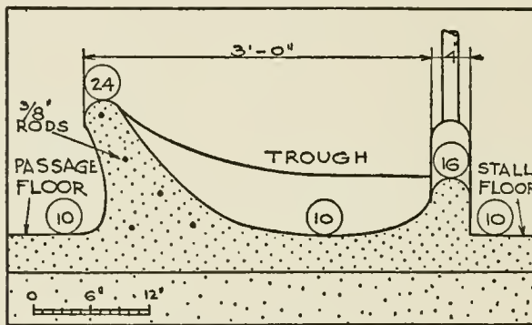
FIG. 11—FEED TROUGH WITH FRONT EDGE 14 IN. ABOVE THE FLOOR SO THAT THE FEED MAY BE RETAINED WITHIN THE TROUGH
