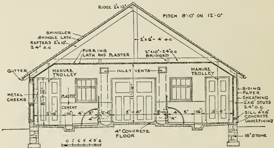
FIG. 6.—SECTION THROUGH A COW BARN 36 FT. WIDE
