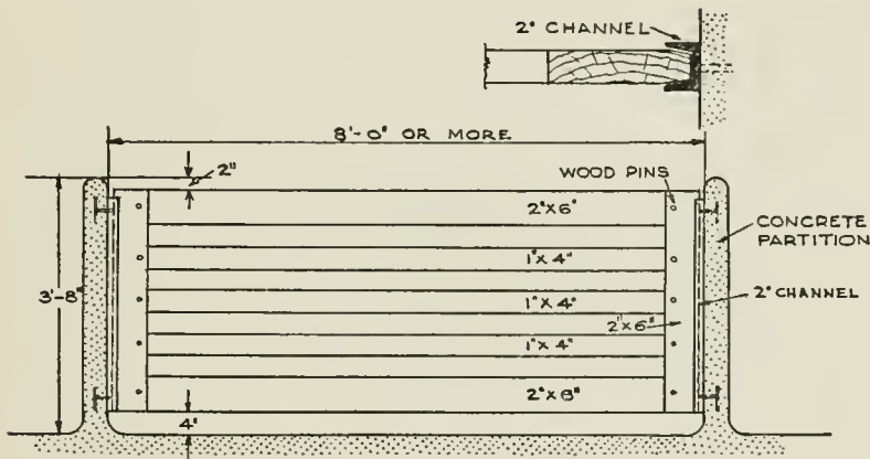
FIG. 8.—DETAIL OF MOVABLE CALF PEN PARTITION
