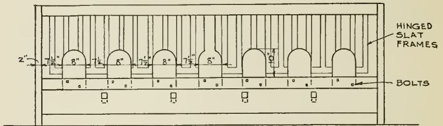
SIDE ELEVATION
