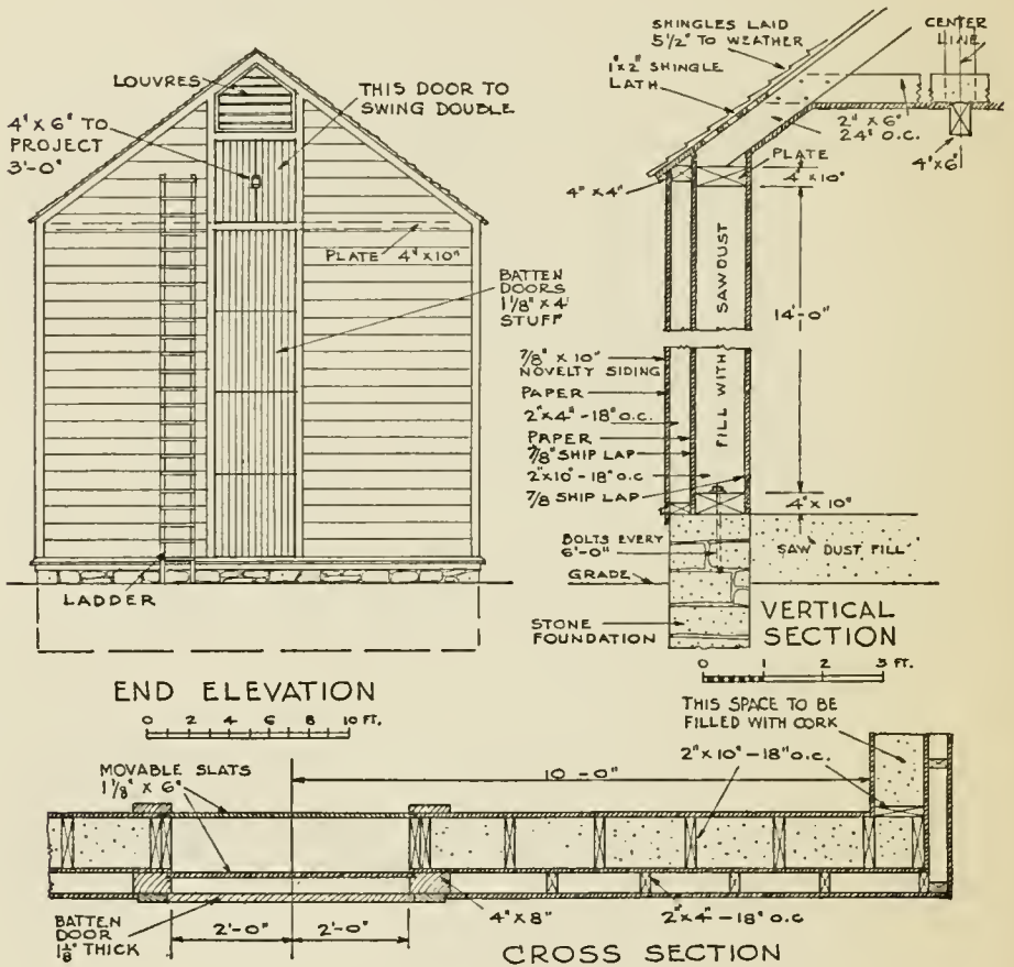
FIG 77.—ELEVATION AND DETAIL OF ICE HOUSE
