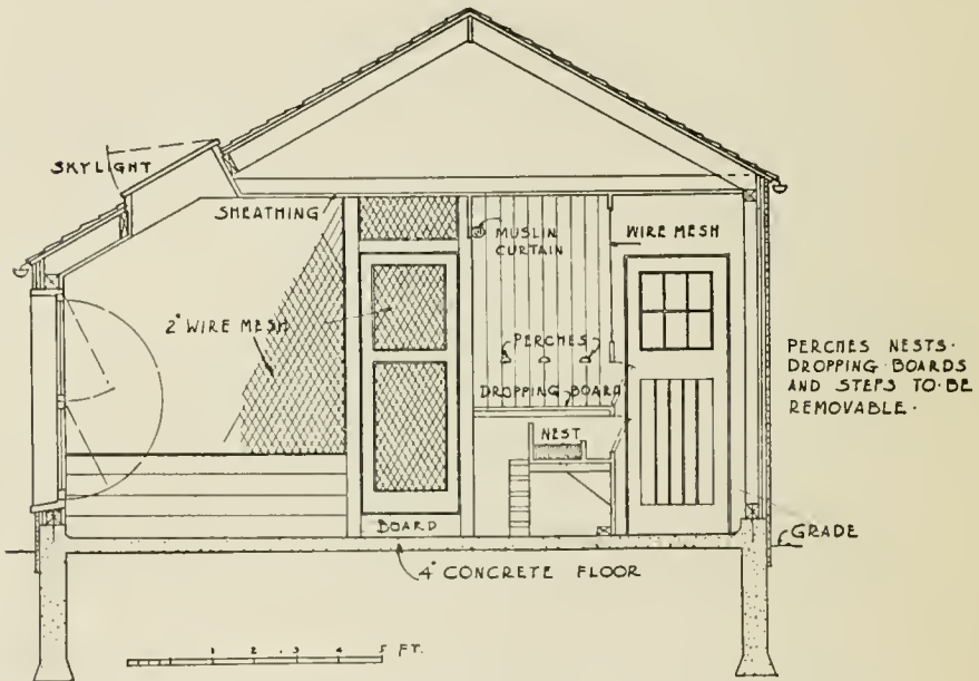
FIG. 66—SECTION THROUGH CHICKEN HOUSE SHOWING NESTS, ETC.
