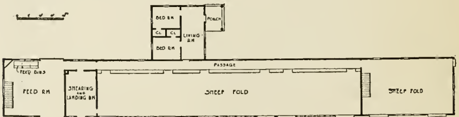
FIG. 71—PLAN OF SHEEPFOLD AT STERLINGTON, N. Y., FOR FRANCIS LYNDE STETSON, ESQ.
