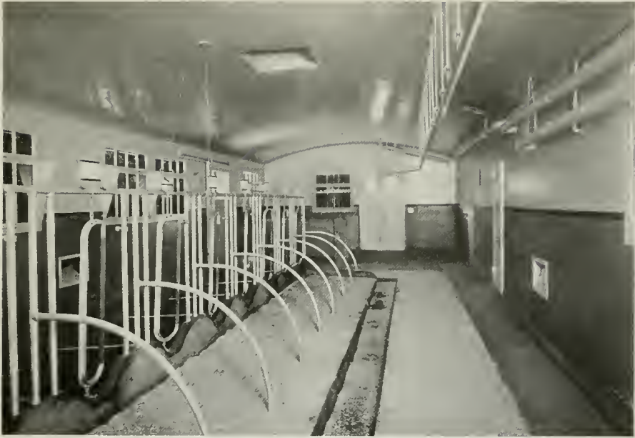
CONTINUOUS FEEDING-TROUGH, DIVIDED BY RODS ONLY
