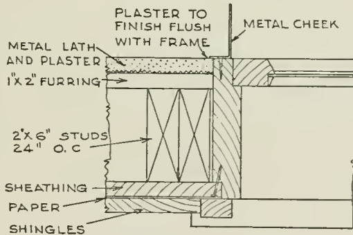
CROSS SECTION AT JAMB
