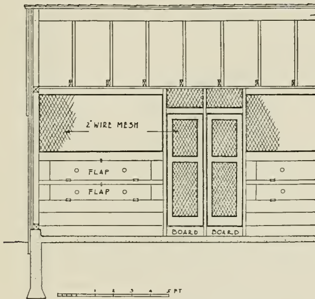
FIG. 65—ELEVATION OF PEN IN PASSAGEWAY
