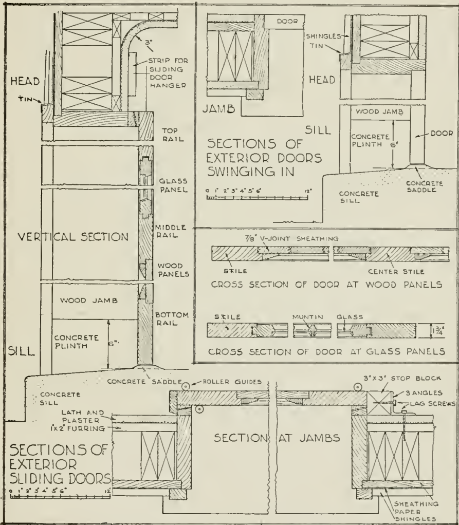
FIG. 20—DETAIL OF THE DOORS FOR THE COW BARN
