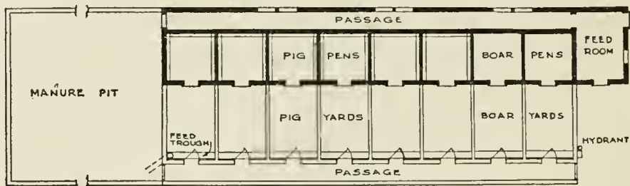
FIG. 75—PLAN OF PIGGERY AT ISLIP, L. I.
