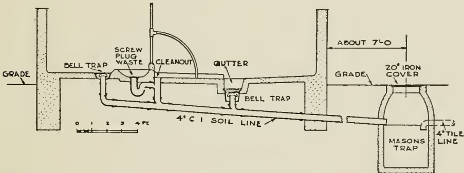
FIG. 15—SECTION THROUGH TROUGH, SHOWING SOIL LINE AND CLEAN-OUT PIT OR MASON'S TRAP
