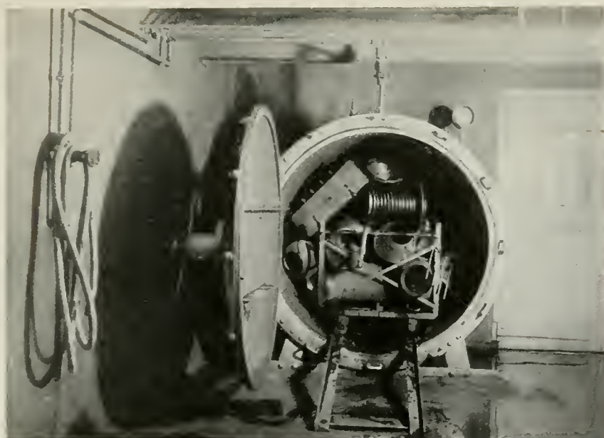
HIGH-PRESSURE STERILIZER FILLED WITH DAIRY UTENSILS READY FOR STERILIZING
