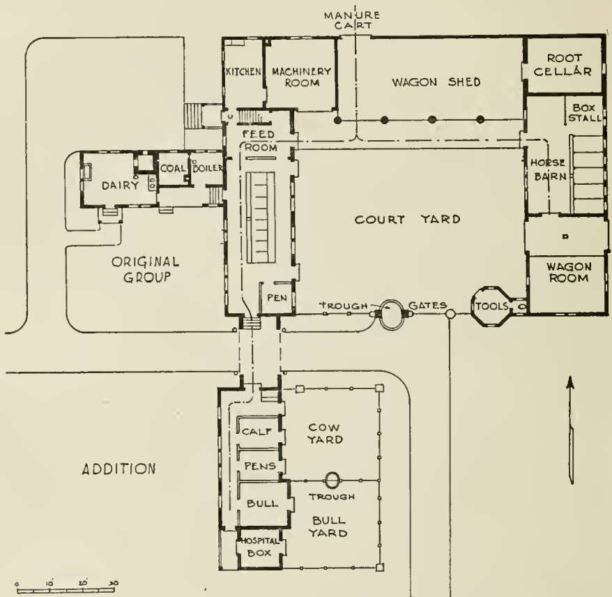
FIG. 46—PLAN OF FARM BUILDINGS AT OYSTER BAY, L. I., FOR MORTIMER L. SCHIFF, ESQ.
