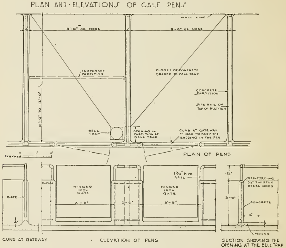
FIG. 9—DETAIL OF CALF PENS
