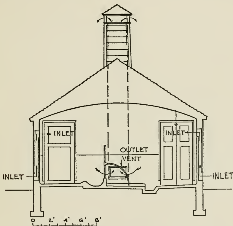
FIG. 16—OUTLET VENT DUCT AT END OF BARN RUNNING FROM FLOOR DIRECT THROUGH ROOF
