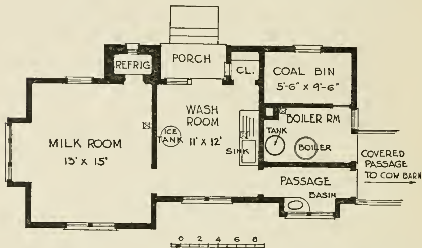
FIG. 26—PLAN OF SMALL DAIRY AT ROSLYN, L. I., FOR BENJAMIN STERN, ESQ.
