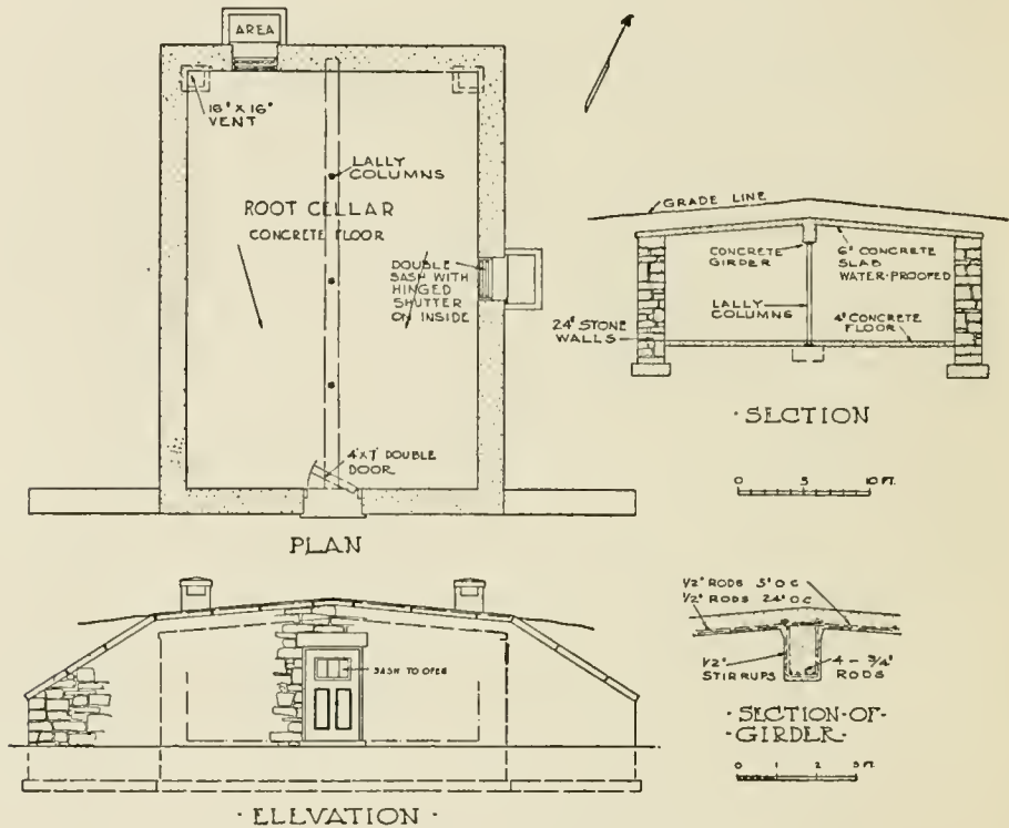
FIG. 76—PLAN OF ROOT CELLAR
