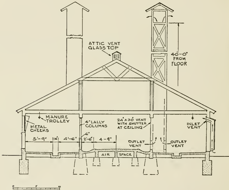
Robert W. Gardner, Architect FIG. 50—SECTION THROUGH THE BRIARCLIFF BARN
