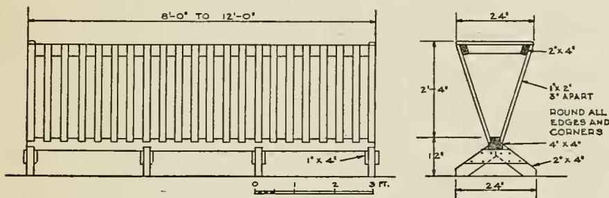
FIG. 69—DETAIL OF USUAL TYPE OF FEEDING RACKS
