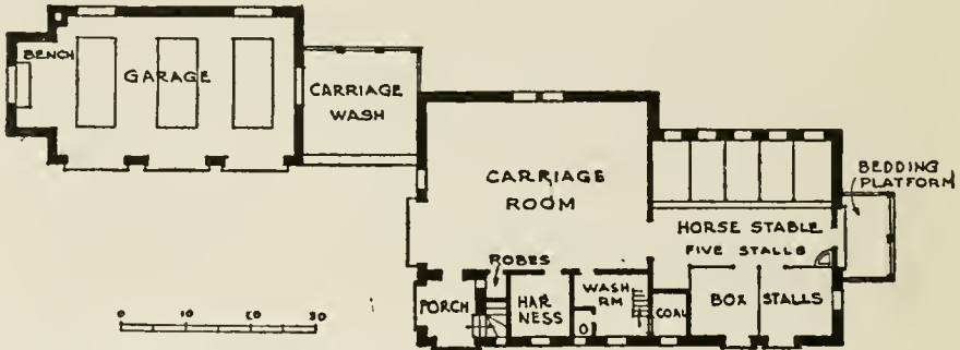
FIG. 56—PLAN OF GARAGE AND STABLE AT ARMONK, N. Y., FOR C. R. AGNEW, ESQ.
