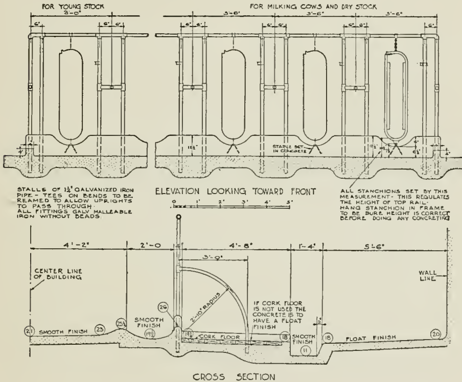
FIG. 7.—DETAIL OF COW STALLS AND STANCHIONS. SEE ALSO PHOTOGRAPH FACING PAGE 32
