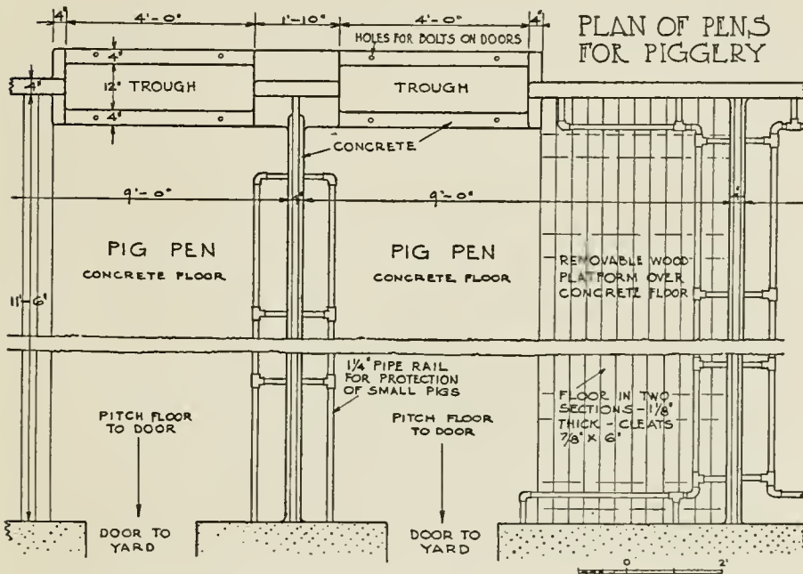
FIG. 73—DETAIL OF PEN FLOOR SHOWING PIPING IN FARROWING PENS
