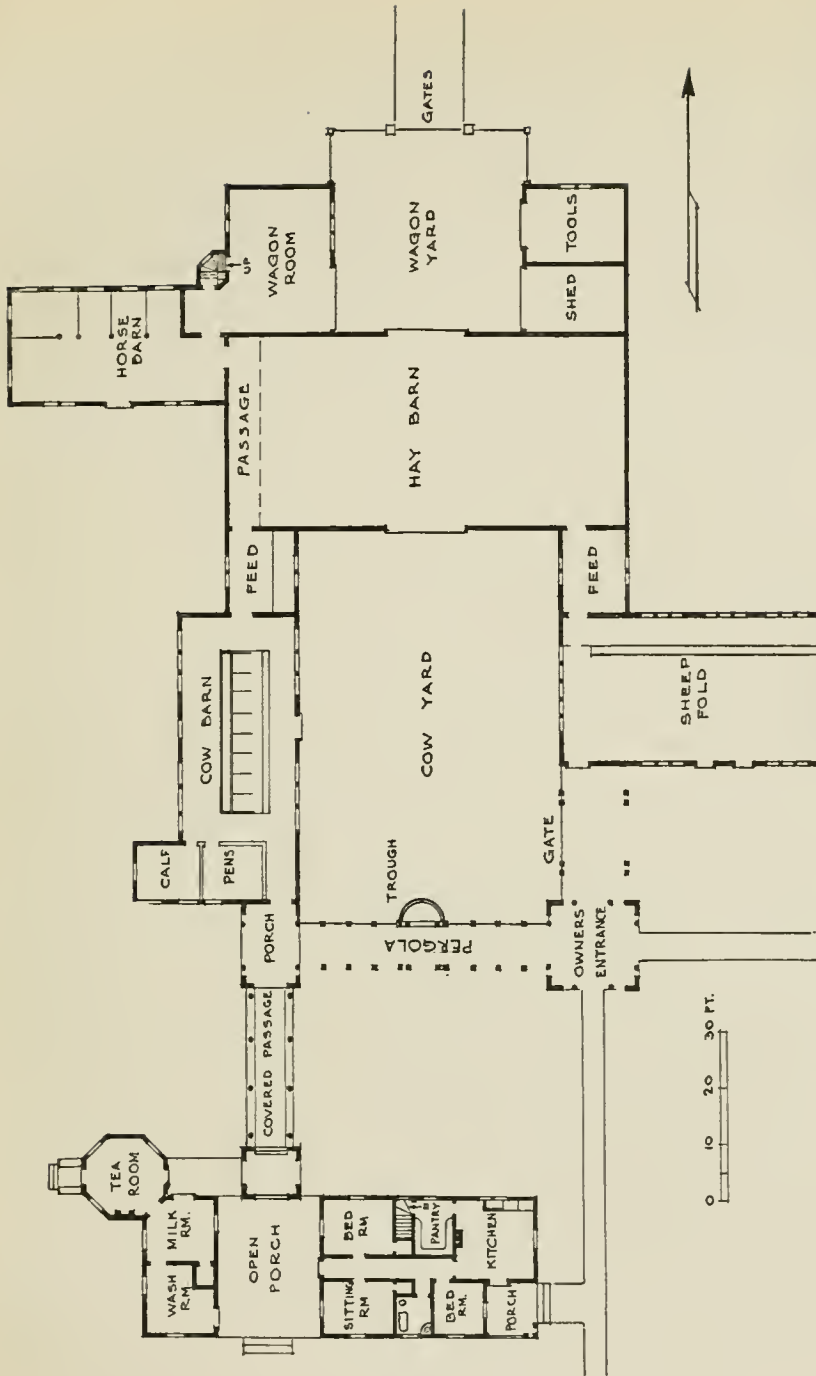
FIG. 38—PLAN OF FARM BUILDINGS AT SCARBORO, N. Y., FOR JAMES SPEYER, ESQ. Alfred Hopkins, Architect
