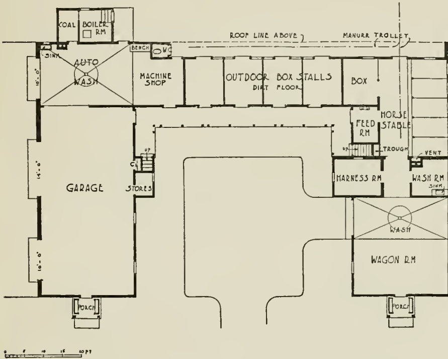
FIG. 57—PLAN OF STABLE AND GARAGE AT ISLIP, L. I., FOR J. HENRY DICK, ESQ.
