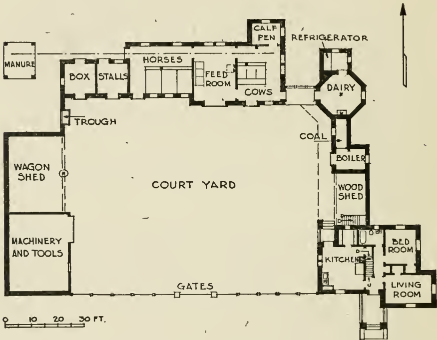
FIG. 44—PLAN OF FARM BUILDINGS AT WOODBURY FALLS, N. Y., FOR CHARLES E. RUSHMORE, ESQ.
