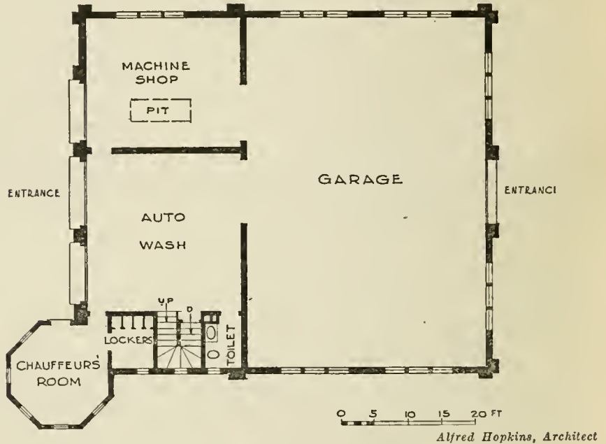
FIG. 58—PLAN OF GARAGE AT ISLIP, L. I., FOR S. T. PETERS, ESQ.
