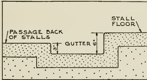
FIG. 12—SHOWING GUTTER WITH LOW SIDE AT PASSAGEWAY. THIS IS UNDESIRABLE
