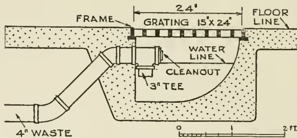
FIG. 61—DETAIL OF SAND TRAP FOR THE AUTOMOBILE WASH OR CARRIAGE WASH
