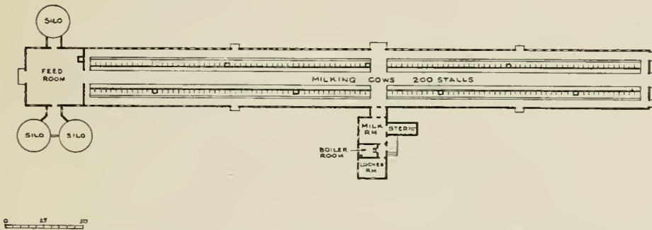
FIG. 49—PLAN OF THE BRIARCLIFF COW BARN, PINE PLAINS, DUCHESS CO., N. Y.
