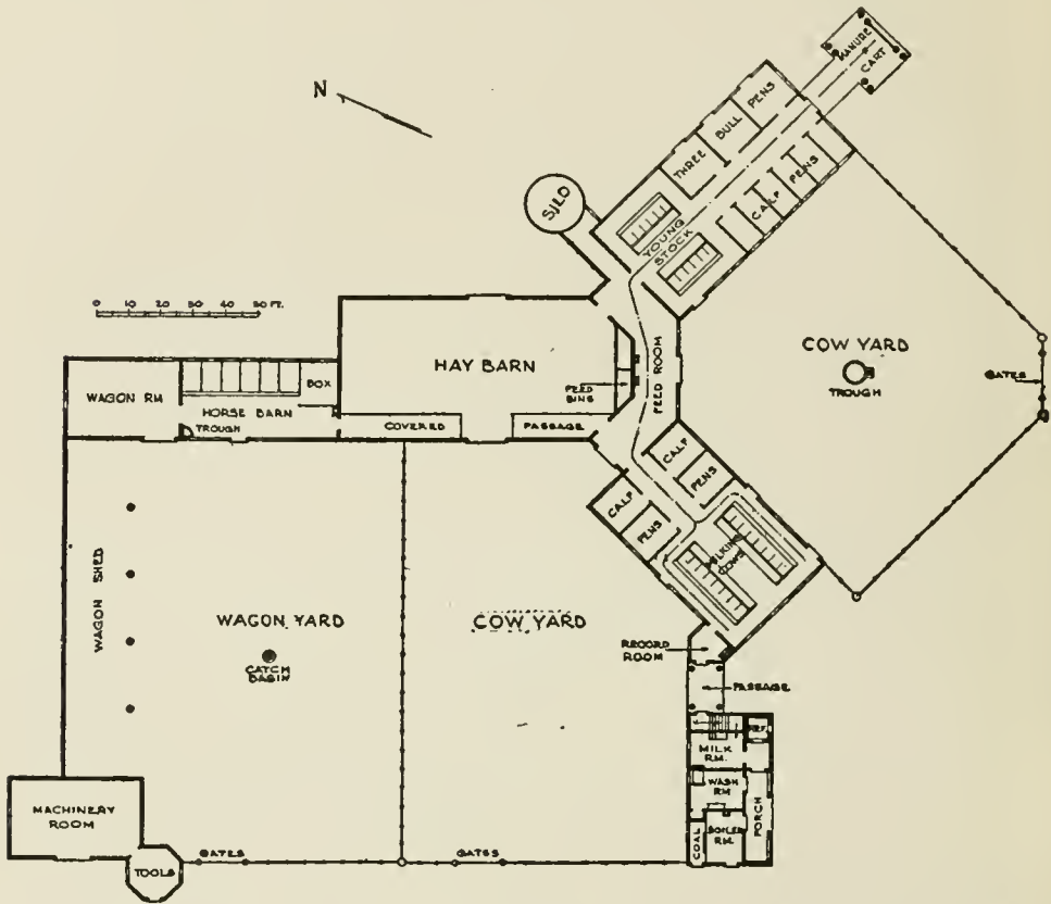
FIG. 47—PLAN OF FARM BUILDINGS AT NORTH EASTON, MASS., FOR F. LOTHROP AMES, ESQ.
