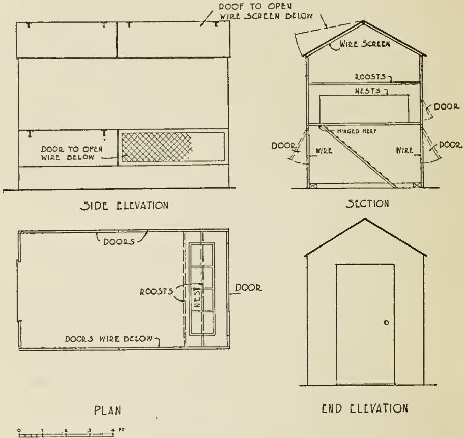
FIG. 62—PLAN OF COLONY HOUSE USED AT SKYLANDS FARM, STERLINGTON, N. Y.
