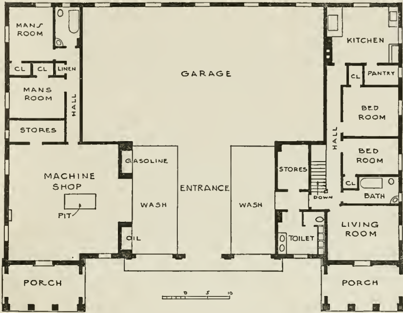
FIG. 60—PLAN OF GARAGE AT GLEN COVE, L. I., FOR CLIFFORD V. BROKAW, ESQ.
