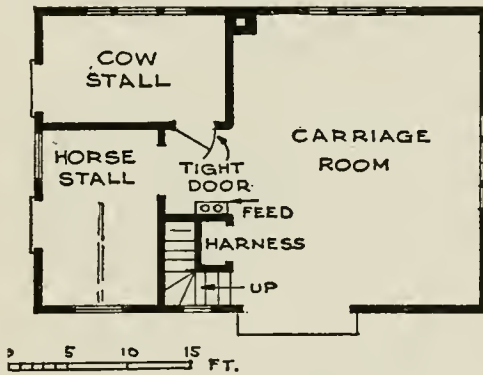
O. S. Keefe, Architect FIG. 52—PLAN OF SMALL STABLE FOR HORSE AND COW
