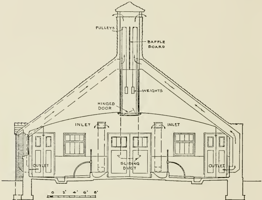
FIG. 17—OUTLET DUCTS IN SIDE WALLS RUN UP THE RAKE OF THE ROOF INTO A CENTRAL VENTILATOR
