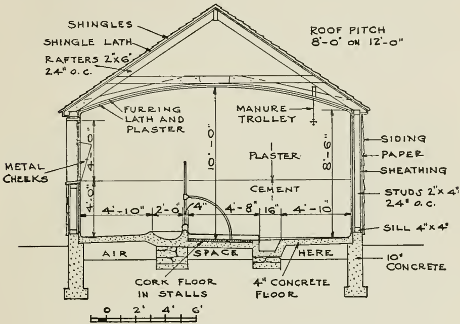
FIG. 5.—SECTION THROUGH A COW BARN 18 FT. WIDE
