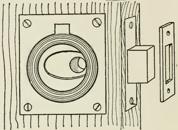
FIG. 34—FLUSH RING AND LOCK
