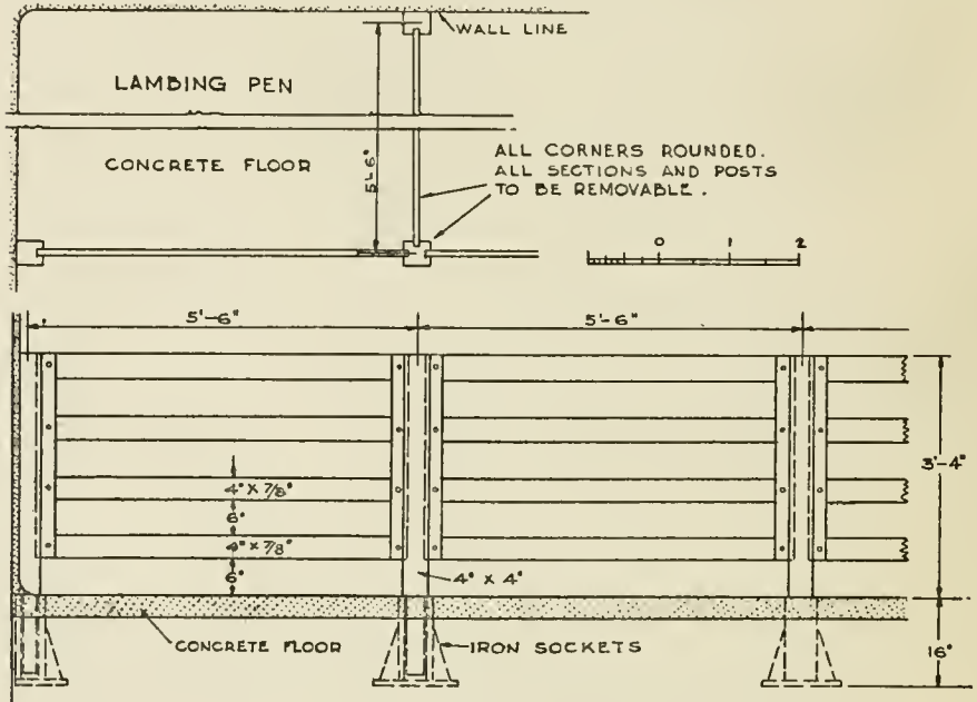
FIG. 70—DETAIL SHOWING REMOVABLE LAMBING PEN PARTITIONS
