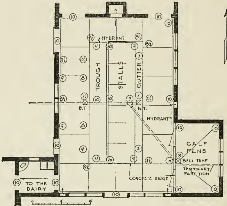
FIG. 13—PLAN SHOWING FLOOR DRAINAGE OF A COW BARN AT GLEN COVE, L. I., FOR CLIFFORD V. BROKAW, ESQ.
