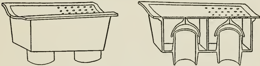
FIG. 14—SPECIAL GUTTER TRAP WITH TWO OUTLETS—ONE TO LIQUID MANURE RECEPTACLE, THE OTHER TO THE SEWAGE DISPOSAL SYSTEM
