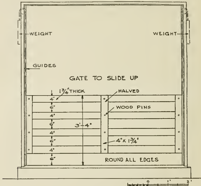
FIG. 67—DETAIL OF SLIDING GATE IN SHEEP PEN DOOR
