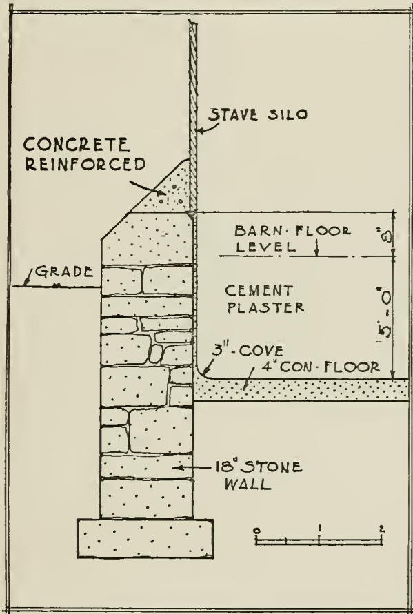
FIG. 18—SECTION THROUGH SILO FOUNDATION
