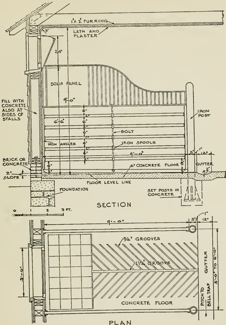
FIG. 32—DETAIL OF THE "BURNETT" STALL—THE BEST TYPE OF THE RIGID STALL PARTITION
