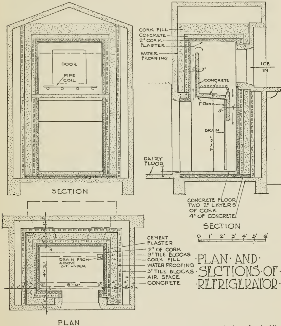
FIG. 24—DETAIL OF CONCRETE REFRIGERATOR
