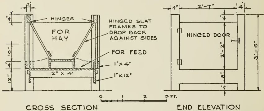
FIG. 68.—DETAIL OF SHEEP FEEDING-RACK RECOMMENDED AS MOST ECONOMICAL OF FEED
