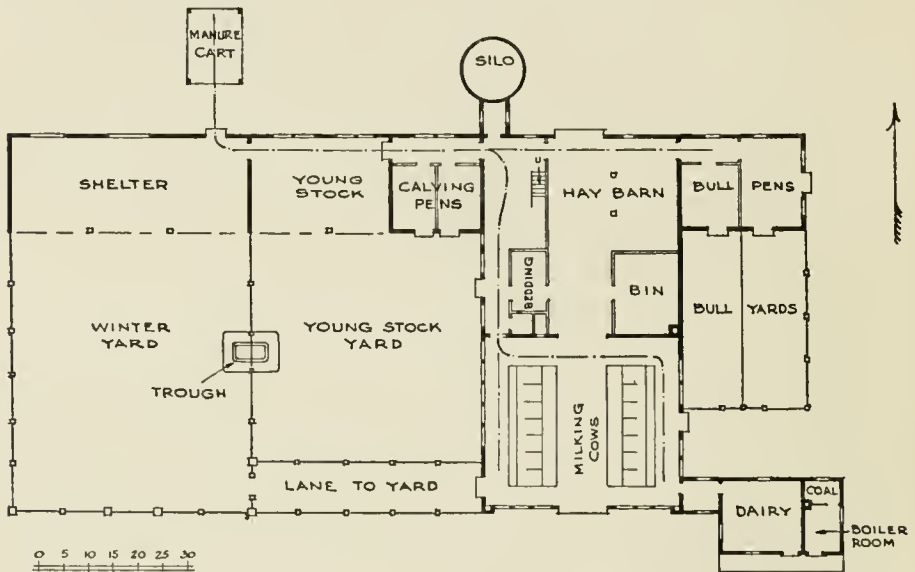
FIG. 19.—PLAN OF FARM BUILDINGS AT FRAMINGHAM, MASS., FOR N. I. BOWDITCH, ESQ.
