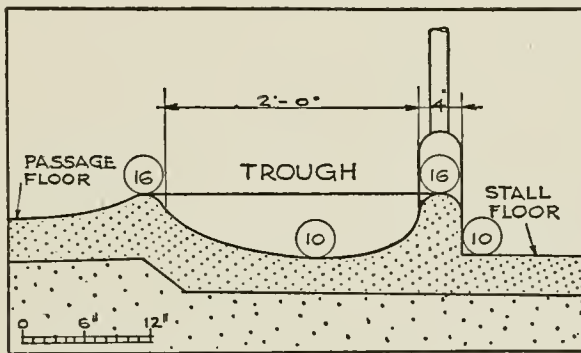
FIG. 10.—FEEDING-TROUGH WITH FRONT EDGE LEVEL WITH THE FLOOR SO THAT FEED PUSHED OUT MAY BE READILY SWEEPED BACK
