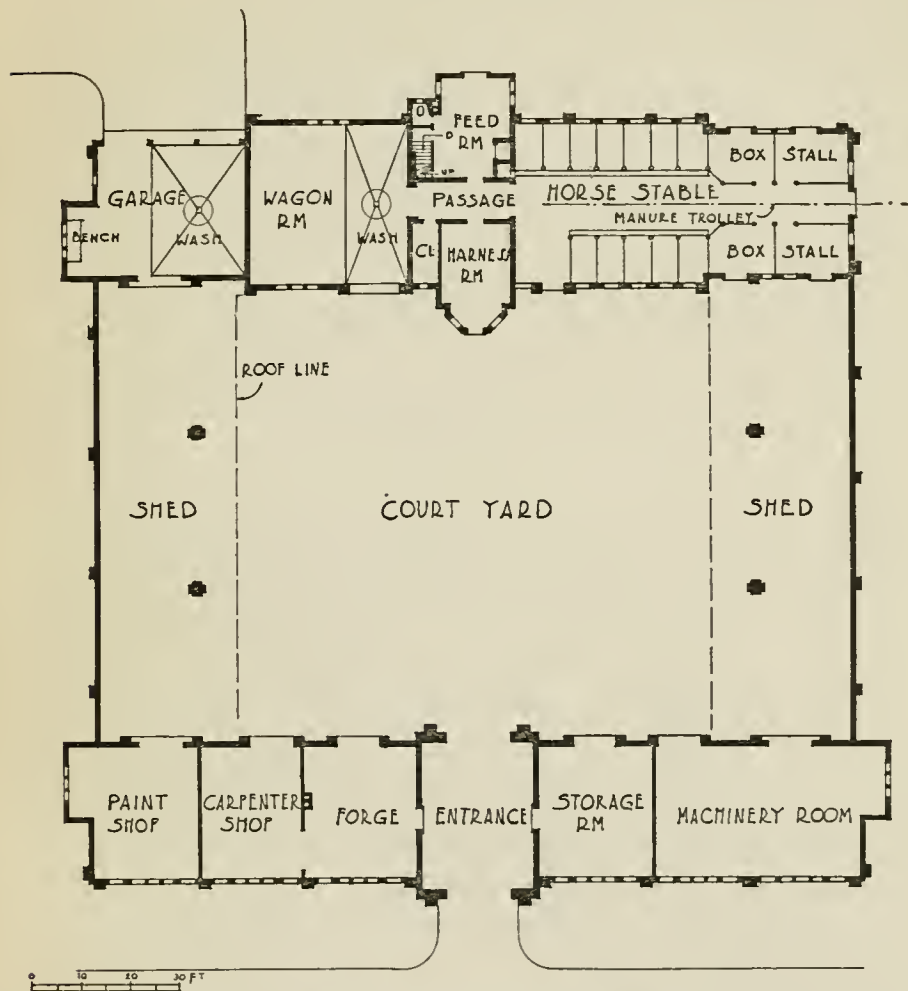
FIG. 55—PROPOSED FARM STABLE AT GREENWICH, CONN., FOR THE LATE HUGH J. CHISOLM, ESQ.
