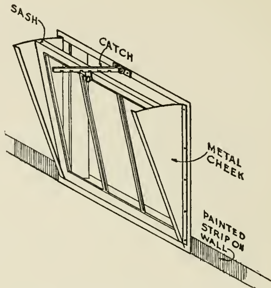
FIG. 35—WINDOW CHEEKS AND SASH FASTENER
