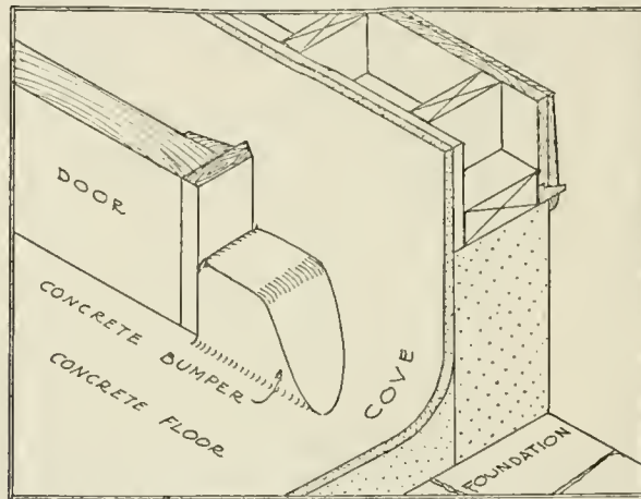
FIG. 21—ISOMETRIC VIEW OF CONCRETE BUMPER FOR DOORS
