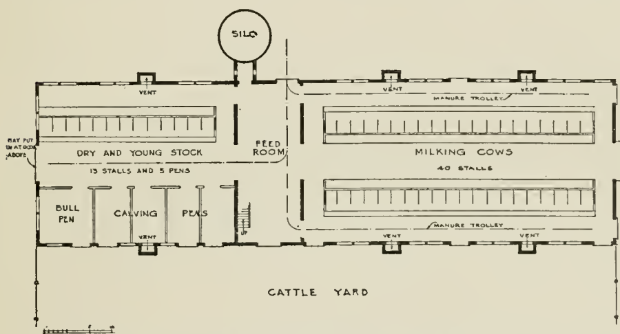
FIG. 1—PLAN SHOWING SIMPLEST POSSIBLE ARRANGEMENT OF COW BARN FOR YOUNG STOCK AND MILKING COWS—FEED BEING STORED OVER YOUNG STOCK
