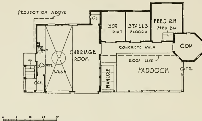
FIG. 54—PROPOSED SMALL STABLE AT HEWLET, L. I., FOR H. T. S. GREEN, ESQ.
