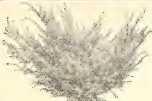
SPREADING YEW
