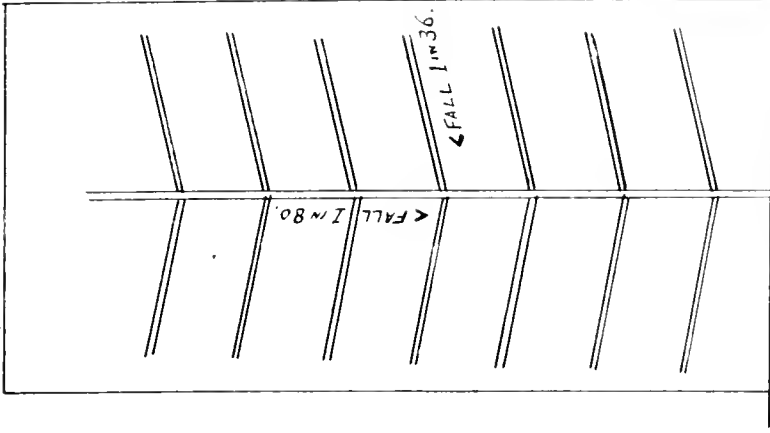
PLAN OF CONCRETE FLOORED STALL, SHOWING DRAINS AND DIRECTION IN WHICH THE GROOVES OF SINGLE GROOVE BRICKS SHOULD BE LAID.
