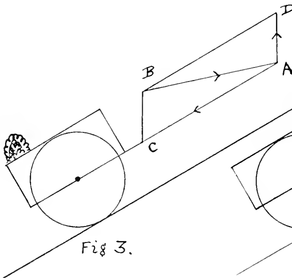
POSITION OF LOAD ON 2 WHEELED VEHICLE.
