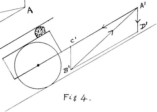
POSITION OF LOAD ON 2 WHEELED VEHICLE.
