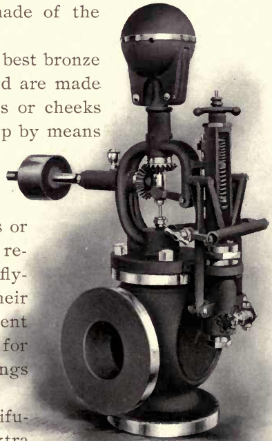
Combined Speed and Pressure Regulator
