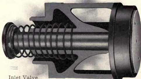
Inlet Valve on High Pressure Air Cylinder
