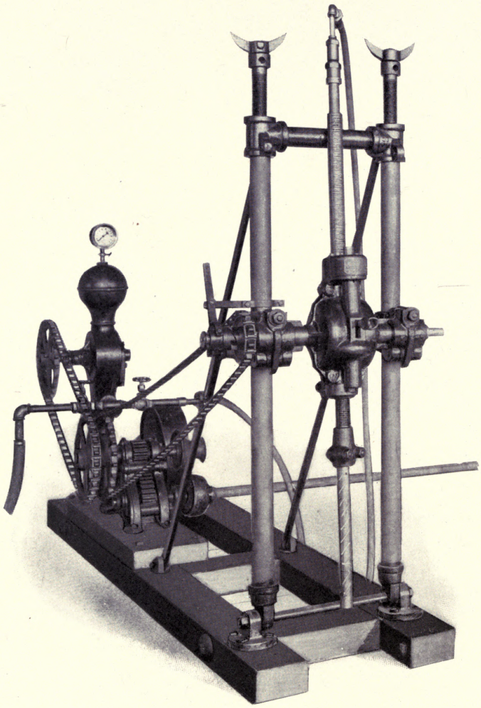
Bullock Diamond Prospecting Core Drill. Hand, horse or belt power, screw feed
