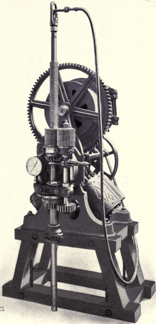
Bullock Diamond Prospecting Core Drill. Screw feed
