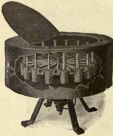
FIG. 17—ELECTRIC CENTRIFUGAL MACHINE OF LATEST DESIGN FOR USE IN BABCOCK TEST
