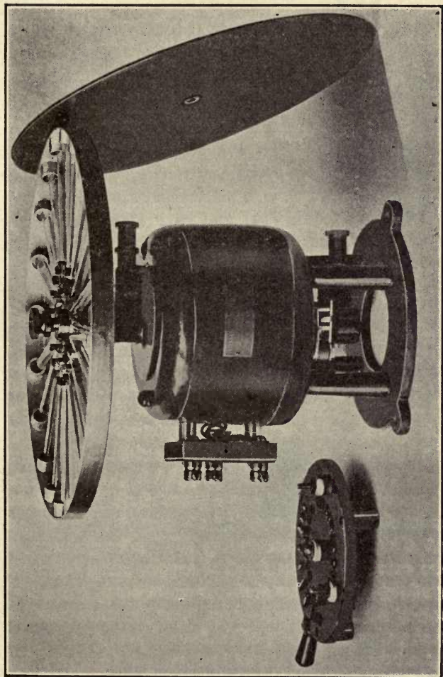
FIG. 44—INTERNATIONAL INSTRUMENT COMPANIES' ELECTRIC CENTRIFUGE FOR SEDIMENTATION WORK Capable of 3,000 revolutions per minute
