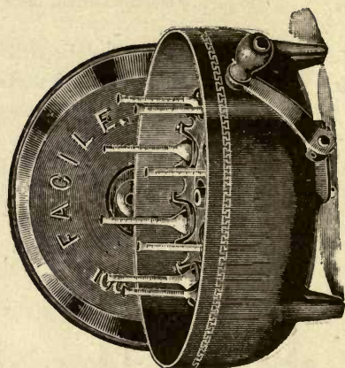
FIG. 15—HAND-TESTER
