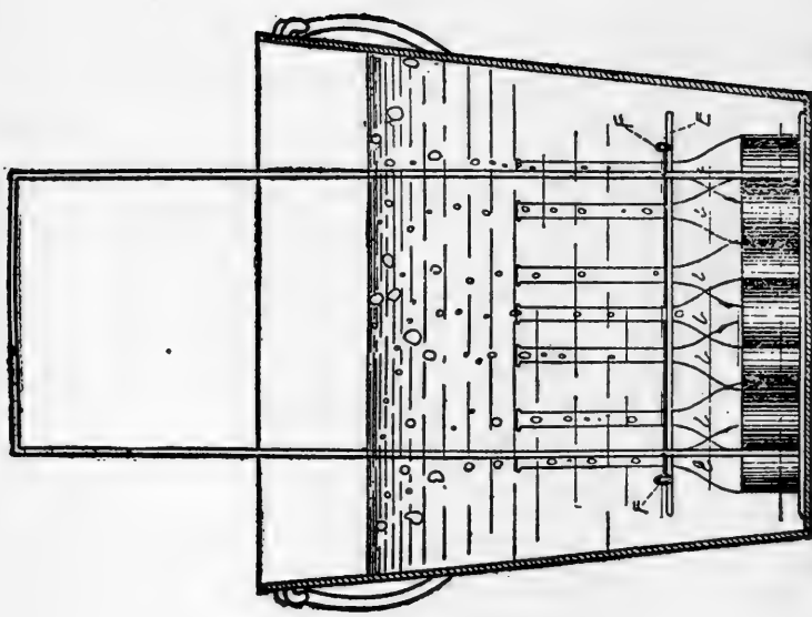
FIG. 25b—BOTTLE-HOLDER WITH BOTTLES IMMERSED IN PAIL OF HOT WATER
