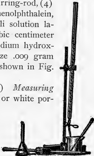
FIG. 37—MANN'S ACID TEST
