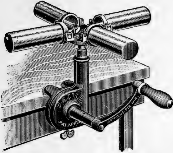
FIG. 16—SMALL HAND-TESTER
