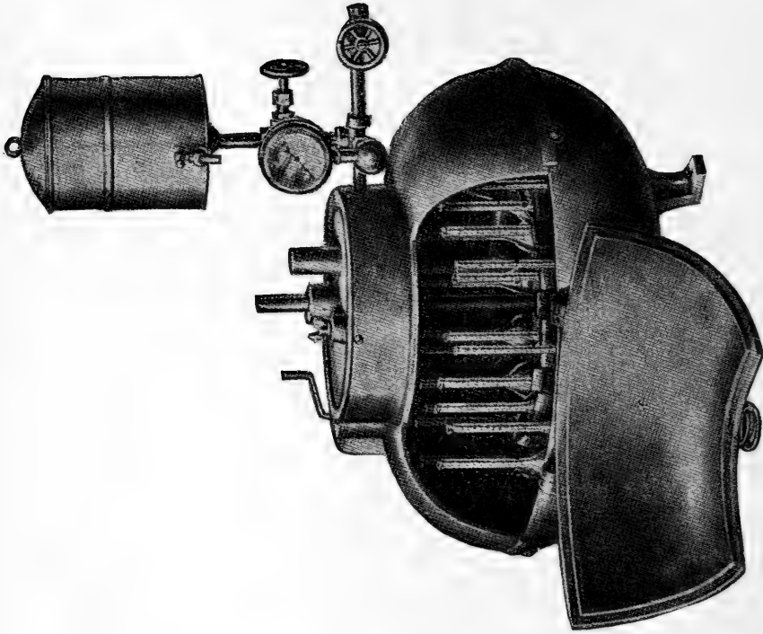
FIG. 14—STEAM-TURBINE TESTER
