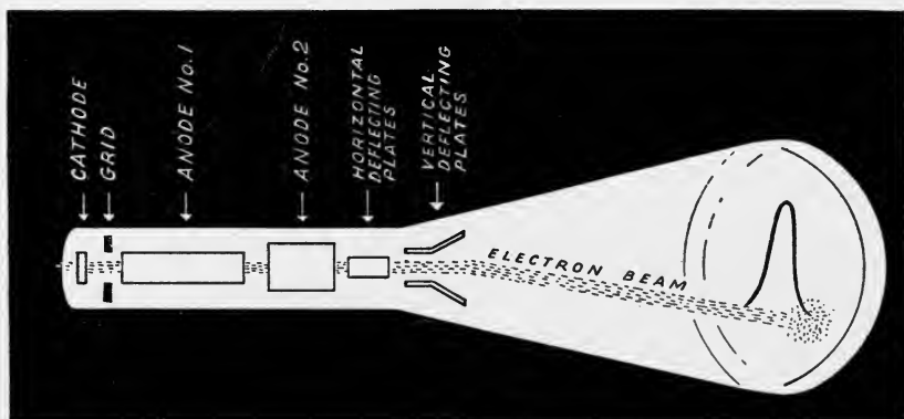
ELEMENTS IN CATHODE-RAY TUBE
