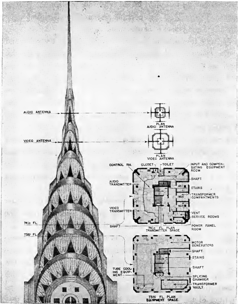
TELEVISION TRANSMITTER ROOM AND ANTENNA LAYOUT
