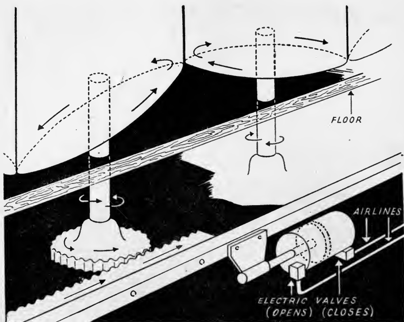
MECHANICAL DEVICE WHICH CONTROLS ACOUSTIVANES
