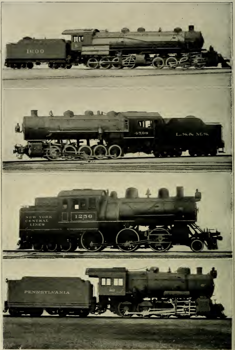
ONE OF THE GREAT MALLET PUSHING ENGINES OF THE DELAWARE & HUDSON COMPANY A TEN-WHEELED SWITCHING LOCOMOTIVE OF THE LAKE SHORE SUBURBAN PASSENGER LOCOMOTIVE OF THE NEW YORK CENTRAL CONSOLIDATION FREIGHT LOCOMOTIVE OF THE PENNSYLVANIA
