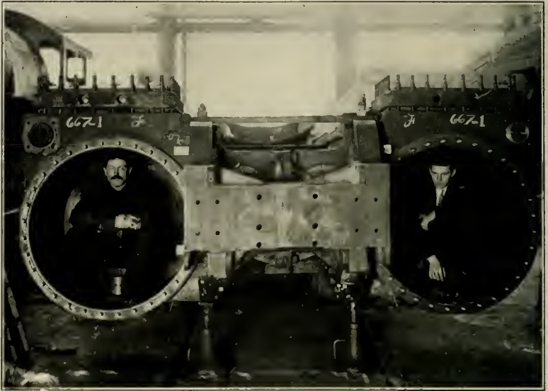
THE CYLINDERS OF THE DELAWARE & HUDSON MALLET
