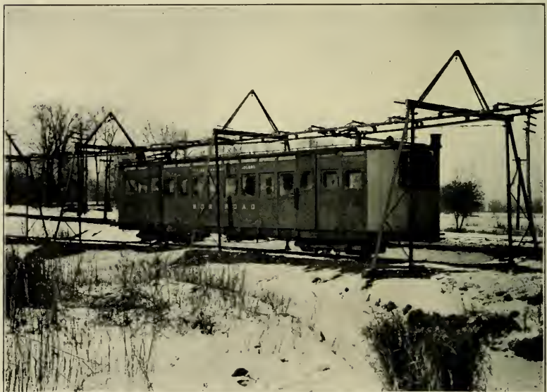
THE CIGAR-SHAPED CAR OF THE MONOROAD
