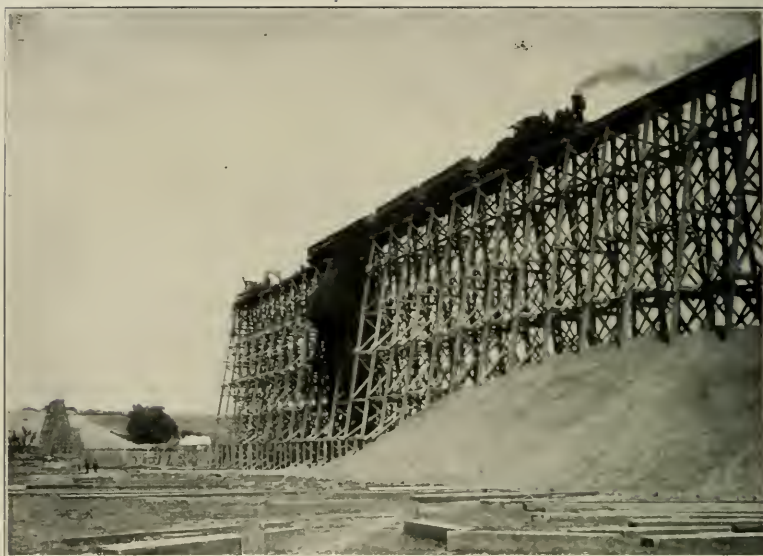
THE MAKING OF AN EMBANKMENT BY DUMP-TRAIN
