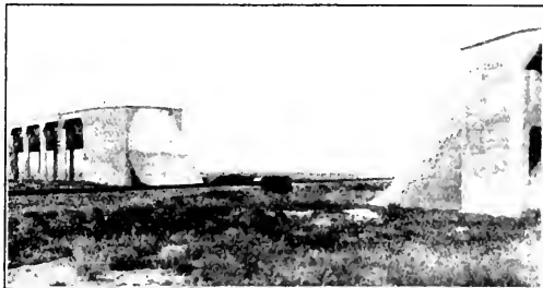
BROOKS AQUEDUCT SHOWING INVERTED SYPHON UNDER MAIN LINE OF THE C.P.R.
