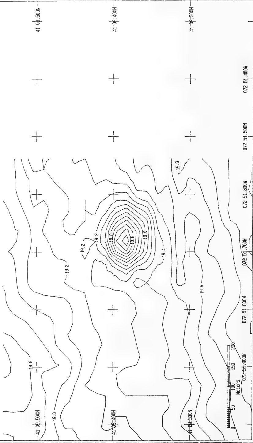
Figure 3-5. Bathymetric contour chart (m) of FVP, July 1986.
