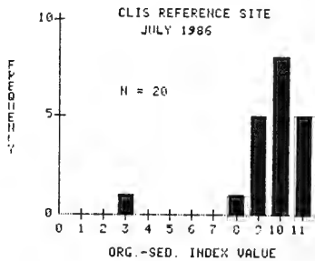
Figure 3-26. Frequency distributions of REMOTS ® Organism-Sediment Indices for all replicates at the FVP mound stations, FVP edge and ambient stations and the new CLIS reference station (n = sample size).
