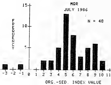
Figure 3-53. Frequency distributions of small-scale boundary roughness, mean apparent RPD depths and OSI values at the MQR disposal mound, July 1986.
