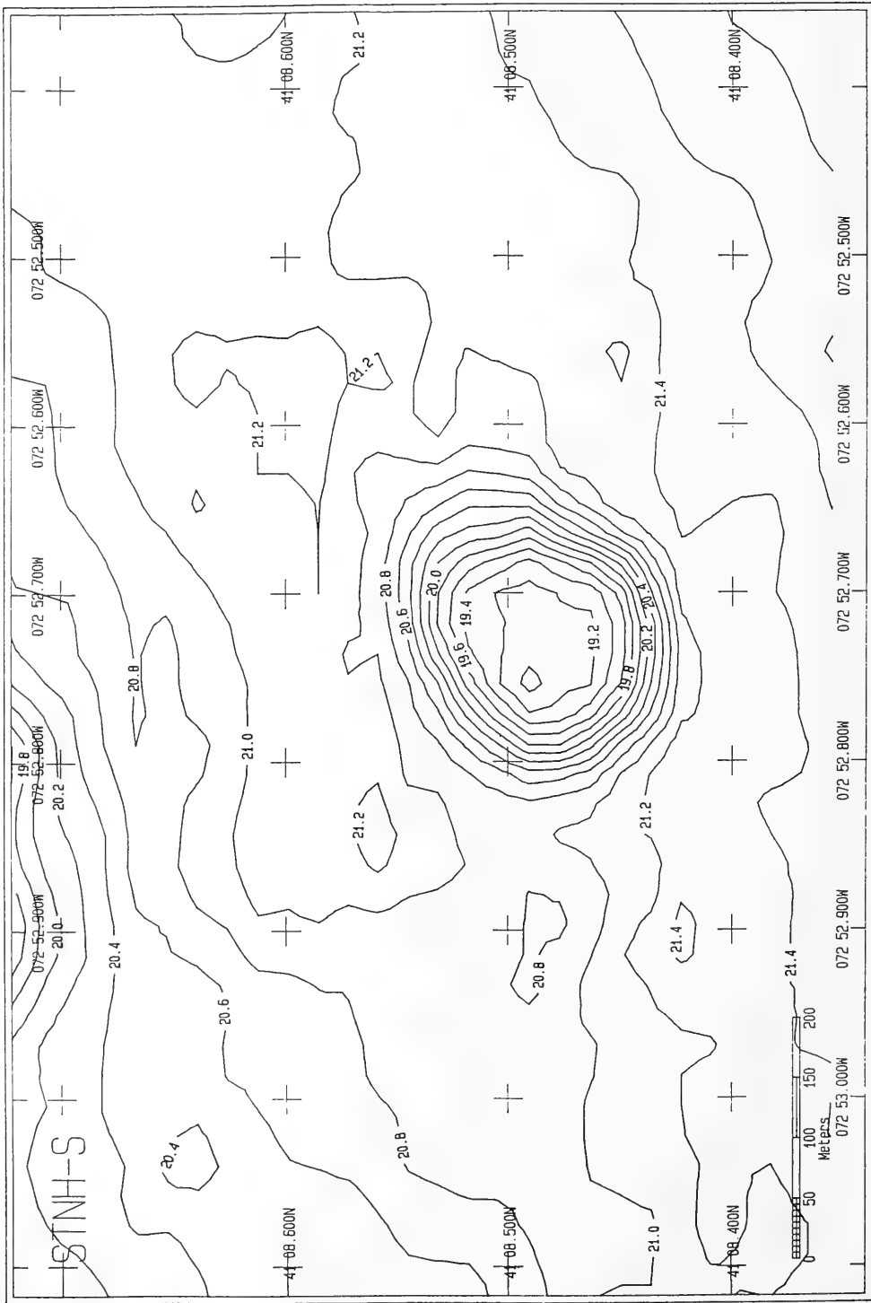
Figure 3-7. Bathymetric contour chart (m) of STNH-S, July 1986.
