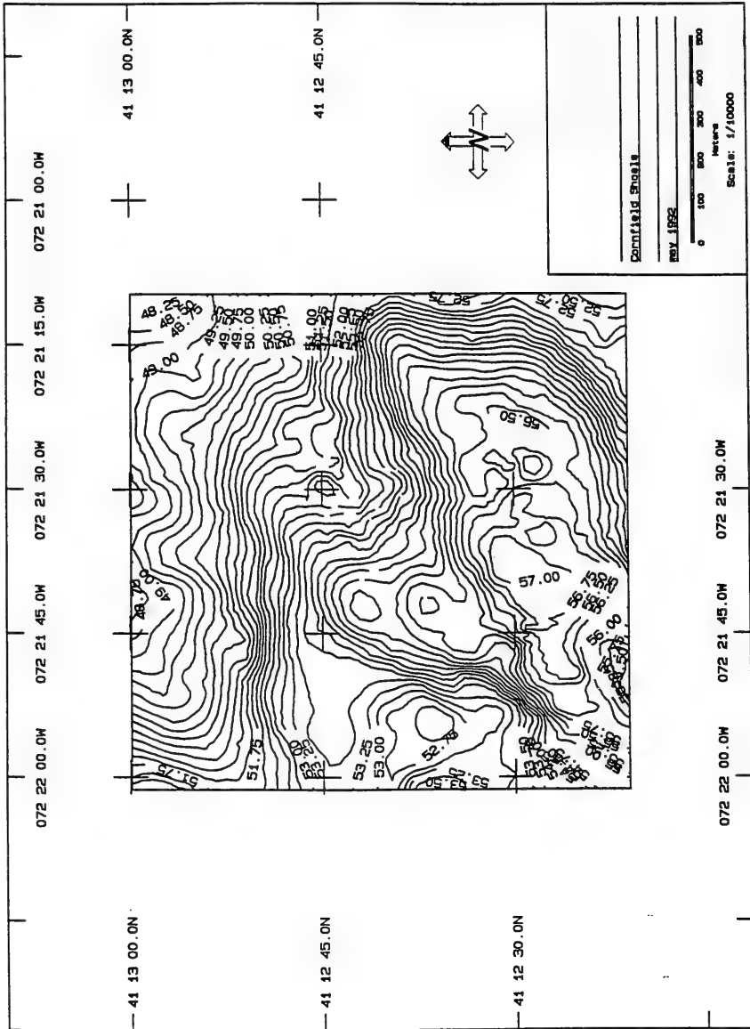
Figure 3-1. Bathymetric contour plot at the Cornfield Shoals Disposal Site, May 1992 (depth in meters)
