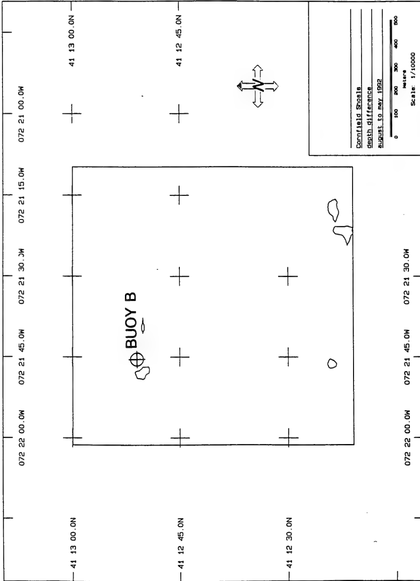
Figure 3-3. Negative depth difference contour plot between May 1992 and August 1992 (contours at 0.2 m)
