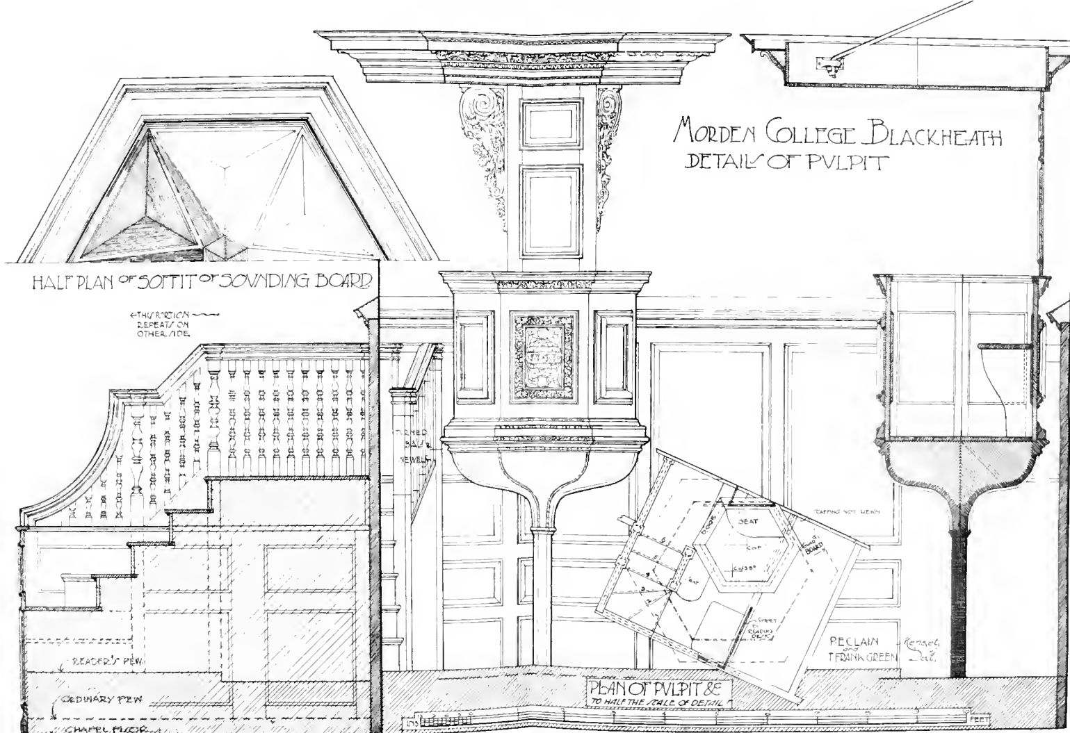
ELEVATION OF PULPIT
