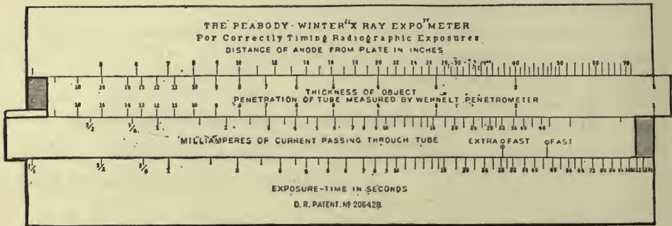
Fig. 26.—The X-ray Expometer. (By courtesy of the Kny-Scheerer Mfg. Co.)
