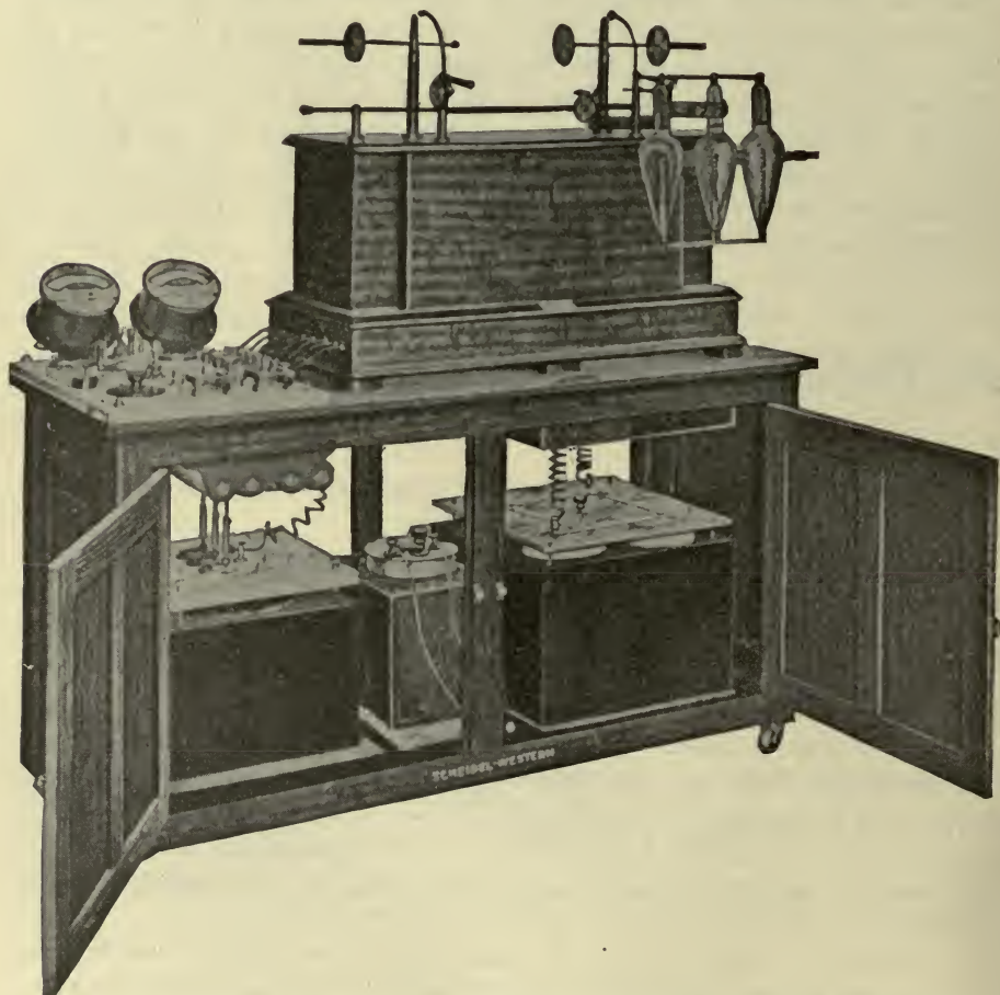
Fig. 5.—Induction Coil Apparatus. (By courtesy of the Scheidel-Western X-ray Coll Co.)
