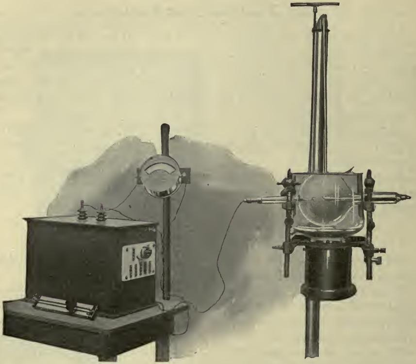
Fig. 23.—The Coolidge X-ray Tube, Operating in Connection with a Current Generating Unit for Heating the Cathode Spiral. The Amperemeter Indicates the Amount of Current Passing Through the Cathode Spiral of the Coolidge Tube. (By courtesy of the Kny-Scheerer Co.)
