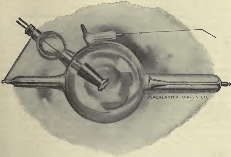
Fig. 12.—Water-cooled Tungsten Target Tube. (By courtesy of the Kelley-Koet Mfg. Co.)
