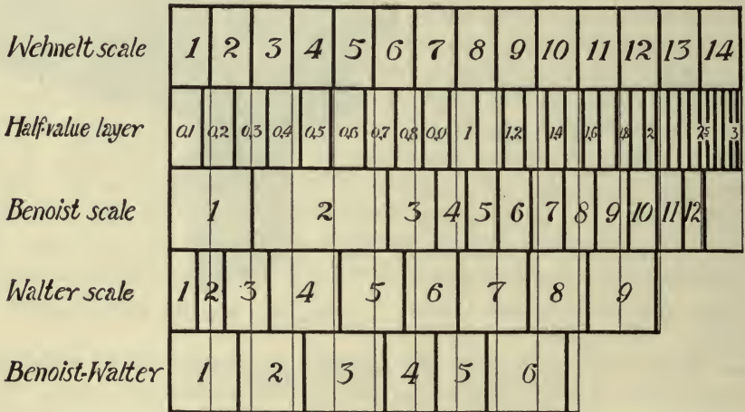
Fig. 15.—Comparative Scale for Penetrometers or Hardness Measurers.
