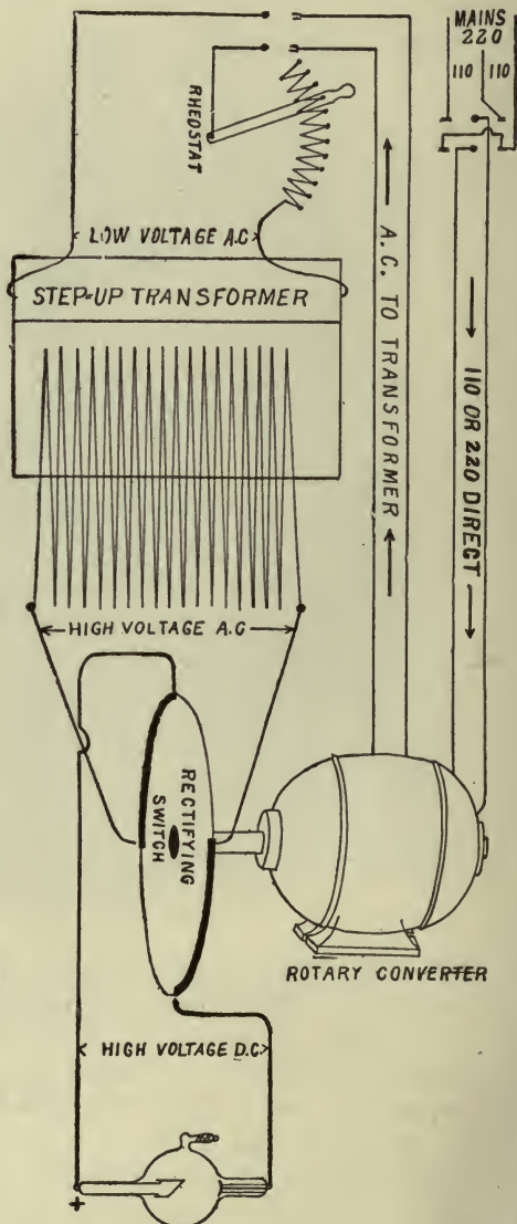
Fig. 10.—Wiring for Direct-current Generator (Interrupterless Transformer Apparatus). (By courtesy of the Kelley-Koett Mfg. Co.)
