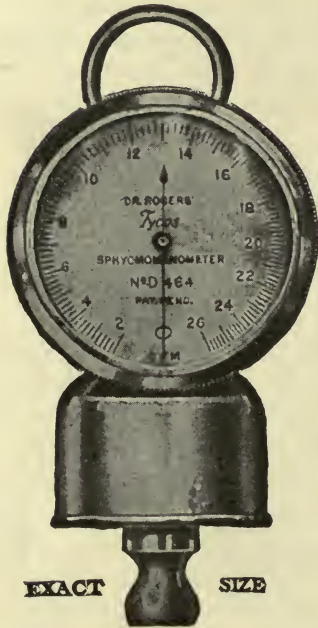
Fig. 227.—Tycos Sphygmomanometer. Method of Use: Pointer on Dial Operated by an Aneroid Chamber of Corrugated Metal—Not a Spring. (By courtesy of Taylor Instrument Co., Rochester, N. Y.)
