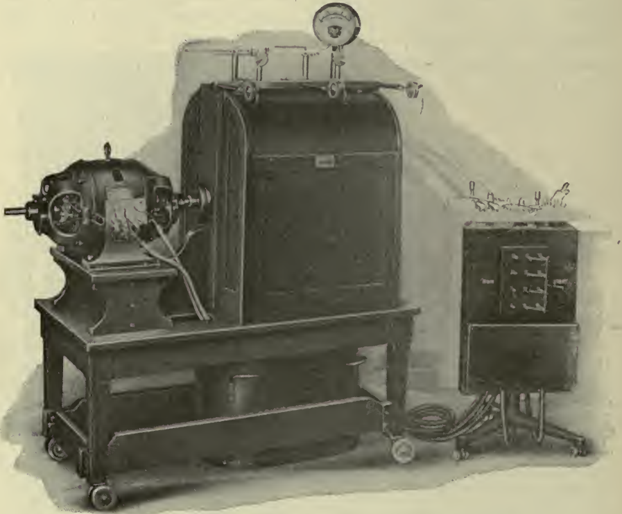
Fig. 7.—Interrupterless Apparatus. Alternating-current Machine. (By courtesy of the Snook-Röntgen Mfg. Co.).
