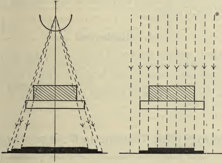
Fig. 20.—Ordinary and Orthogonal Projection. (After T. Brugsch and A. Schittenhelm.)
