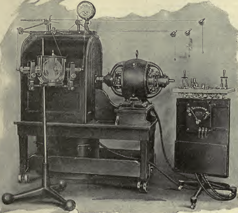
Fig. 8.—Interrupterless Apparatus. Direct-current Machine. (By courtesy of the Snook-Röntgen Mfg. Co.).
