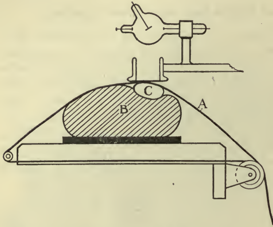
Fig. 25.—Compressor for Use in X-ray Work (Gurt).
