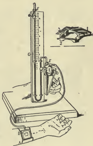
Fig. 237.—Apparatus of Hooker and Eyster for Determining the Venous Pressure. (J. H. H. Bull.)
