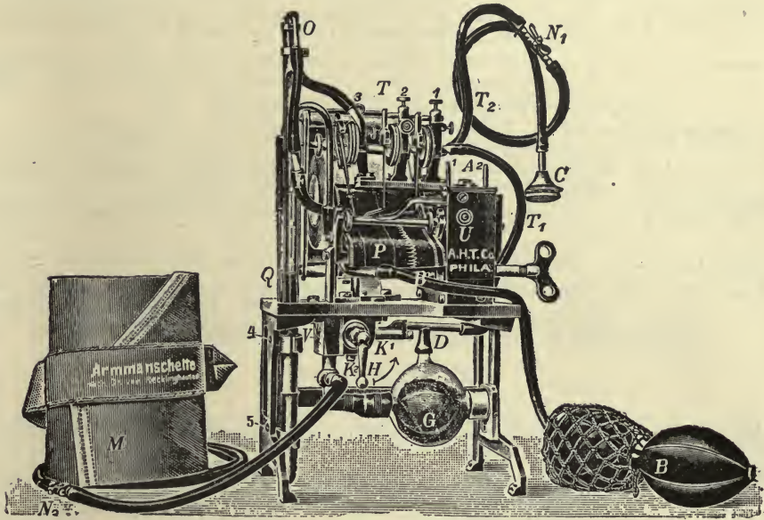
Fig. 229.—Uskoff's Blood-pressure Apparatus. (By courtesy of A. H. Thomas Co., Philadelphia.)
