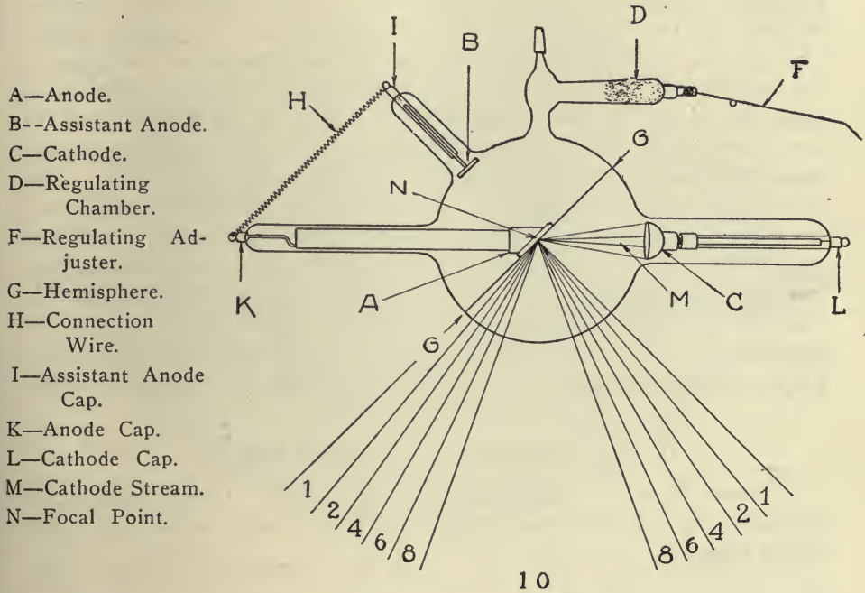
Fig. 11.—Diagram of a Röntgen Tube. (By courtesy of the Scheidel-Western X-ray Coil Co.)
