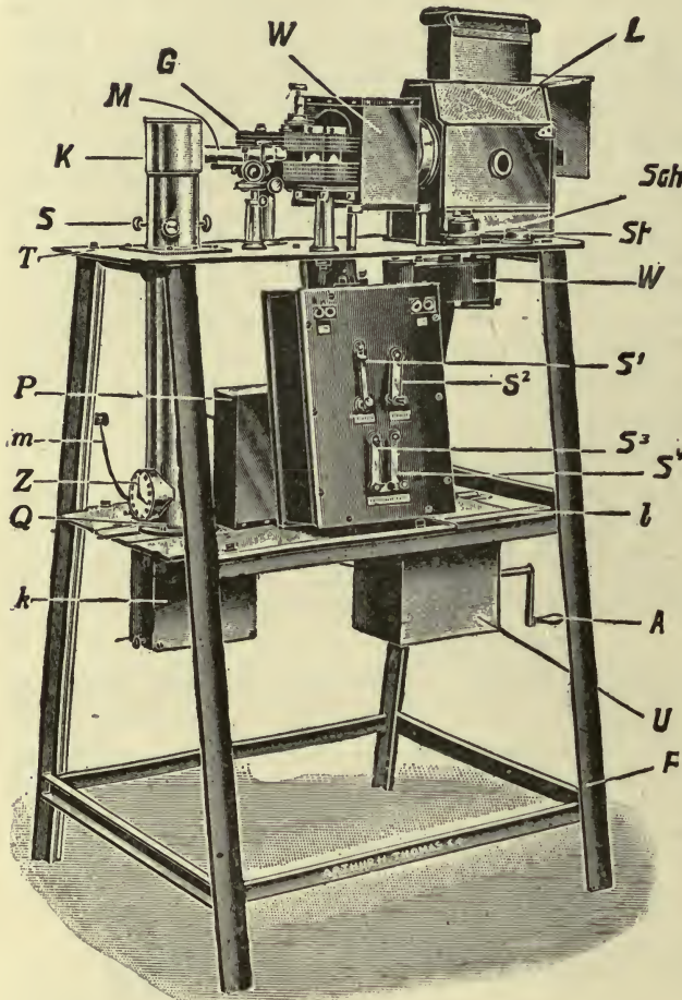
Fig. 213.—Small Electrocardiograph, Edelmann Model. New Simplified Electrocardiographic Outfit, Complete with L Arc Lamp, G Einthoven String Galvanometer with Permanent Magnet, M Projection Microscope, S 1 S 2 S 3 and S 4 Electric Devices for Determining the Sensibility of the Galvanometer and for Compensation of Skin Currents, Photographic Register, Electrodes and Stand. This Outfit is One of the Latest and Lowest Priced Complete Installations for the Taking of Electrocardiograms. (By courtesy of A. H. Thomas Co., Philadelphia.)
