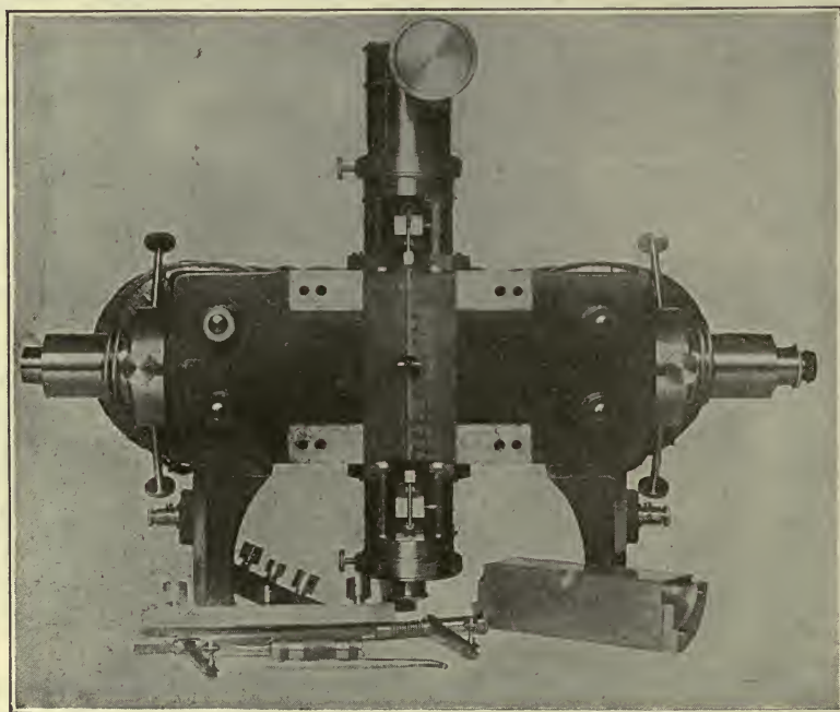
Fig. 215a.—The Williams-Hindle Electrocardiographic Outfit. (By courtesy of Dr. H. B. Williams.)
