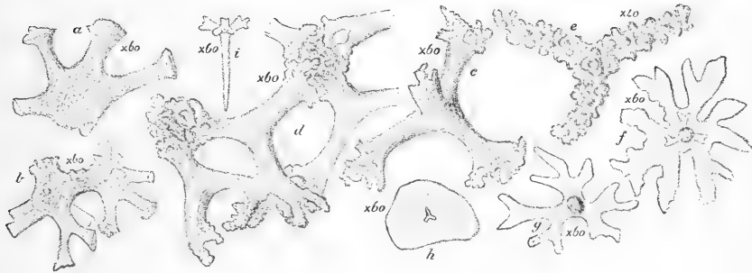
FIG. 5.—Various forms of fossil skeletal- and dermal-spicules of lithistid Sponges. ( a ) Elementary spicule of Anomocladina lithistid, Mastasia Neocomiensis , Hinde, from the Upper Greensand of Warminster, Wilts. ( b ) Paired or twin spicule of Anomocladina lithistid, Cylindrophyma milleporata , Goldf., sp. ( c ) Skeletal-spicule of Tetracladina lithistid, Callopegma acaule , Zitt. ( d ) Skeletal-spicules of Callopegma Schlanbachii , Zitt., showing their mode of union with each other. ( e ) Skeletal-spicule of tetracladine lithistid, Plinthosella squamosa , Zitt. ( f ) Dermal spicule of lithistid, showing the canals. ( g ) Another dermal spicule, showing the rudimentary shaft. ( h ) Dermal spicule of lithistid, in which no shaft is developed, but traces of the canals remain. ( i ) Dermal spicule of lithistid with furcate head-rays.
