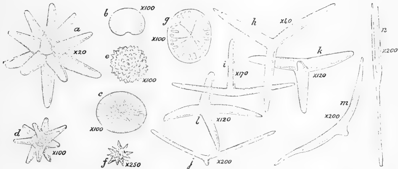
FIG. 7.—Different forms of fossil siliceous heteractinellid and multiaxial spicules and also spicules of fossil calcisponges. ( a ) Spicule of Asteractinella expansa , with twelve unequal rays proceeding from a common centre. ( b ) Kidney-shaped spicule of the dermal layer of Geodia . ( c ) Another dermal spicule of Geodia , showing its composition of apparent spicular rods. ( d ) Globostellate spicule in which there are traces of canals in each of the rays. ( e ) Globate spicule with a surface covered by minute spines. ( f ) Stellate spicule, probably of the dermal layer of a tetractinellid Sponge. ( g ) Thin elliptical disc with canals radiating from the centre; probably a dermal spicule, named Stelletites callodiscus , Carter. ( h ) A three-rayed equiangular and equiradiate spicule of fossil calcisponge. ( i ) A three-rayed sagittate spicule, with two equal, paired rays, and one ray, the basal, shorter than the other two. ( j, m ) Three-rayed spicules, with the basal ray only slightly developed; from the fibre of Tremacystia D'Orbigny , Hinde. ( k ) Four-rayed sagittate spicule with blunted apical ray, from the same Sponge. ( l ) A four-rayed spicule, showing the apical ray. ( n ) Three rayed (tuning-fork) spicule, in which the paired rays are nearly parallel with each other.
