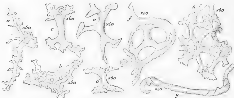
FIG. 4.—Various forms of fossil lithistid spicules belonging to the families of the Rhizomorina, Megamorina, and Anomocladina. ( a ) Branching, spinous, skeletal-spicule of rhizomorine lithistid, Selischothos Mantelli , Goldf. sp. ( b ) Two skeletal-spicules of the same Sponge, showing their mode of union with each other. ( c ) Skeletal-spicule of the rhizomorine Sponge, Cnemidiastrum Hoheneggeri , Zitt., from the Upper Jura of Cracow. ( d ) Skeletal-spicule of the rhizomorine Sponge Aulocopium , sp. from the Silurian of Gothland. ( e ) Skeletal-spicule of a megamorine Sponge, Doryderma , sp. from the Senonian strata of Coesfeld, Westphalia. ( f ) Skeletal-spicules of Doryderma , showing their mode of union with each other. ( g ) Skeletal-spicule of the megamorine Sponge, Carterella , sp. ( h ) Portion of the skeletal mesh of the Anomocladina Sponge, Astylospongia , sp. from the Silurian of Gothland, showing the spicules and their mode of union with each other.
