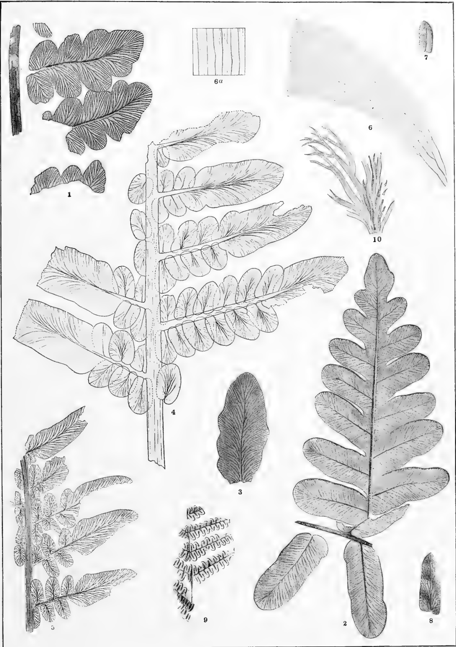
FERNS: CALLIPTERIDIUM, NEUROPTERIS, ALETHOPTERIS, AND LINOPTERIS.
