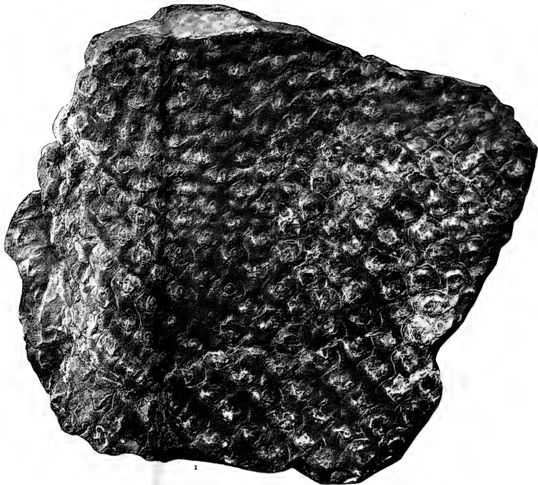
LYCOPODIALES: ONPHALOPHOIOS. (Fig. 1 is made to natural size.)
