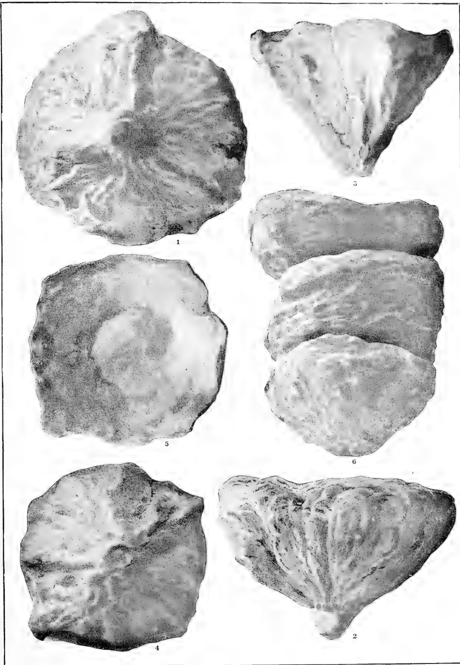
COMOSTICHUS, A SUPPOSED FOSSIL ALGA
