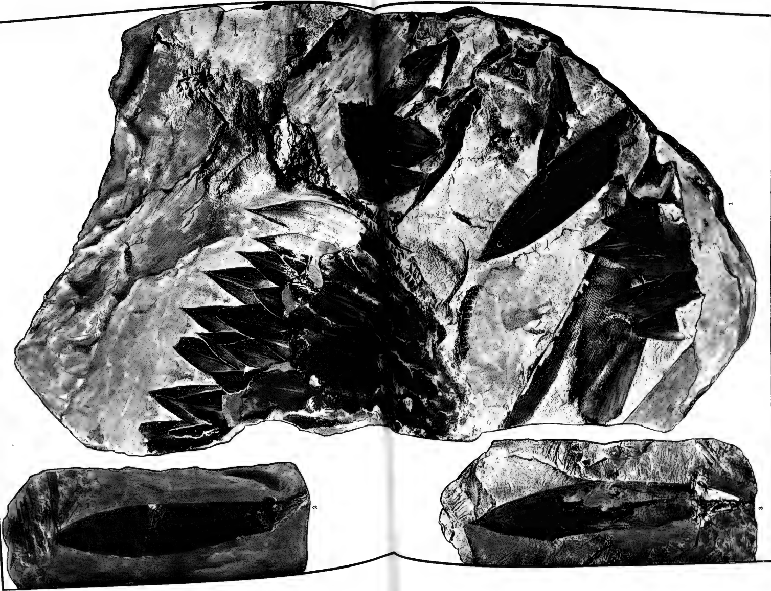
LYCOP. L. ALBES. LEAF AND STEM. PL. 1. LEAF AND STEM.
