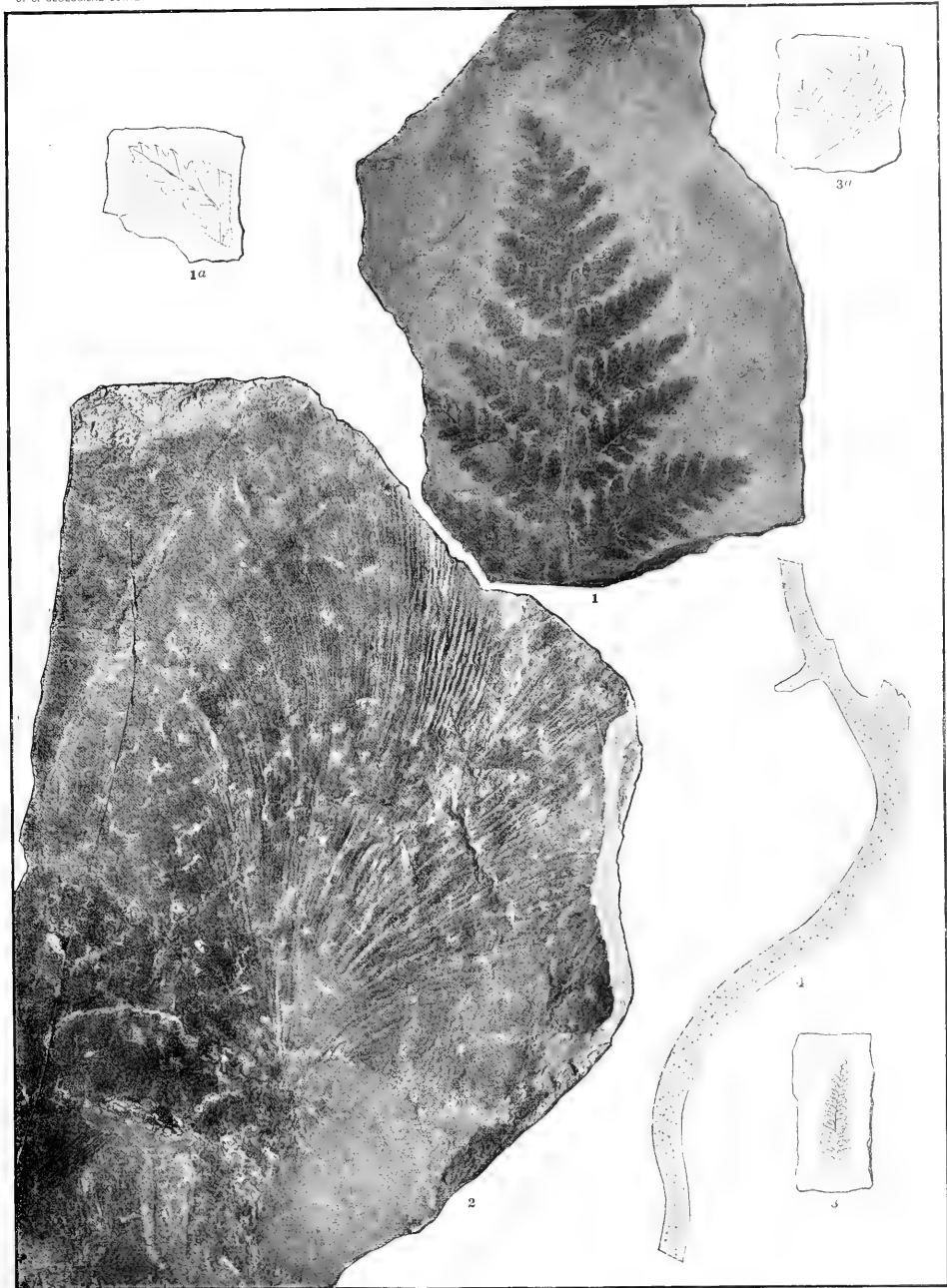
FERNS: NEUROPTERIS, SPHENOPTERIS, AND PECOPTERIS. ALGOID AXIS.
