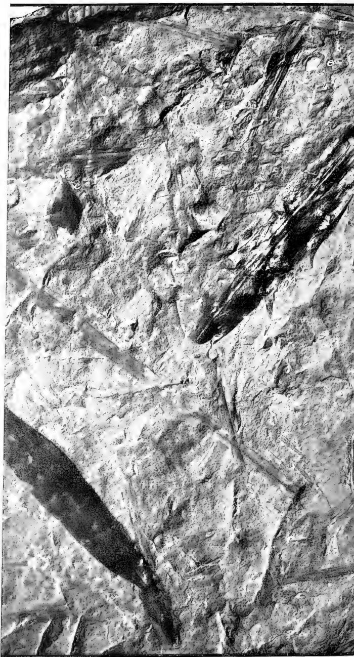
FERNS: CALLIPTERIDIUM AND LYCOPODIALES: LEPIDOPHLOIC CORDAITALES: CARDIOCARPON.
