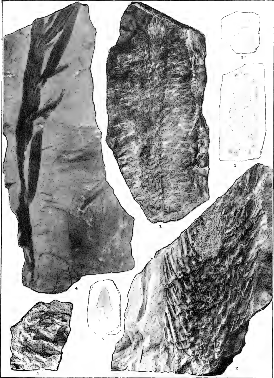
LYCOPODIALES: LEPIDOPHLOIOS, LEPIDOSTROBUS, TRILETES, AND TÆNIOPHYLLUM
