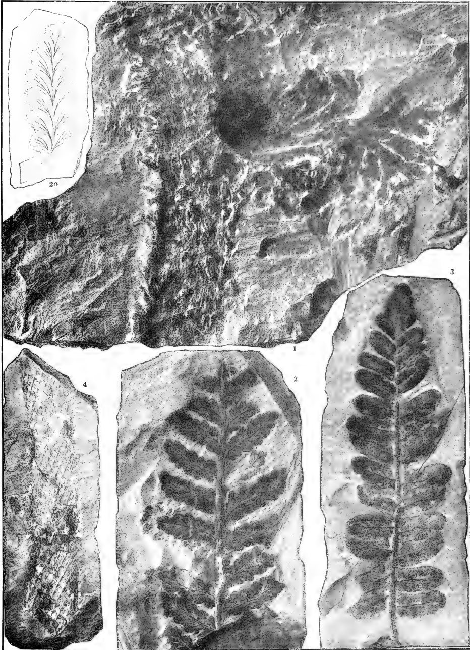
FERNS: SPHENOPTERIS, NEUROPTERIS, AND APHLEBIA. LYCOPODIALES: LEPIDODENDRON.
