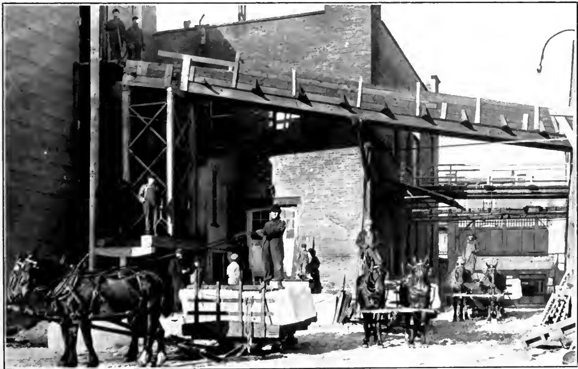
ICE HOUSE OF THE MONTREAL DAIRY CO., LIMITED. Capacity 7,000 tons.
