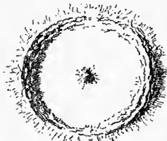
PETAVIUS. 78 Miles Diam r
