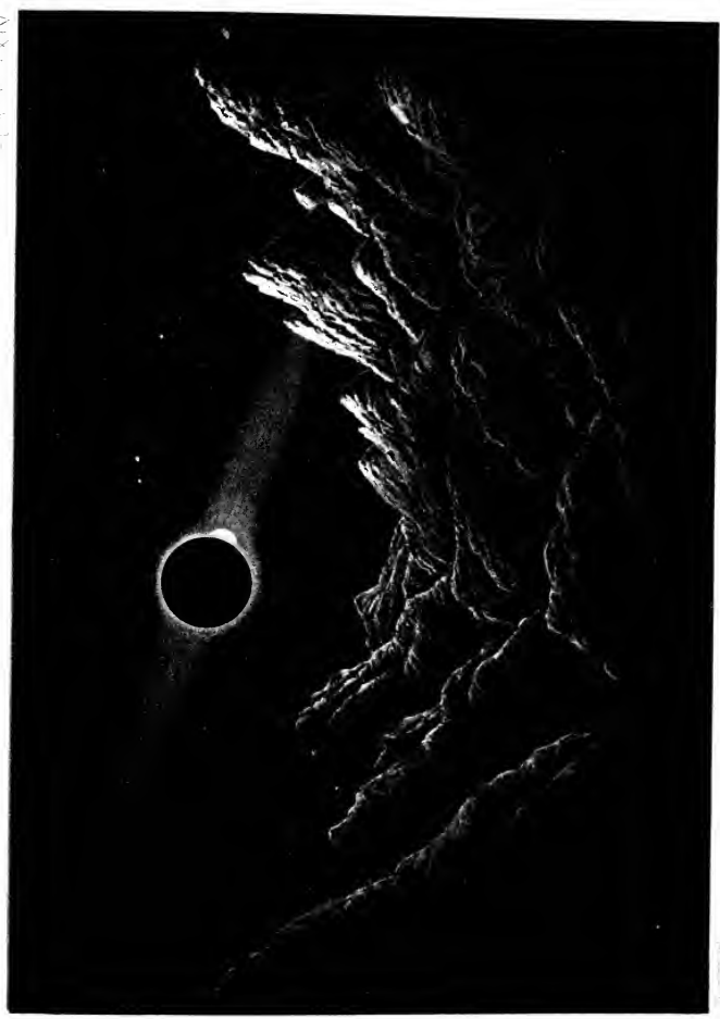
ASPECT OF AN ECLIPSE OF THE SUN BY THE EARTH AS IT WOULD APPEAR AS SEEN FROM THE MOON.
