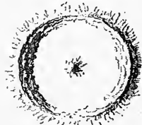
ALPHONS 70 Miles Diam r
