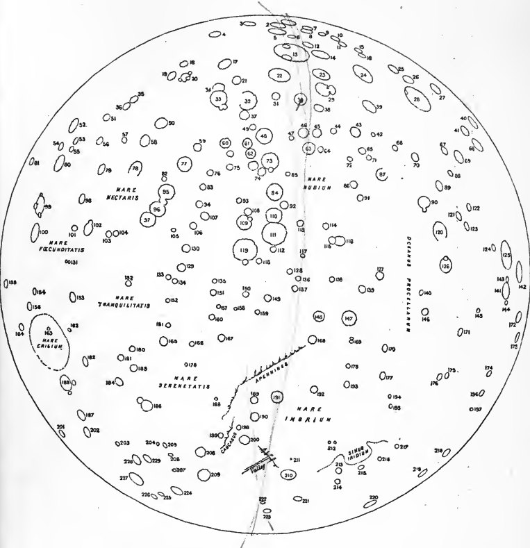
SKELETON MAP OF THE MOON. TO ACCOMPANY PICTURE MAP (Plate V.).
