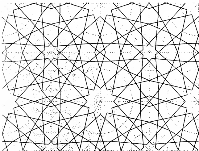
105 SQUARE PLAN. DIVIDE AS INDICATED AND INSCRIBE A STARRED DODECAGON, THE EXTENDED LINES OF WHICH FORM AN OUTER STAR ALSO OF TWELVE POINTS; THE STARRED OCTAGON IS CONSTITUTED BY POINTS PROLONGED FROM THE DODECAGON.
