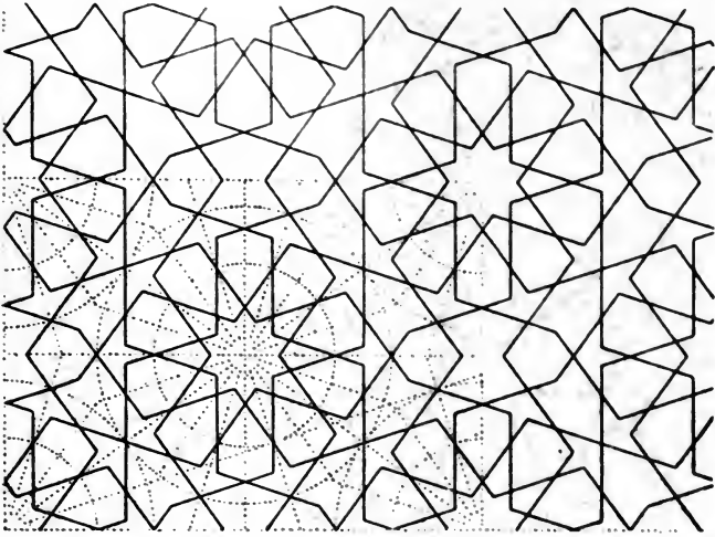
175 SUB-DIVIDE AS INDICATED. DESCRIBE CIRCUMFERENCES EQUAL AND TANGENT, AND TAKE THE DIAGONALS OF FOUR IN FOUR DIVISIONS. LASTLY, THE ROSETTES ARE EFFECTED.
