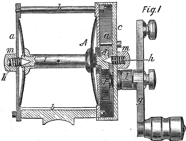
“Imbric” Compensating Reel. (Abbey & Imbric.)
