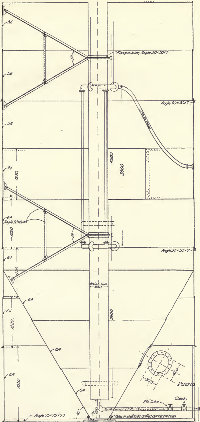
FIG. 5. LOWER PART OF BROWN AGITATING VAT
