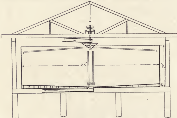
Fig. 66. ARRANGEMENT OF VAT AND DISTRIBUTERS
