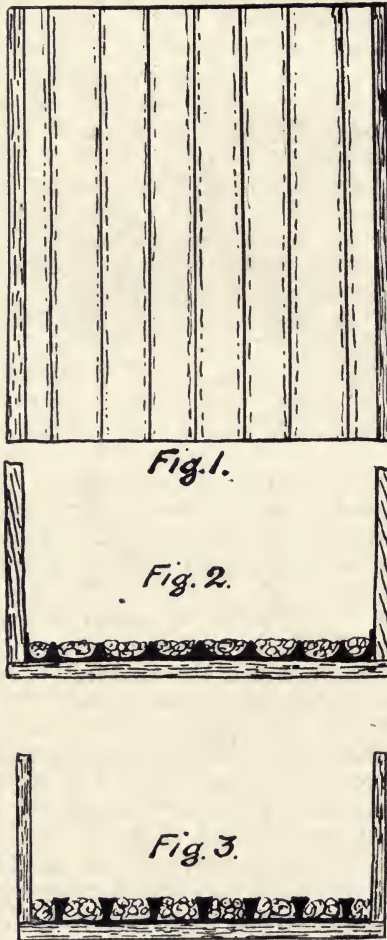
FIG. 30. LINING FOR BOTTOM OF LAUNDERS
