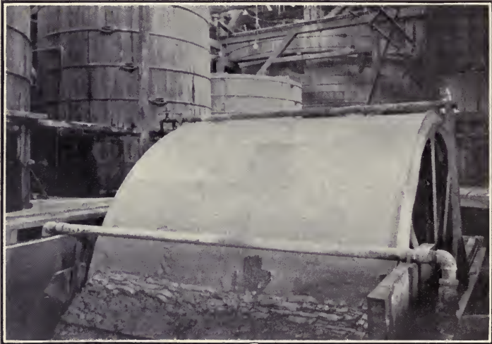
One of Four Oliver Continuous Filters at North Star Mines, Grass Valley, Cal.
