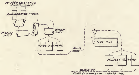
Fig. 33. TREATMENT OF SULPHIDE ORE
