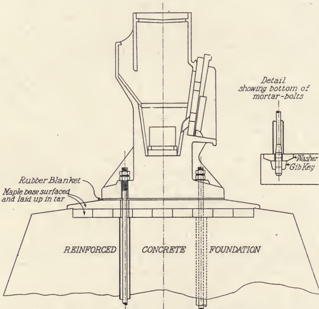
Fig. 51. MORTAR FOUNDATIONS
