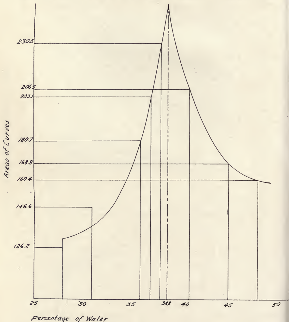
Fig. 85. TEST ON BEST DILUTION OF TUBE-MILL FEED
