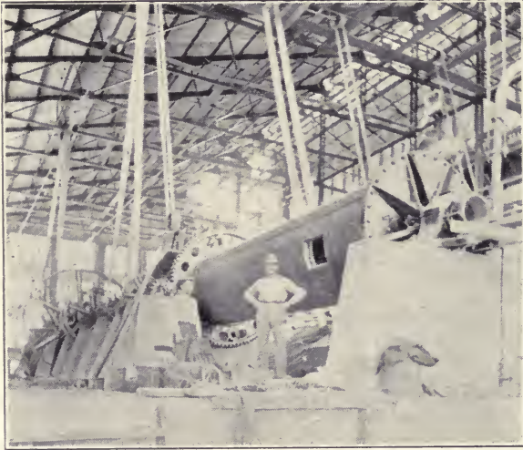
Fig. 49. TUBE-MILL IN THE NEW PLANT OF THE GOLDFIELD CONSOLIDATED
