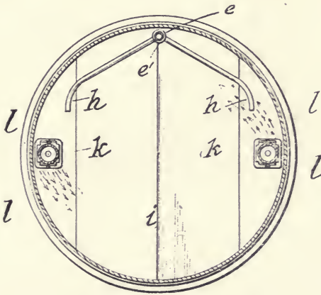
Fig. 88. PARRAL TANK
