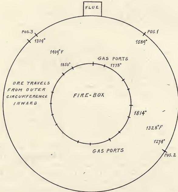
Fig. 18. CHART SHOWING POSITIONS OF READINGS ON THE HOLT-HOFF FURNACE.
