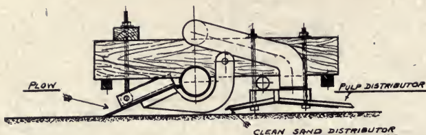
Fig. 46. DETAIL OF CARRIAGE
