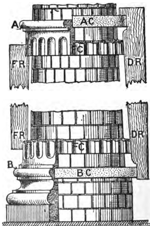
FORMING FLUTED COLUMNS—COLLAR METHOD.
