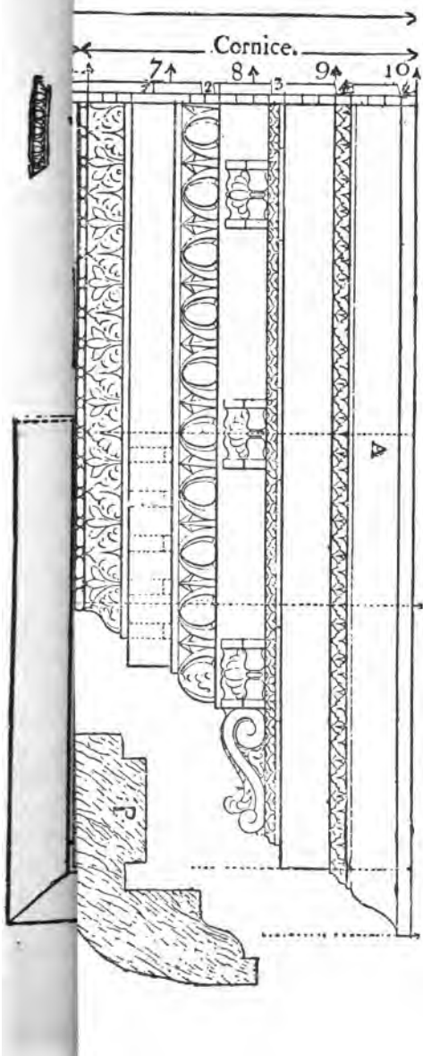
ELEVATION OF CORINTHIAN ENTABLATURE AND PLAN OF CORNICE AT EXTERNAL ANGLE. PLATE 1
