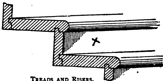
TREADS AND RISERS. NO. 25.
