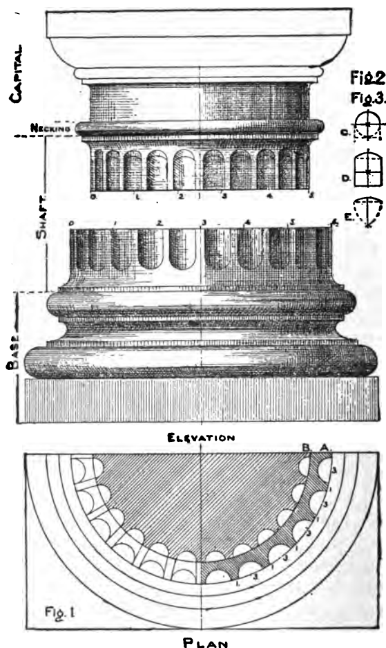
—DIMINISHED FLUTED COLUMNS.
