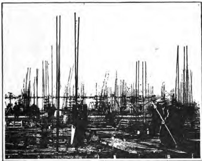
Fig. 7.—Ramsome System of Erecting Columns.
