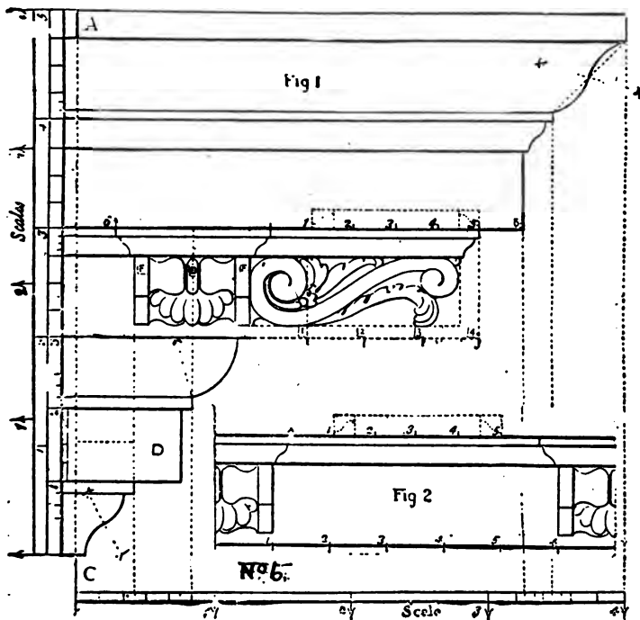
CORINTHIAN CORNICE.
