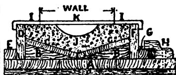
FIG. 1.—SECTION OF MOULD FOR CASTING SILLS.
