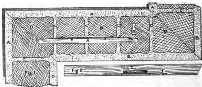
-FIG. 1. FLOATING COVES. FIG. 2. LEVELLING RULE.
