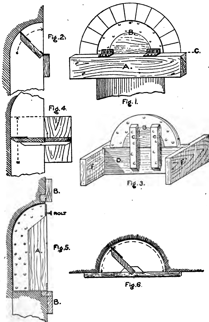
FORMING NICHES WITH RUNNING MOULDS. NO. 23.
