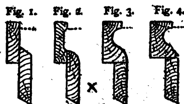
SECTIONS OF NOSING MOULDS WITH RISER BOARDS. NO. 20.
