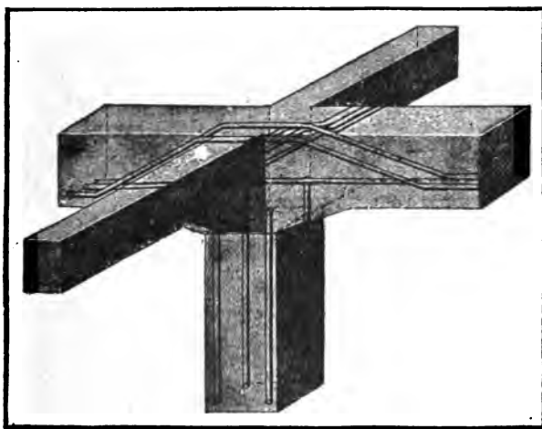
Fig. 3.—A Reinforced Concrete Pier for Railway Traffic.
