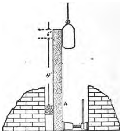
First method of testing posts by impact.
