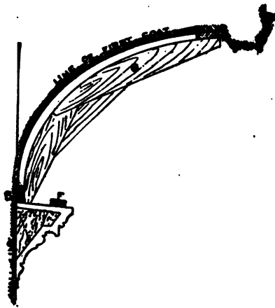
SECTION OF COVE SHOWING PRESSED SCREED PROCESS.
