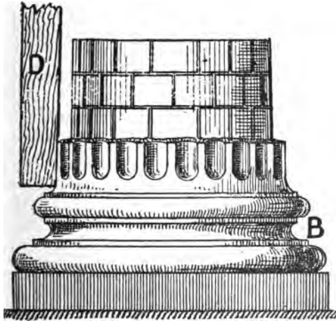
-FLOATED FLUTED COLUMNS, RIM METHOD.
