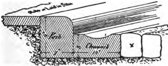
SECTIONS OF CONCRETE KERB, CHANNEL, AND PAVING.
