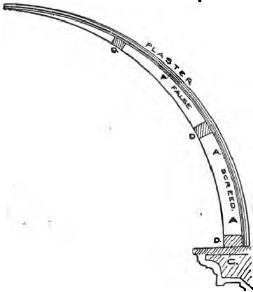
SECTION DOUBLE DIMINISHED MOULDINGS— FALSE SCREED METHOD.
