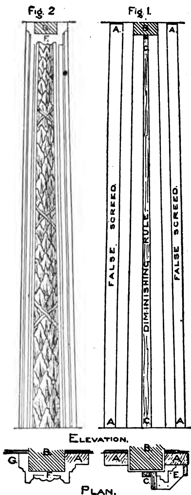
ELEVATION DOUBLE DIMINISHED MOULDINGS—FALSE SCREED METHOD.
