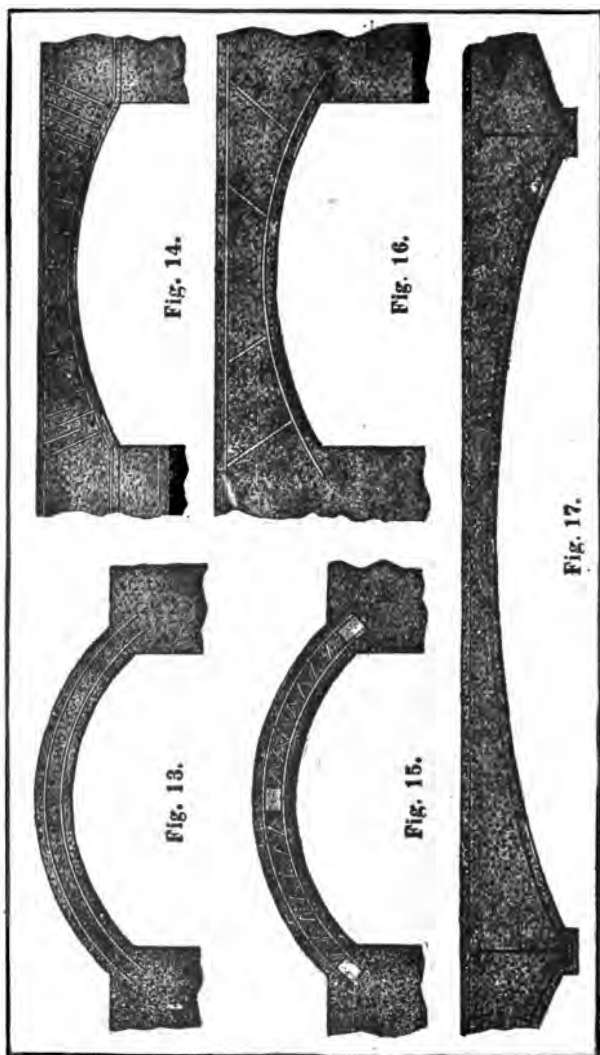
Types of Reinforced Concrete Arches.
