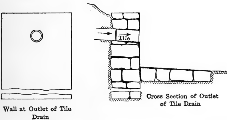
Detail of outlet of a tile drain.
