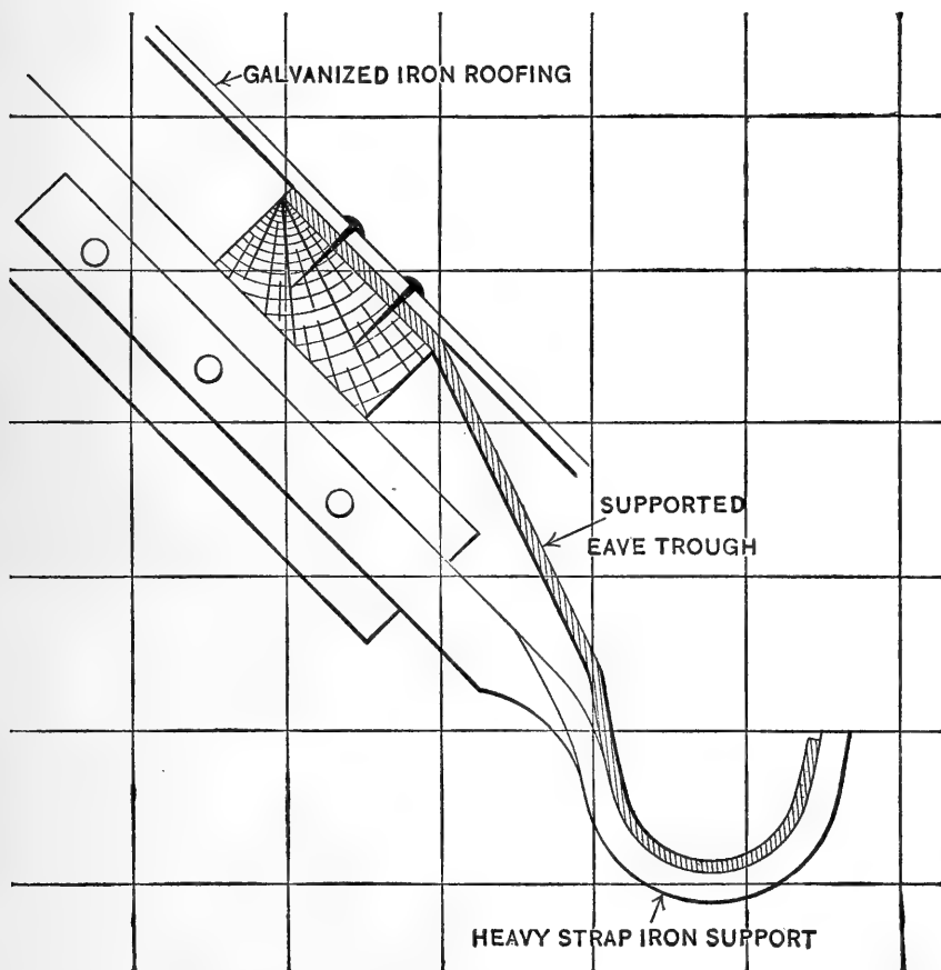
A firmly supported eave-trough.
