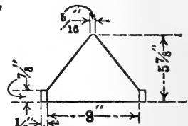
Wire Screen High Ridge Frame of White Pine
