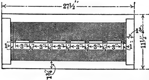
Mosquito trap, with details of construction.
