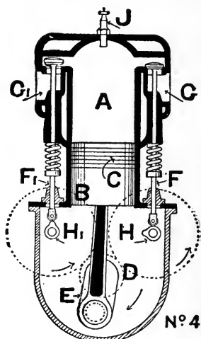
EXHAUST STROKE.
