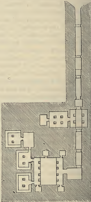
Plan of the tomb of Ramesses I.
