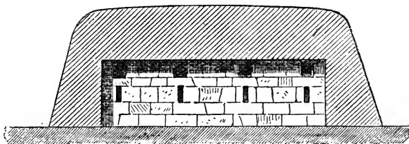
5. Transverse section of the chamber of a Maṣṭaba.
