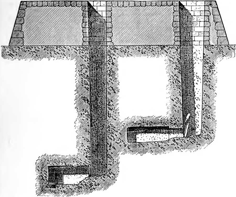
8. Maṣṭaba at Gizeh with double pit.
