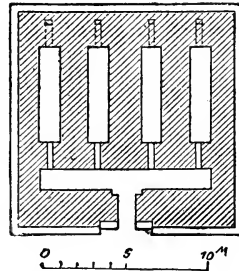
3. Plan of a Maštaba with four serdābs.
