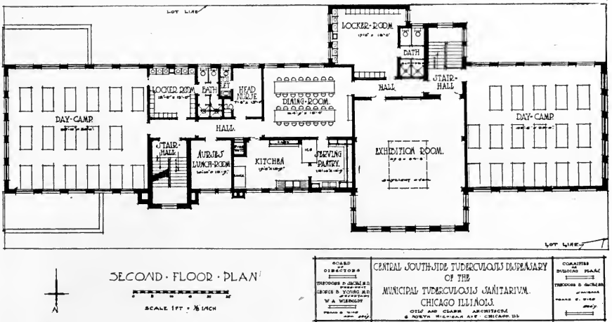
Second Floor
