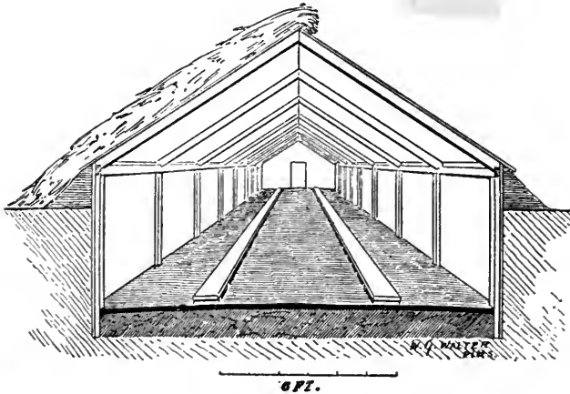
FIGURE 500.—Mushroom Houses, Flat Beds.
